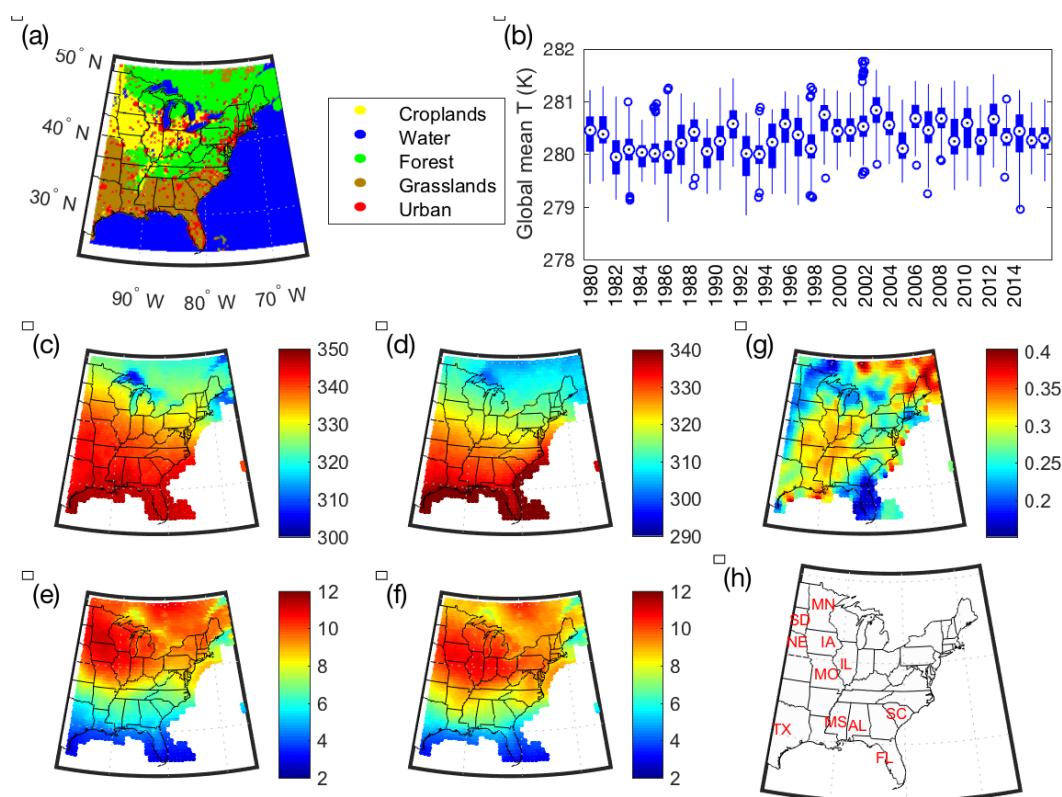
Figure 1. (a) The study domain used herein and five consolidated land use land-cover (LULC) classes as represented at a resolution of 0.05 \times 0.05^\circ from the MODIS land cover data set for 2014 (MCD12C). (b) A boxplot of daily global mean JJA temperature values (K) (1980-2014) as computed from the MERRA-2 output. (c) Mean summertime (JJA) maximum- \theta_e and (d) minimum- \theta_e (K) as computed from hourly T and q at 2-m and surface pressure ( P ) in each MERRA-2 grid cell. Standard deviation of daily (e) maximum- \theta_e and (f) minimum- \theta_e (K). (g) Mean soil moisture estimates from MERRA-2 used as a predictor in the ANN and computed as follows: the daily mean value for total profile soil moisture content (PRMC) for each grid cell is averaged over a spatial area of 3 \times 3 grid cells centered on the grid cell of interest, and used to compute a 90-day running JJA mean soil moisture ( \text{m}^3\text{m}^{-3} ). Panel (h) shows the location of states that are explicitly referred to herein.
