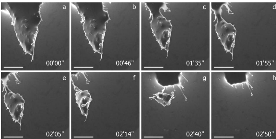
Figure 5. The dynamical in-situ micrographs of a large size (~100 μm), brine-covered piece of ice formation and breakaway during slow evaporation of water from the FF. Imaged with the ESEM AQUASEM II; beam energy 20 keV, ionisation detector, water vapour pressure 348 Pa, sample holder temperature -5.2 °C, sample to aperture distance 2mm. Scale bars: 100μm. A video of this case is attached (S2).
