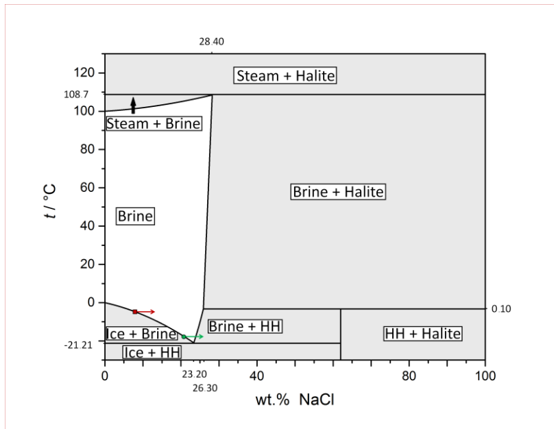
Figure 4: The phase diagram for a water/NaCl system. Indicated (red and green arrows) are our experimental conditions at about -5 °C and -17 °C. HH stands for hydrohalite (NaCl.2H 2 O). Based on equations from (Brady, 2009).
