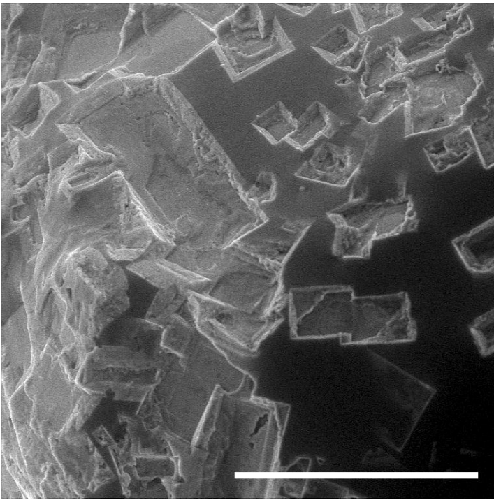
5 Figure 8: The NaCl crystals are clearly seen on the top of the surface brine layer of the FF. During the gradual process of evaporation, the individual ice crystals were moving on the brine surface at first, eventually growing into a large cluster of crystals. The ESEM AQUASEM II, ionisation detector, air pressure 510 Pa, sample holder temperature -15.0 °C, sample to aperture distance 2mm. Scale bars: 200µm. A video visualizing the formation of these crystals is attached (S5).
