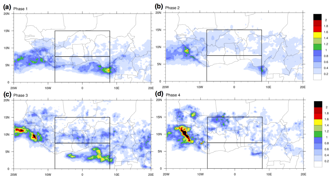
5 Figure 6: Horizontal distribution of mean precipitation during the four Phases of the DACCIWA campaign. Plots are based on TRMM precipitation and given in \text{mm h}^{-1} . (a) Phase 1 (01–21 June 2016), (b) Phase 2 (22 June–20 July 2016), (c) Phase 3 (21–26 July 2016) and (d) Phase 4 (27–31 July 2016). The black boxes mark the areas used to compute the north–south precipitation difference shown in Fig. 5a. Corresponding anomalies are shown in Fig. S1.
