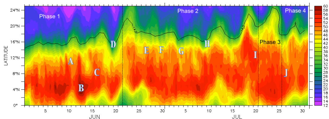
10 Figure 7: Evolution of TCWV (shading in mm) and the ITD (black line, identified from the 14^{\circ}\text{C} isoline of 2-m dewpoint) during June–July 2016 based on ECMWF operational analysis. The four Phases of the DACCIWA campaign and significant synoptic-scale features A–J are marked at the approximate time and latitude of crossing the DACCIWA focus region as in Fig. 5b.
