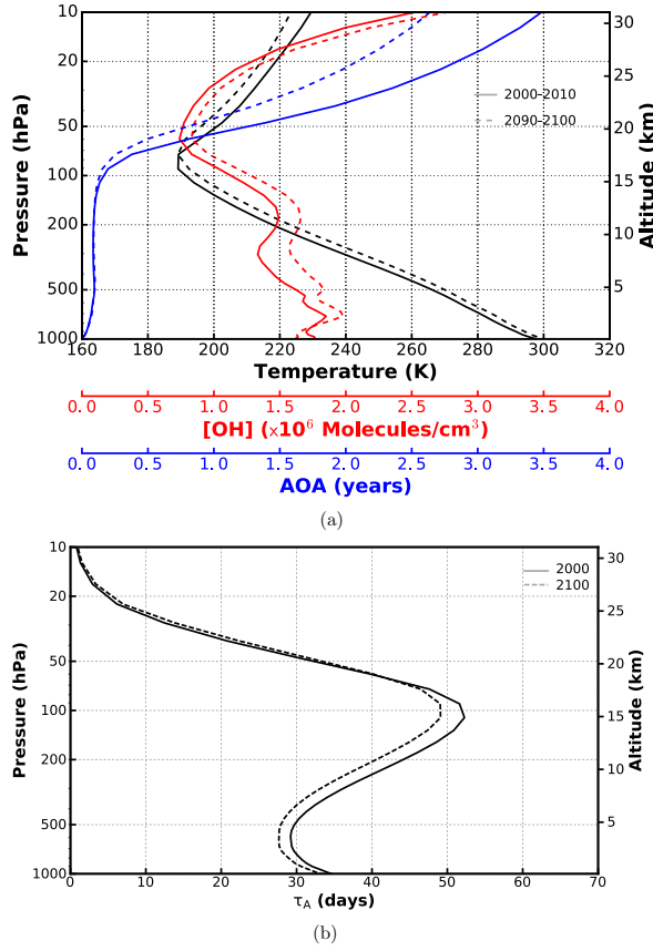
Figure 6. Tropical average profiles from ESCiMo RC2-base-05 simulation of changing variables in Eq. (3) for present day (solid lines) and future (dashed lines). (a) Temperature, OH concentration, and age of air; (b) Lifetime of CHBr 3 .
