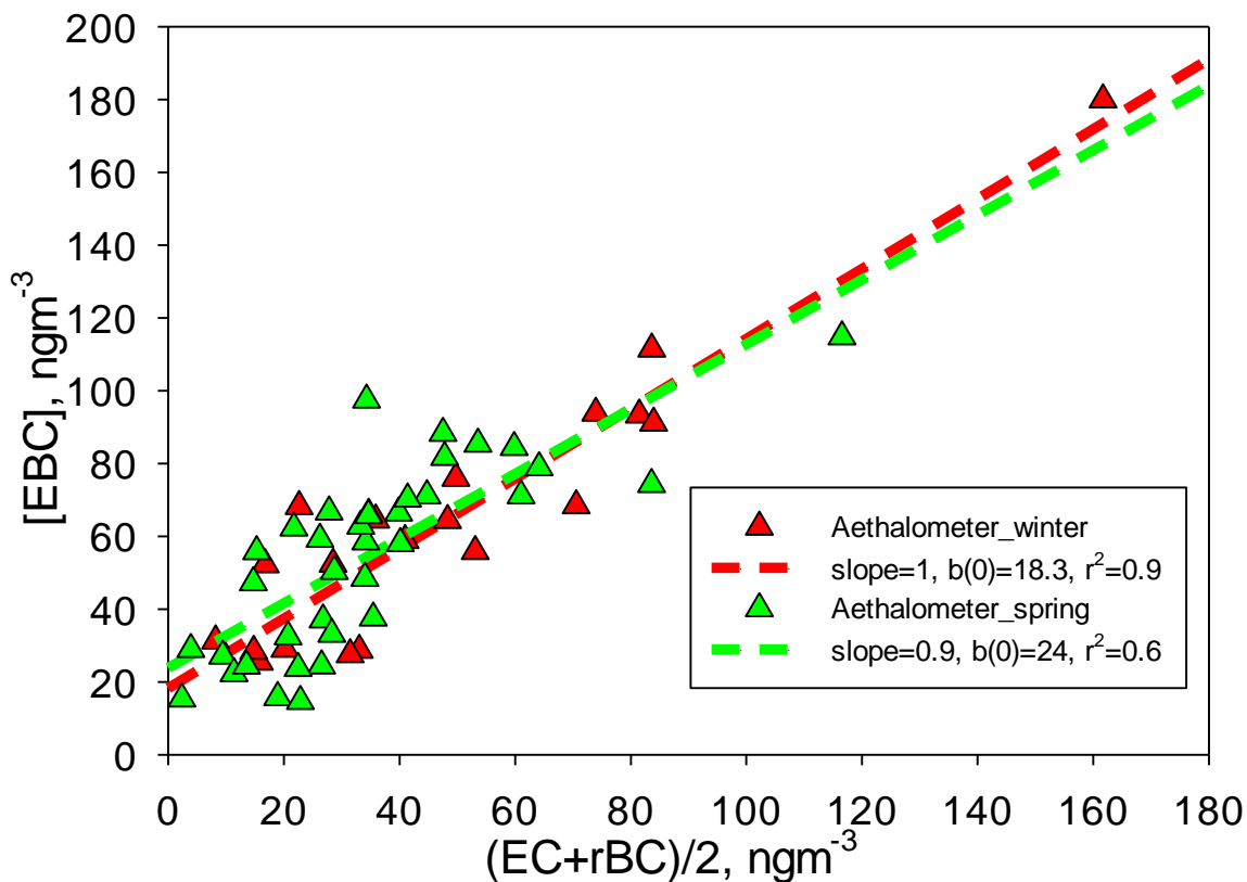
Supplement_Fig.: Improved agreements were obtained between the best estimated black carbon mass and masses obtained by optical technique such as Aethalometer ( green and red triangles are for data during spring and winter ). EBC Aethalometer and rBC data were averaged to EC sampling times.
