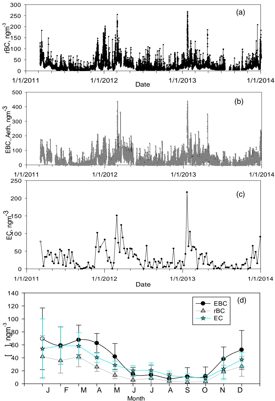
Figure 5: The temporal variation of BC at Alert, NU from March 2011 to December 2013: (a) hourly refractory BC, (b) hourly equivalent BC from the Aethalometer @ 880 nm, (c) weekly EC concentrations, and (d) monthly averaged mass of each technique and standard deviation.
