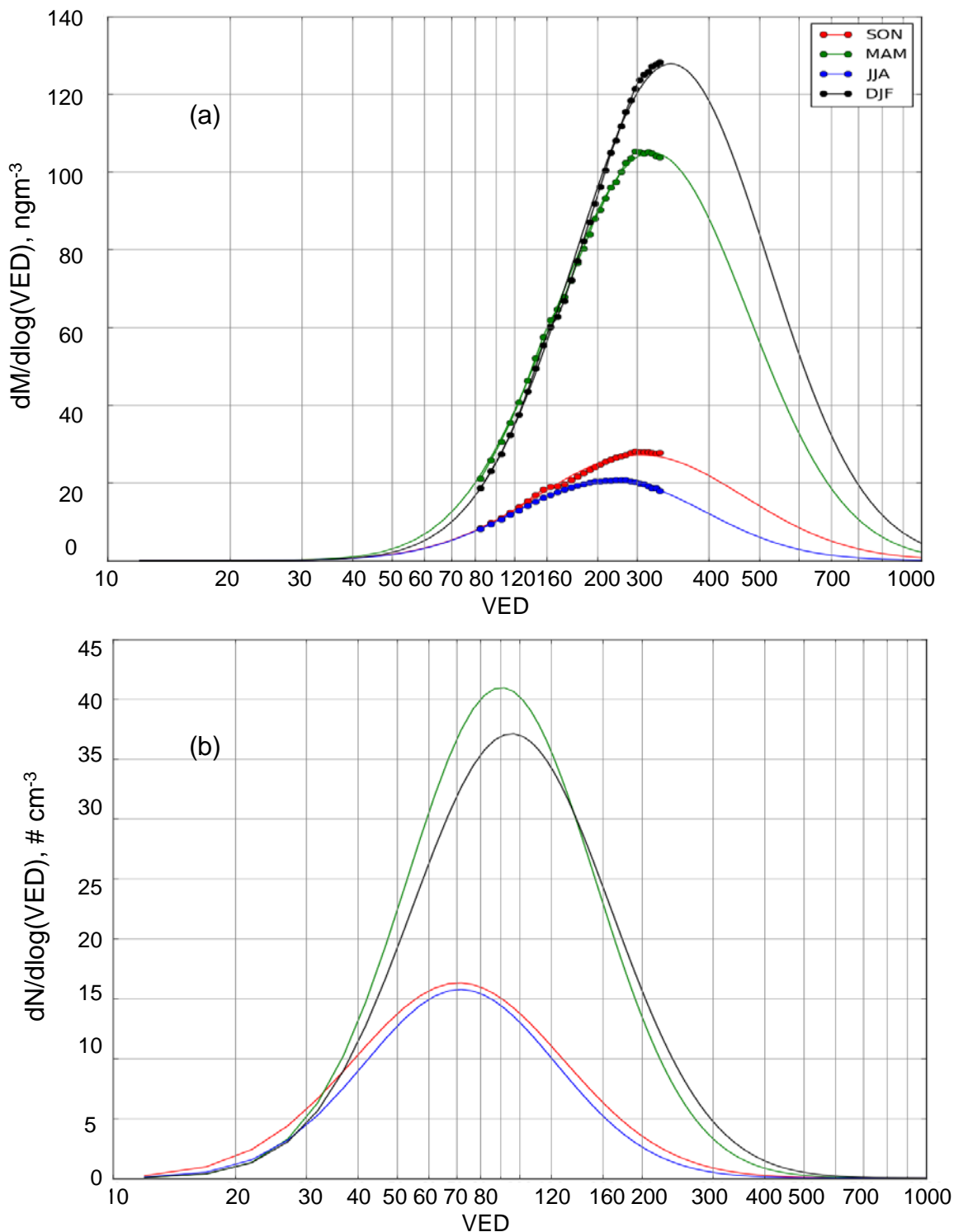
Figure 3: Seasonally-averaged mass (a) and number (b) distributions, by Volume Equivalent Diameter (VED), of rBC particles detected by the SP2 at Alert, NU from March 2011 to December 2013. The number distributions are estimated from the fits to the mass distribution. The black, green, blue, and red data curves represent the three-month average season: winter (DJF), spring (MAM), summer (JJA), and fall (SON), respectively. On average, a modal mass diameter at 225 nm was measured for rBC during winter and around 170 nm during summer. The number distribution shows a mode at 100 nm during winter due to long range transport influence and during the light period in the spring, giving a smaller particle diameter. VED indicates volume equivalent diameter. The solid circles represent the size range of calibration.
