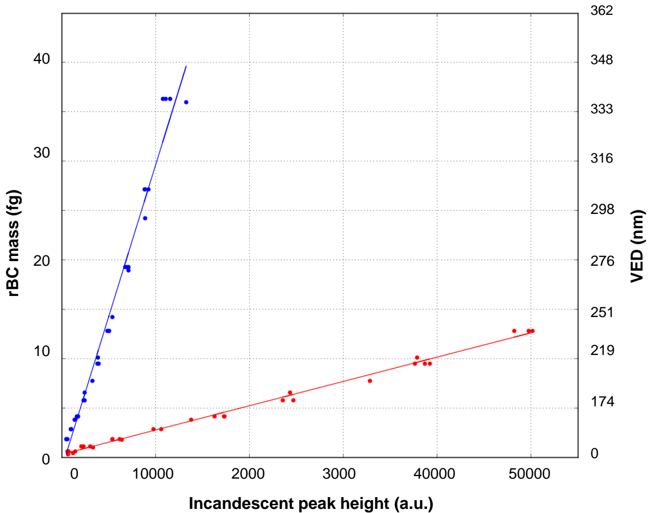
Figure 2: A calibration curve for SP2 #58 shows an incandescent peak height with an arbitrary unit response to rBC mass (fg). The data points in blue circles apply to the low gain channel and those in red circles to the high gain channel. The right hand axis shows the volume equivalent diameter (VED) in nm.
