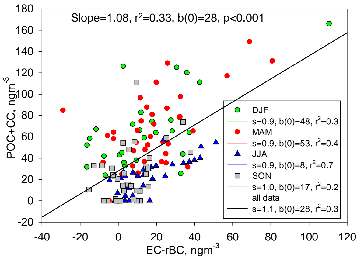
Figure 8: The weak but significant ( p<0.001 ) correlation among the difference between two weekly masses (EC and rBC) at Alert and the oxygenated carbon component as represented by POC+CC, shows some positive tendency indicating incomplete separation of EC from other co-eluting thermal components. The correlation improves for summer (blue symbol, r^2=0.7 ) indicating a more consistent oxygenated source as compared to other seasons where r^2=0.3 .
