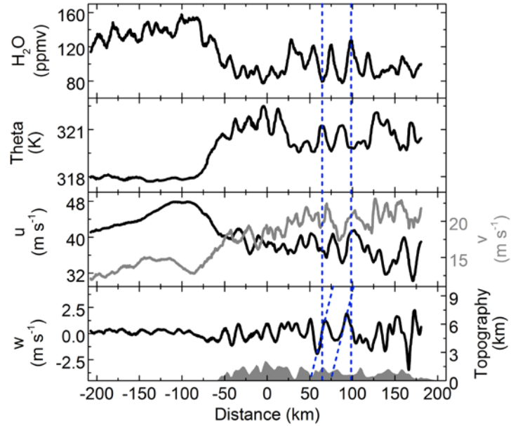
Figure 3. A portion of the time series of the DLR Falcon flight FF04 on 4 July 2014 shown in Figure 2. The measurements were taken during the second flight leg at 8.9 km altitude over the South Island of New Zealand. The distance refers to Mt. Aspiring as the highest summit during this mountain transect (west to east). The vertical blue dashed lines mark single wave events. The diagonal blue dashed lines in the bottom panel connect the maximum or minimum of the vertical wind motion with the respective maximum or minimum in the perturbations of water vapor and theta which displays the phase shift between these parameters.
