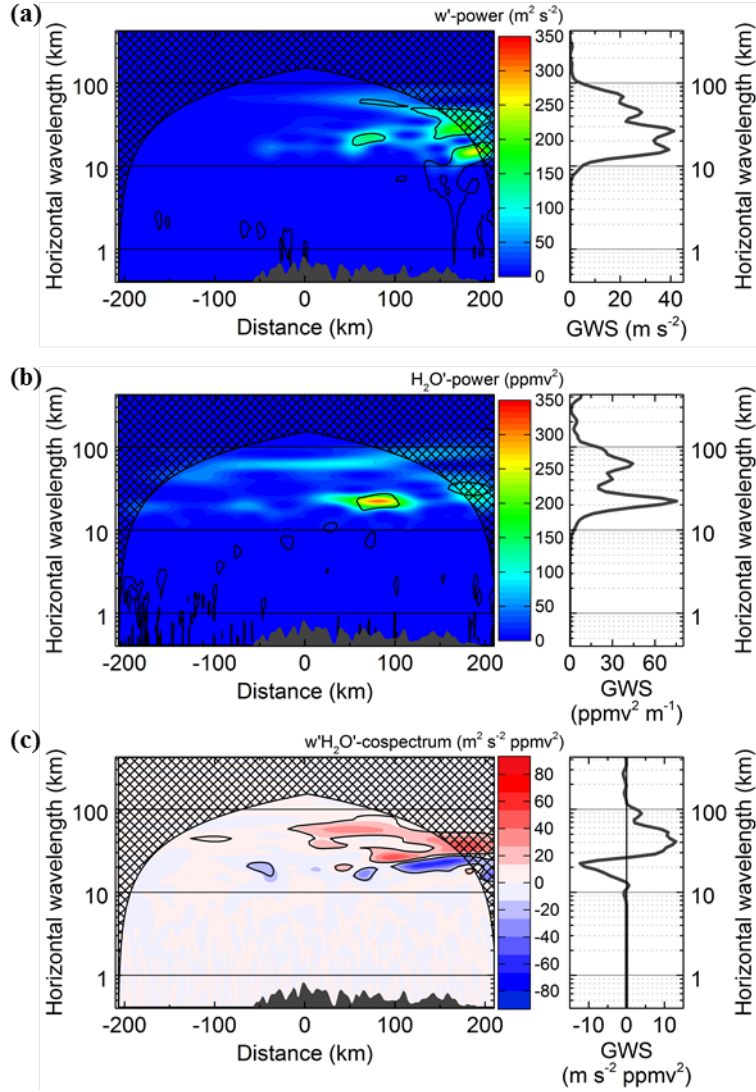
5 Figure 5. Wavelet analysis of the second flight leg of the DLR Falcon flight FF04 shown in Figure 2: (a) power spectrum of vertical wind perturbation w' , (b) power spectrum of water vapor perturbation H_2O' , and (c) cospectrum of the vertical water vapor flux w'H_2O' . The right panels show the corresponding global wavelet spectrum (GWS). Thin black lines around coloured areas are the 95 % confidence level; the crosshatched area is the COI. The topography (maximum mountain height of 2049 m) is represented by the dark grey area in the bottom of each panel.
