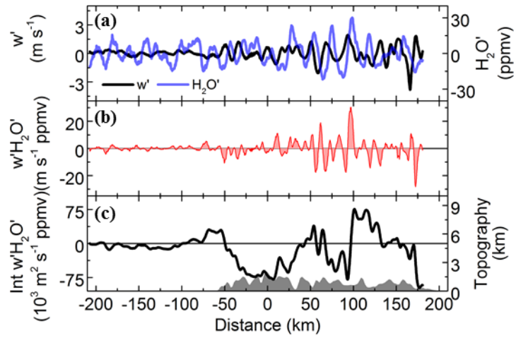
10 Figure 4. Same flight leg as in Figure 3. Shown are components of the vertical water vapor flux. The vertical wind perturbation (black) and the water vapor perturbation (blue) in (a) are combined to the local vertical water vapor flux w'H_2O' (b). The bottom panel (c) shows the integrated vertical water vapor flux \int w'H_2O' dx and the topography.
