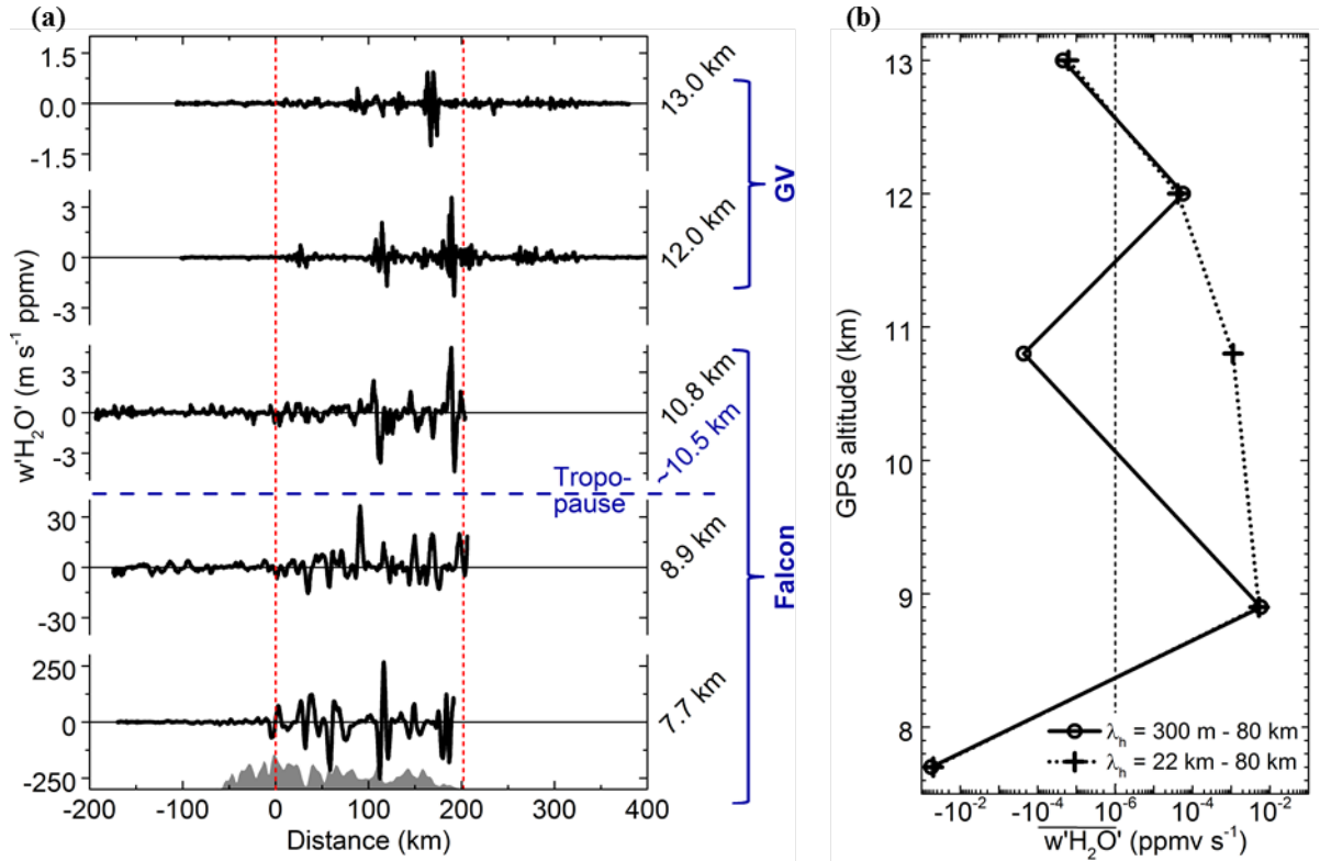
10 Figure 6. (a) Vertical water vapor fluxes using data from DLR Falcon flight FF05 (lower three panels) and NSF/NCAR GV flight RF16 (upper two panels) on 4 July 2014. The fluxes are shown for different flight altitudes over the topography of the Southern Alps. The approximate height of the tropopause at 10.5 km is displayed by the dashed blue line. The red dashed lines mark the region that is used to get the water vapor fluxes shown in panel (b). (b) Vertical profile of the water vapor fluxes integrated over the mountain region with highest mountain wave activity. The profiles are shown for horizontal wavelengths between 300 m and 80 km (solid line) and between 22 km and 80 km (dashed line).
