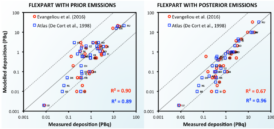
1 2 Figure 9. Country-by-country total cumulative deposition of 137 Cs simulated with 3 FLEXPART model using the prior and posterior emissions versus the estimated ones from the 4 Atlas (De Cort et al., 1998) and from Evangelou et al. (2016). The different countries are 5 highlighted using their official country codes (Austria (AT), Belarus (BY), Belgium (BE), 6 Croatia (HR), Czech Republic (CZ), Denmark (DK), Estonia (EE), Finland (FI), France (FR), 7 Germany (DE), Greece (GR), Hungary (HU), Ireland (IE), Italy (IT), Latvia (LV), Lithuania 8 (LT), Luxembourg (LU), Moldavia (MD), Netherlands (NL), Norway (NO), Poland (PL), 9 Rumania (RU), Russia (RU, European part), Slovak Republic (SK), Slovenia (SL), Spain 10 (ES), Sweden (SE), Switzerland (CH), Ukraine (UA) and United Kingdom (GB)).
