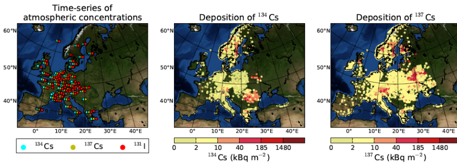
Figure 3. Locations of atmospheric activity concentration measurements of ^{134}\text{Cs} , ^{137}\text{Cs} and ^{131}\text{I} and deposition locations and levels of ^{134}\text{Cs} and ^{137}\text{Cs} over Europe adopted from Evangelidou et al. (2016).
