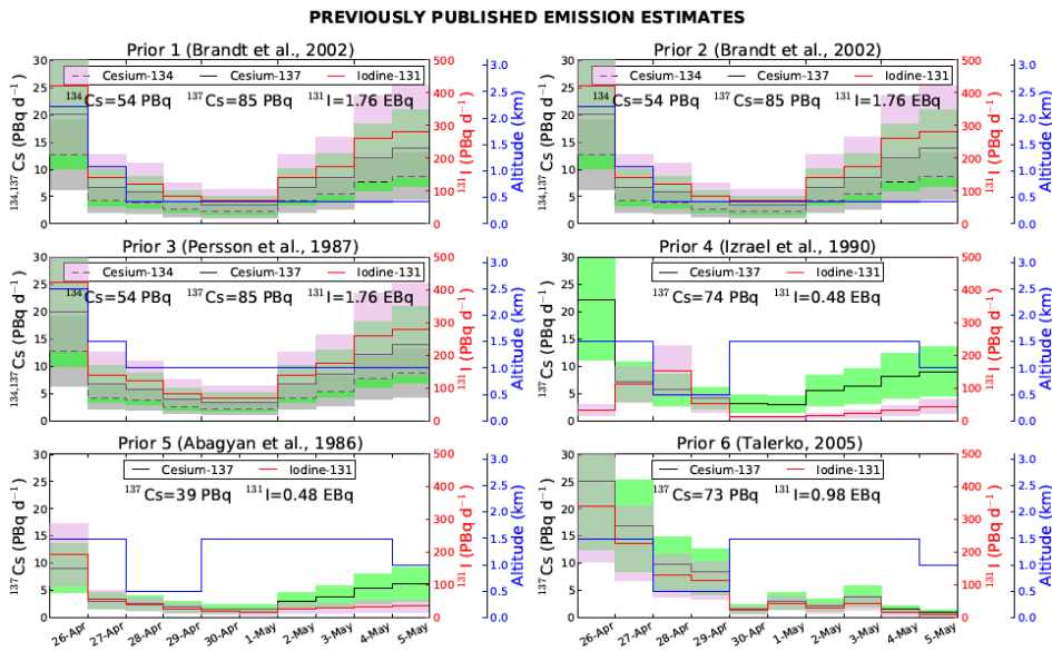
4 Figure 1. Six different profiles of source releases for ^{134}\text{Cs} (black dashed line), ^{137}\text{Cs} (black 5 line) and ^{131}\text{I} (red line), published after the Chernobyl accident. These emissions were used to 6 calculate the a priori (prior) source information and the relative uncertainty of the inversion. 7 Blue line indicates the maximum altitude of the emissions.
