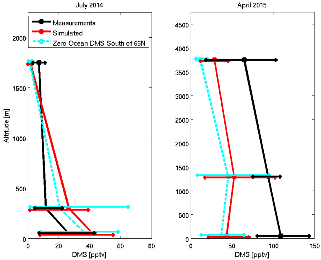
1 2 Figure 5. The campaign-mean vertical profile of DMS from the GEOS-Chem simulation (red line) and 3 measurements (black line) for July 2014 and April 2015. Simulations for zero ocean DMS at latitudes south of 4 66°N (SimZeroBelow66) are shown as cyan dashed line. The 20 th and 80 th percentiles are shown by horizontal 5 bars. 6 7 8 9 10 11 12 13 14 15 16 17 18 19 20
