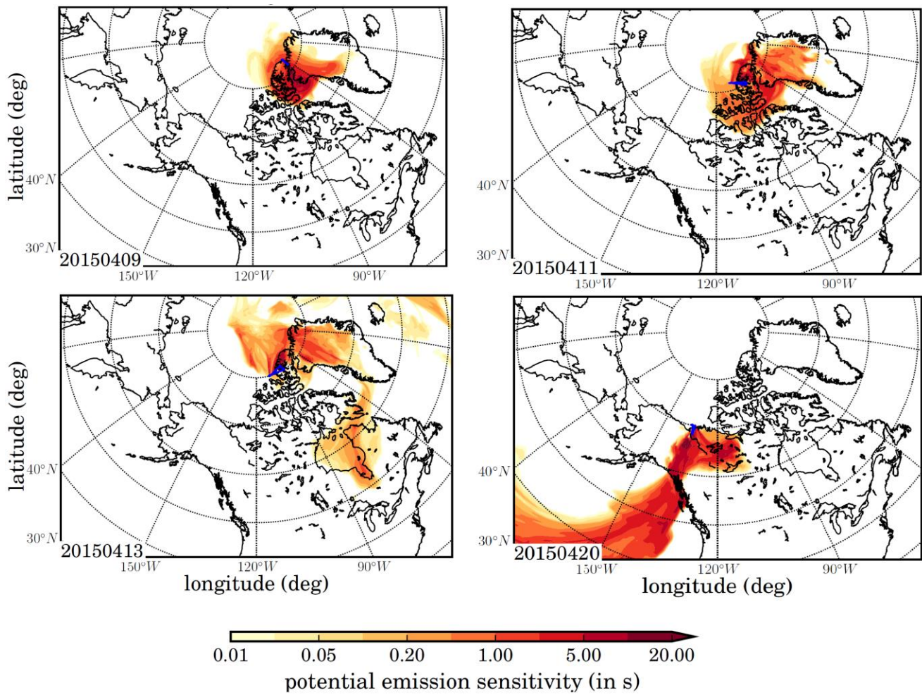
1 2 Figure 7. FLEXPART-ECMWF potential emissions sensitivity simulation plots for 4-day back trajectories for 3 column from 0 to 1000 m on (a) April 9 th (14:45:00 h UTC), (b) April 11 th (18:55:00 h UTC), (c) April 13 th 4 (18:27:00 h UTC), and (d) April 20 th (22:26:00 h UTC), 2015. The color bars indicate air mass residence time 5 (seconds) before arriving at the aircraft location. The blue lines show Polar 6 aircraft routes. 6 7 8 9 10 11 12 13 14
