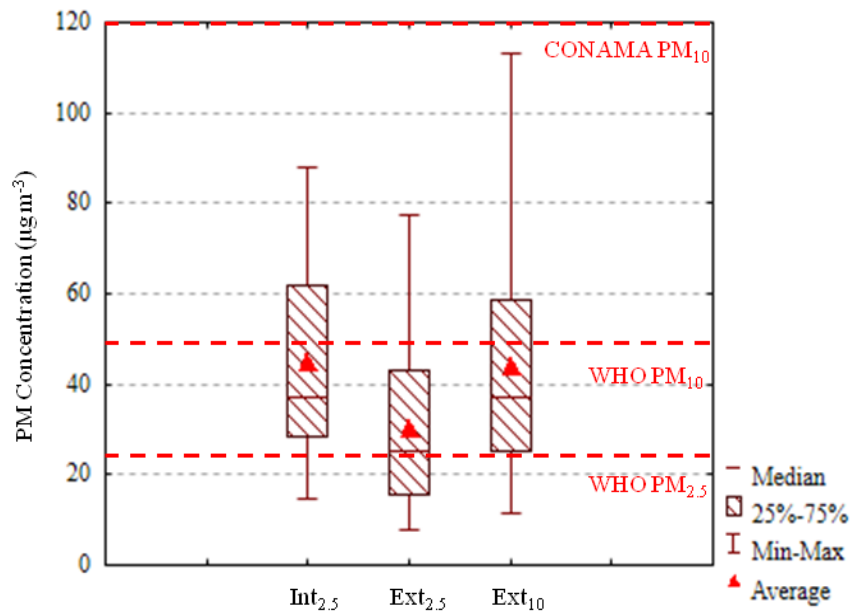
1055 Figure 3. Box plot for particulate matter concentrations in the intensive and extensive campaigns.
