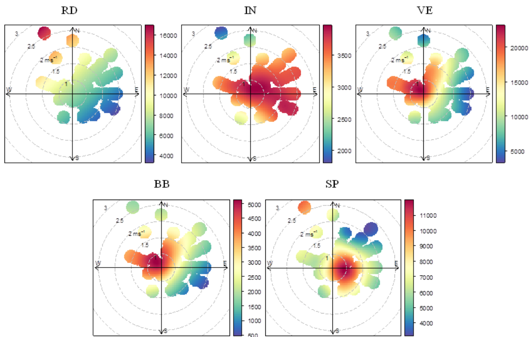
1085 Figure 10. Polar plots of sources contributions in São Paulo ( \text{ng m}^{-3} and \text{m s}^{-1} ).
