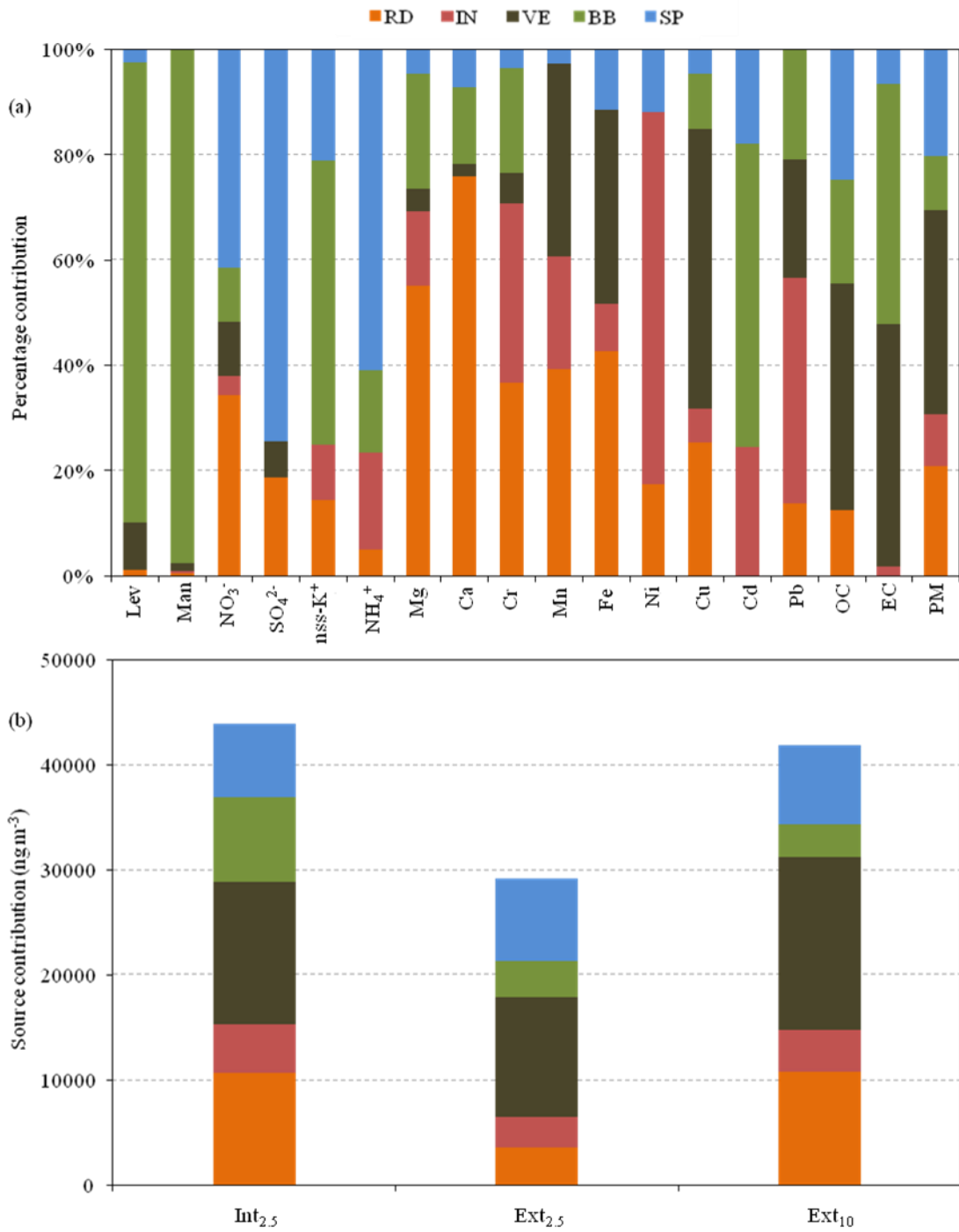
Figure 9. (a) Profile of species for each source (RD - Road dust, SP - Secondary processes, IN - Industrial, VE - Vehicular, BB - Biomass burning, VE - Vehicular, IN - Industrial and RD - Road dust, SP - Secondary processes) (b) Contribution of sources for each campaign.
