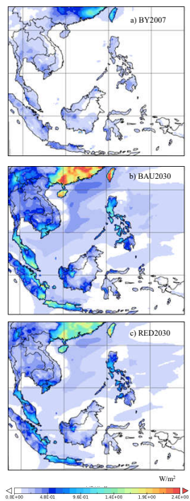
Figure 4: Spatial distribution of annual average BC DRF under BY2007, BAU2030 and RED2030 scenario.
