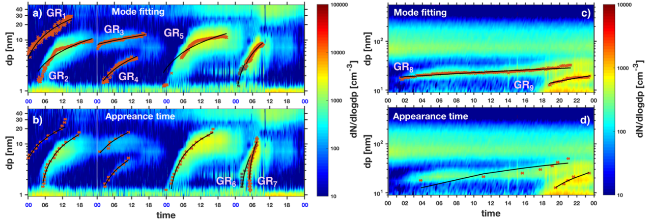
Figure 5. Comparison of growth rates for nine growth modes ( GR_i , i = 1 \dots 9 in figure) determined by the mode-fitting method (a & c) and by the appearance time method (b & d), from the AIS measurement for 9 – 12 March 2011 (left-hand-side column) and from the DMPS measurement for 25 Feb. 2011 (right-hand-side column). Growth rates estimated from linear fittings with root-mean-square errors expressed as uncertainties are shown in Table 1. The red or grey dots depict the estimated size evolution of ions/particles with respect to time determined by the mode fitting or appearance time methods, with the linear fits to these size-time relationships shown as black lines.
