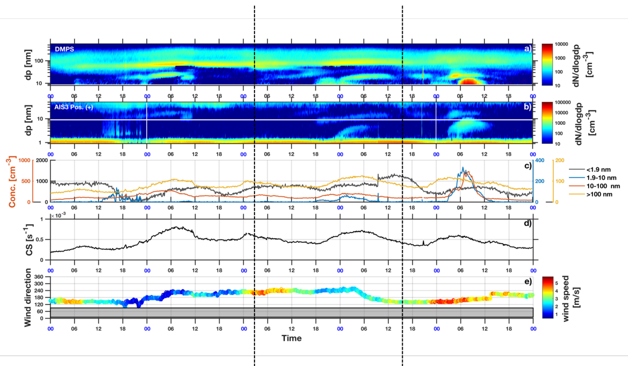
Figure 4. Consecutive multi-mode formation and growth events observed during 12-16 February 2011. a) DMPS spectra; b) AIS positive polarity spectra; c) ion and particle concentrations in four different size ranges 0.9-1.9 nm (ions), 1.9-10 nm (ions), 10-100 nm (total particles), and total particles of diameters above 100 nm; d) CS; and e) wind direction, colour-coded with wind speed. The white line in b) indicates the lower limit of the DMPS size range. The grey band in e) represents the contaminated wind sector. The two vertical dashed lines are to outline the three NPF occurred on 14-15 February 2011. Data are presented in UTC.
