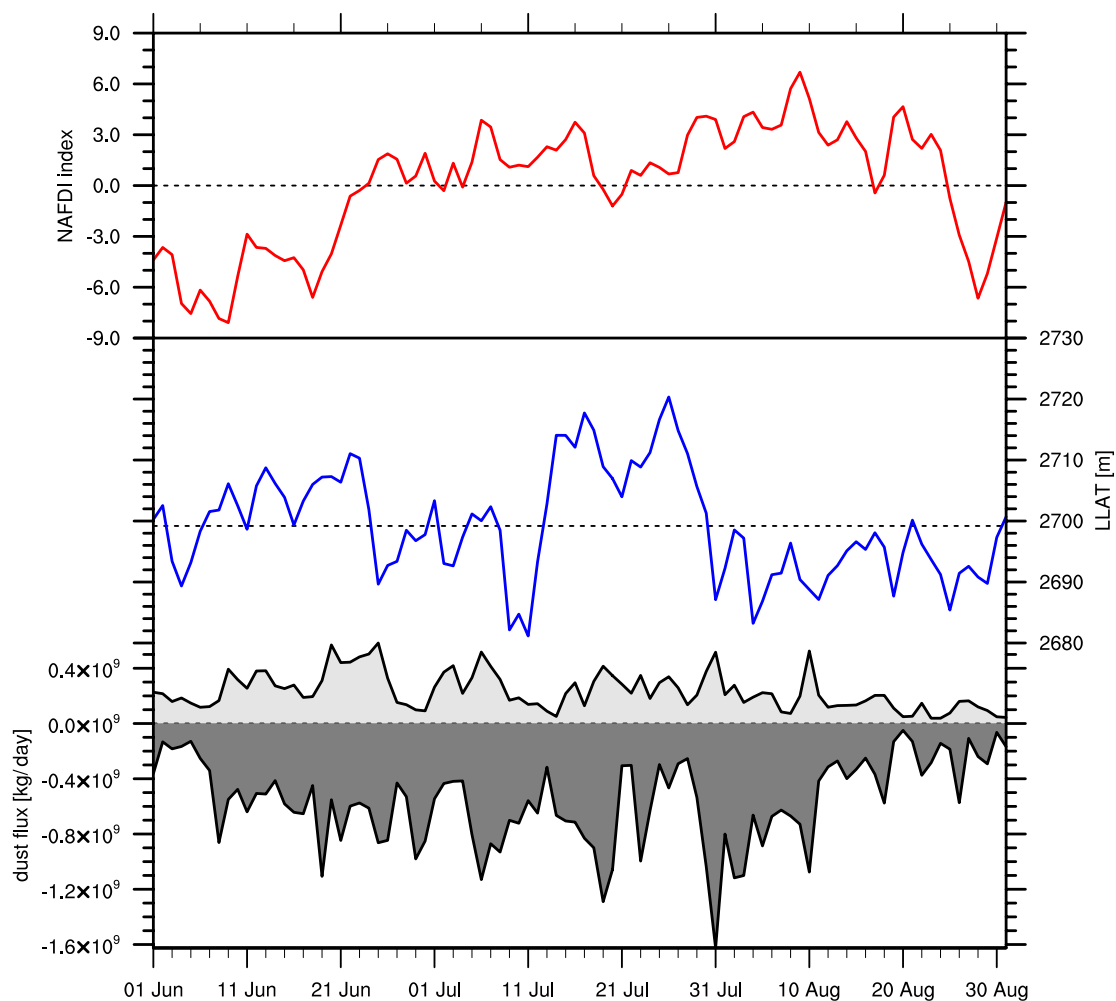
Figure 12. Time series of the NAFDI index (red) indicating the strength of the Harmattan, the LLAT (blue) representing the depth of the SHL, and the westward (dark grey) and eastward (light grey) dust flux at 20^\circ\text{W} integrated over the total column (0-22km altitude) and the latitudinal band between 10 and 25^\circ\text{N} .
