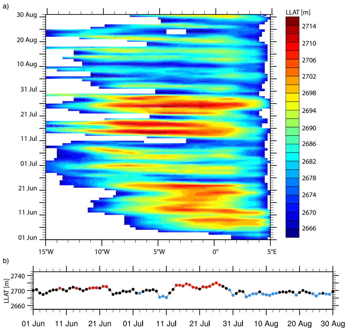
Figure 8. (a) Hovmöller diagram of low-level atmosphere thickness (LLAT) [m] representing the SHL at 23°N. (b) Time series of maximum LLAT [m] for June to August 2013. Blue circles indicate daily LLAT maximum values less than the 25th percentile, red circles indicate daily LLAT maximum values above the 75th percentile. The LLAT is calculated from COSMO-MUSCAT simulation following Lavaysse et al. (2009).
