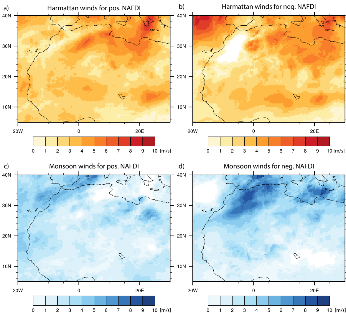
Figure 6. Composite of meridional winds for 75th percentile (positive values) and 25th percentile (negative values) of the NAFDI index values. The meridional winds [m/s] are shown separately for northerly winds referring to the Harmattan (a, b), and southerly winds referring to the Monsoon (c, d).
