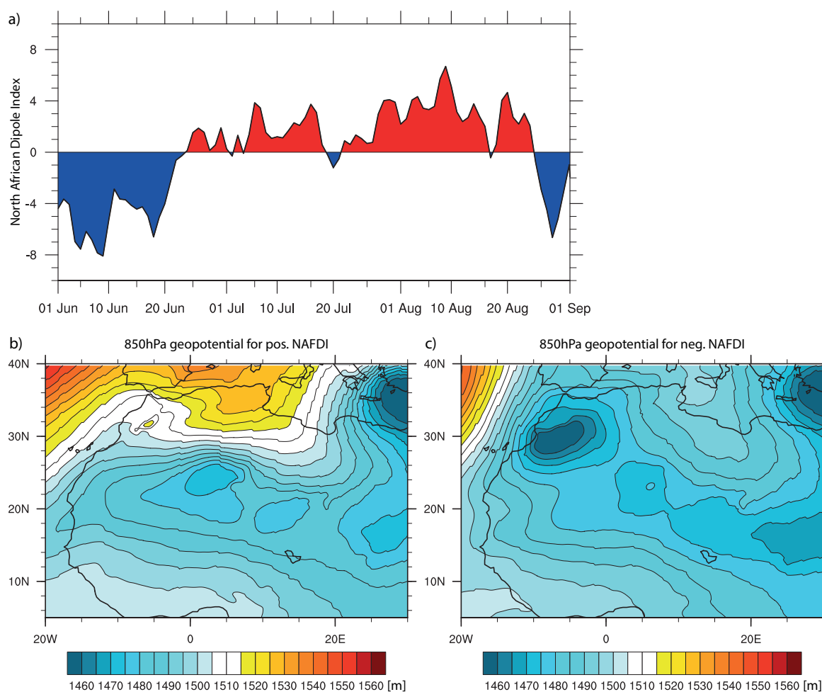
Figure 4. (a) North African Dipole Intensity index calculated following Eq. 1 reflecting the strength of the Harmattan flow over North Africa. (b) Composite of 850hPa geopotential height [m] days within the 75th percentile range of the NADI index values, and (c) for days within the 25th percentile range.
