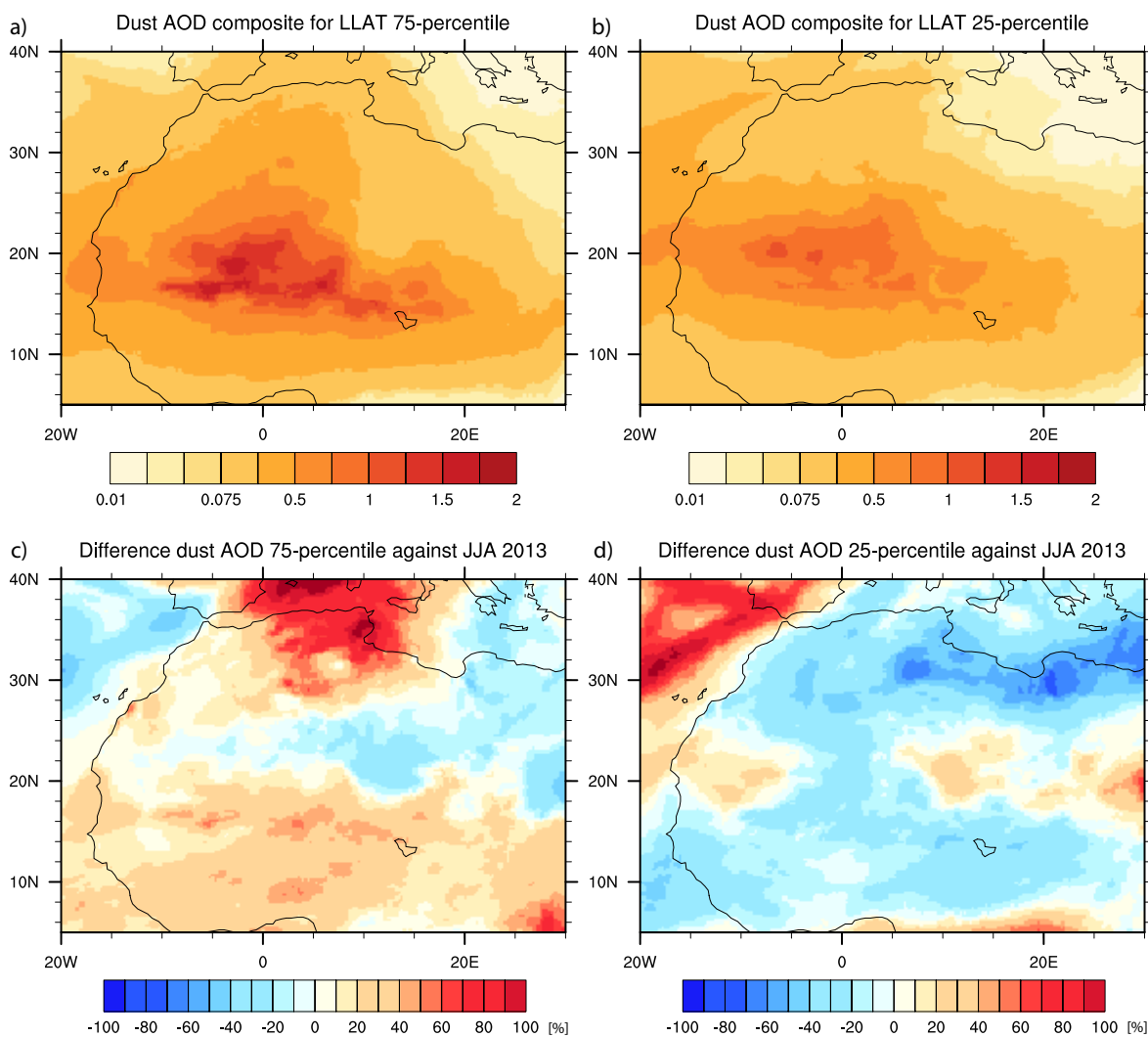
Figure 9. Composite of dust AOD for the days corresponding to the 75th percentile (a) and 25th percentile (b) of the LLAT. See further Fig. 8 for the assignment of the days to the 25th and 75th percentile respectively. (c) and (d) show the relative difference to the JJA 2013 mean.
