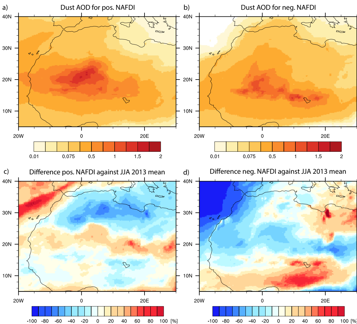
Figure 5. Composite of dust AOD for days within the 75th percentile (a) and 25th percentile of the NAFDI index values. (c) and (d) show the relative difference to the JJA 2013 mean.
