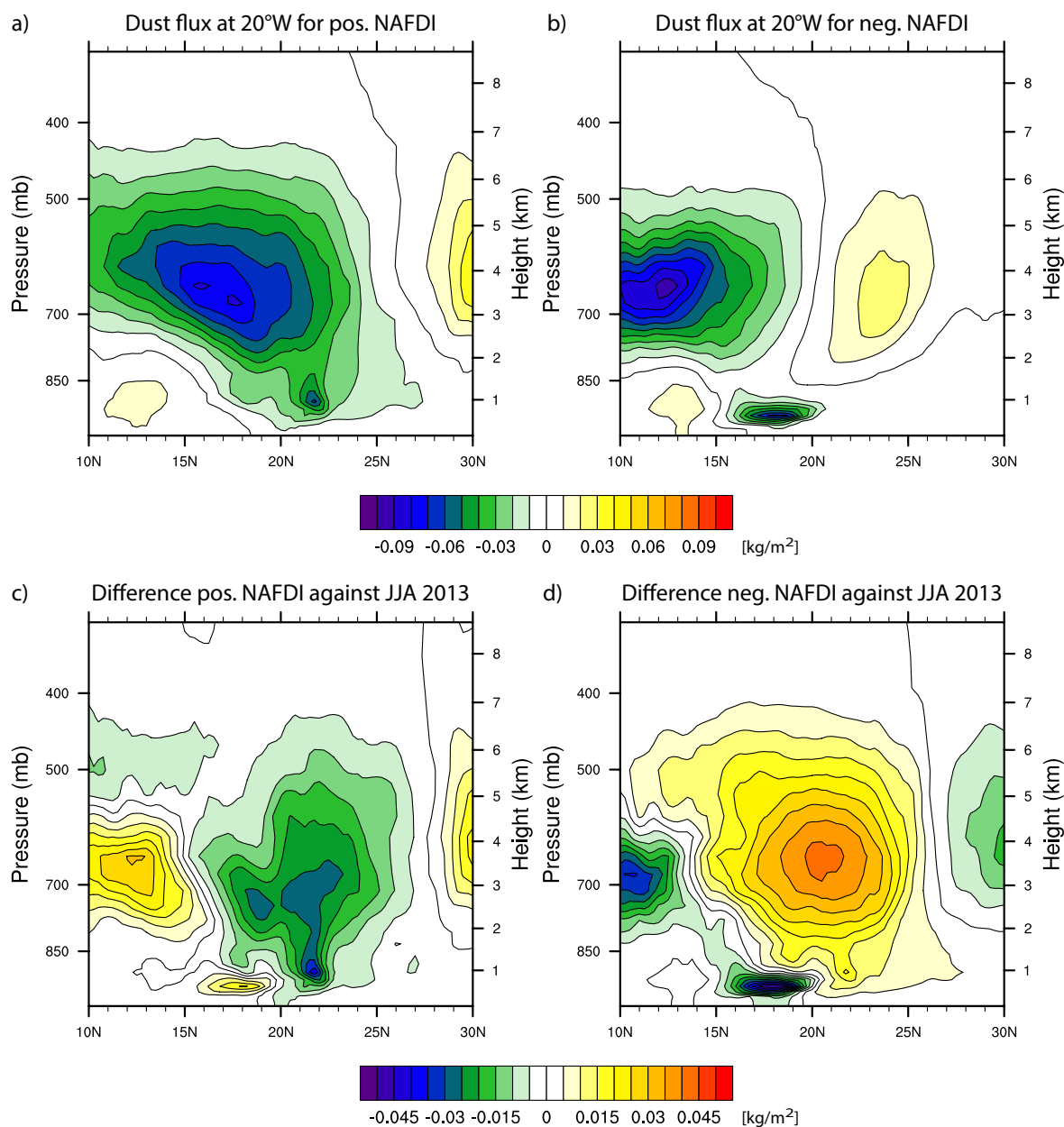
Figure 7. Composite plots of the vertically integrated zonal dust flux [ \text{kg}/\text{m}^2 ] at 20°W for the days out of June, July, August 2013, which correspond to the 75th percentile (a) and 25th percentile (b) of NAFDI index values. Dust export towards the North Atlantic is represented by negative values, positive values indicate transport back to the North African continent. Dust fluxes are totals over the 10-25°N latitudinal band. Differences in dust flux compared against the JJA 2013 mean dust flux are shown in (c) and (d).
