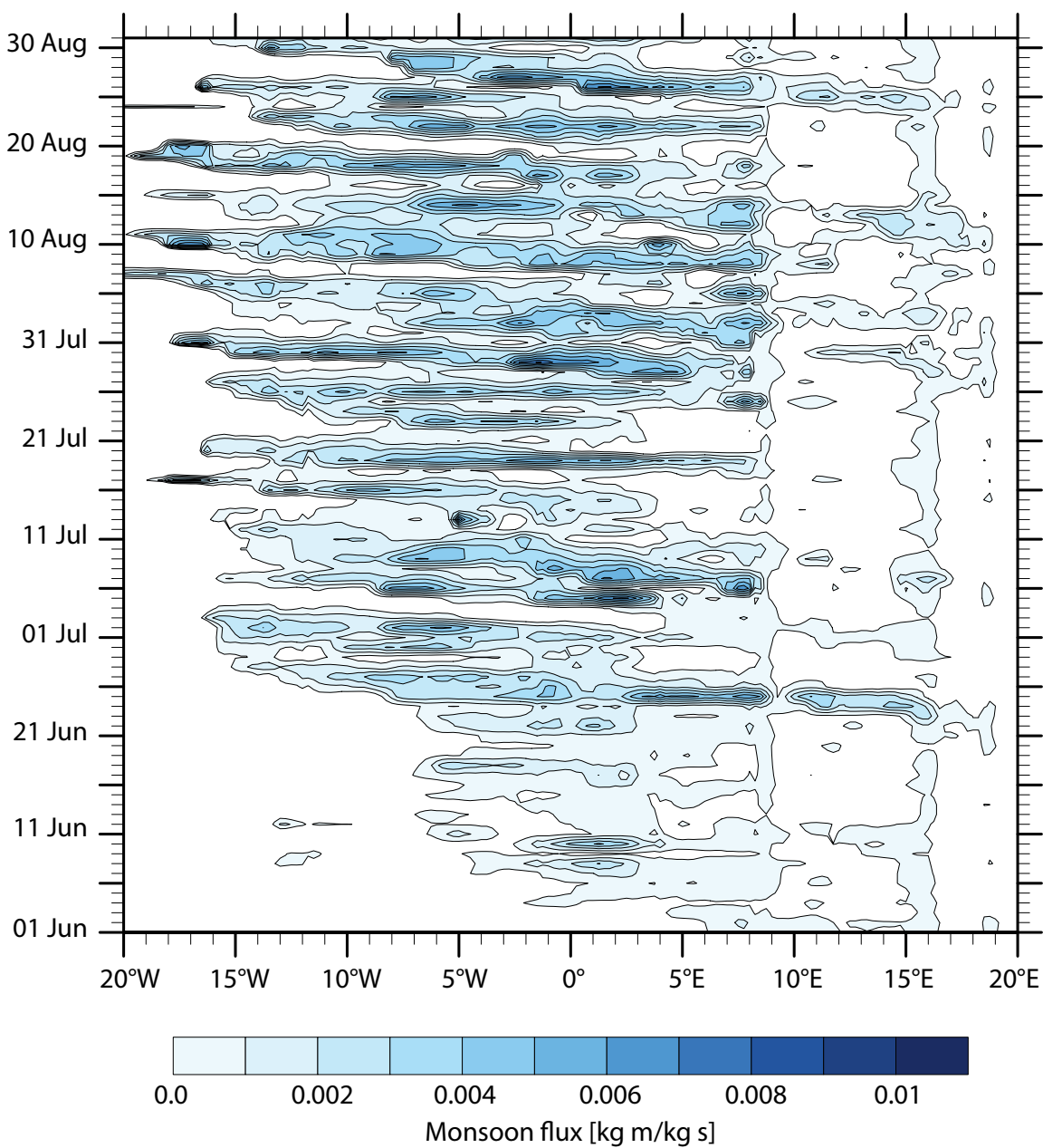
Figure 10. Meridional monsoon flux [kgm/kg s] at 20°N at surface level calculated as the product of the northward component of the meridional wind and the specific humidity, both at 10m above ground level.
