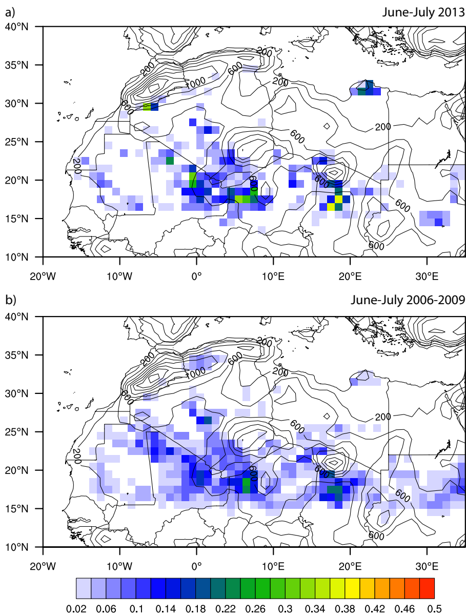
Figure 1. Occurrence frequency of dust source activation (fraction of days with dust occurrence) for the two-month period June and July for 2013 (a) and the four-year period 2006-2009 (b). Topography [m] is given by the black solid lines at 200m intervals.
