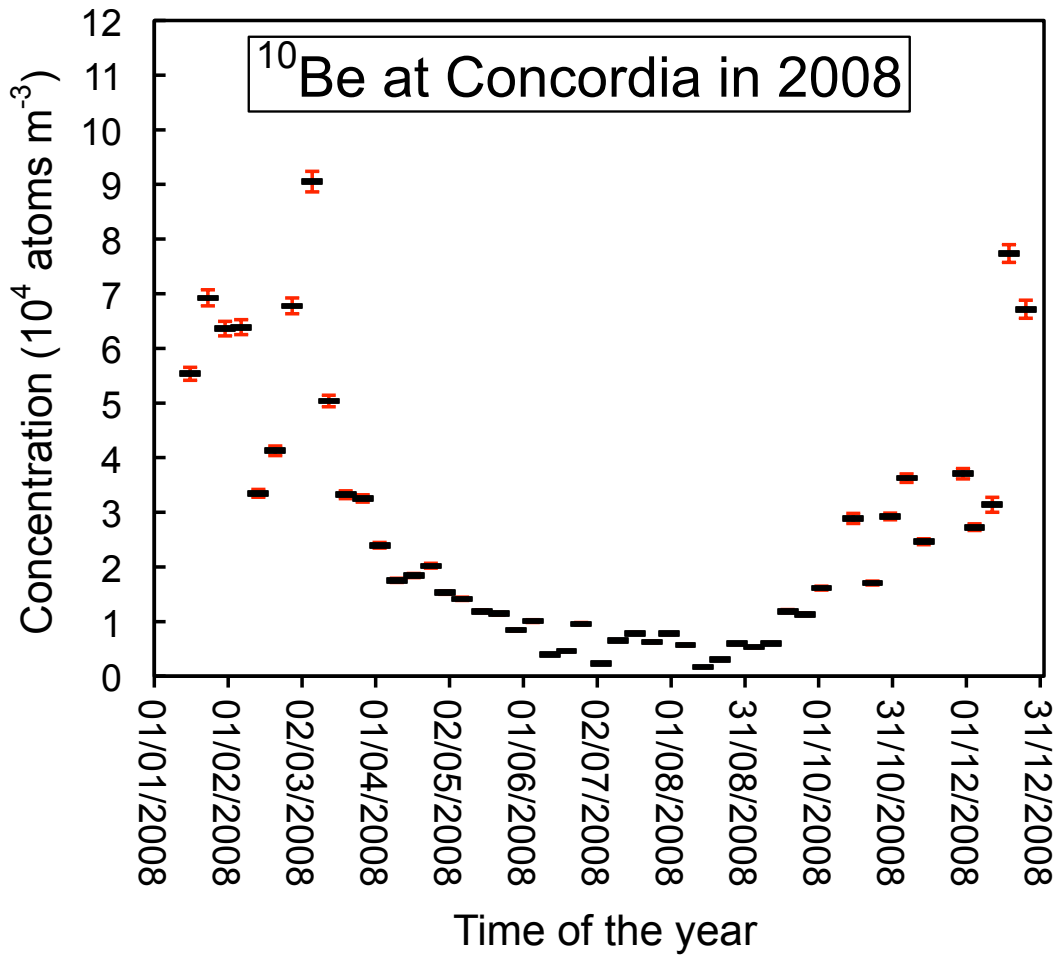
5 Figure 9. Annual cycle of ^{10}\text{Be} concentrations in 2008 at Concordia. Vertical bars (in red) refer to AMS uncertainties (see Sect. 2).
