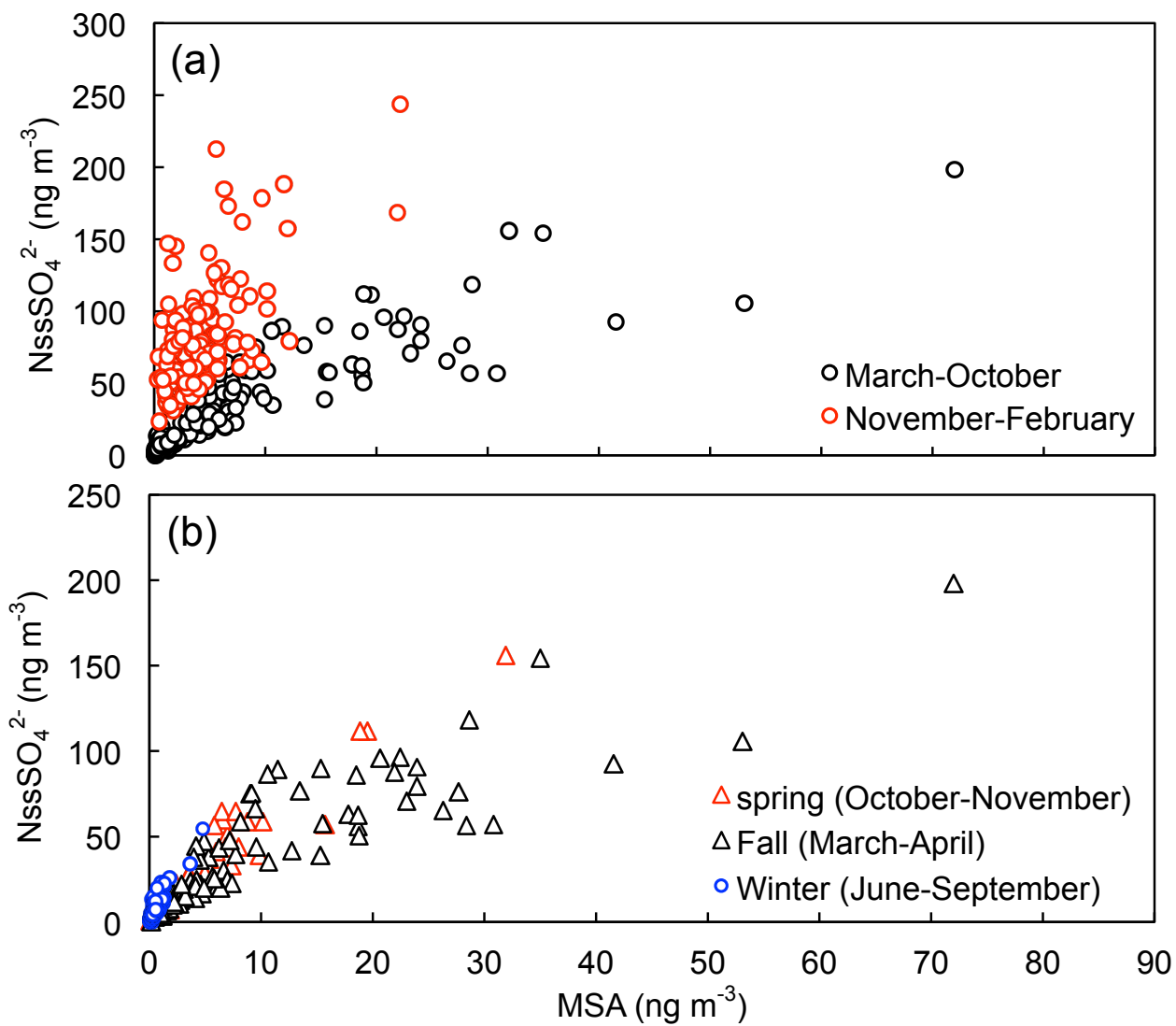
Figure 10. Correlation of nssSO 4 with MSA concentrations observed at Concordia on HV bulk aerosol samples. (a): All data (red circles highlight mid-summer samples), (b): Spring to fall samples.
