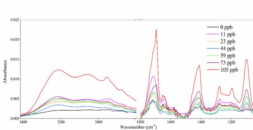
Figure 4: IR spectra of aerosols from the cyclohexene/NOx/SO 2 system under different SO 2 concentrations.
