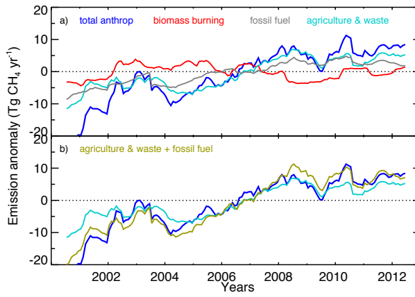
10 Figure 3: 12-month running mean of global annual methane anthropogenic emission anomalies ( \text{Tg CH}_4 \text{ yr}^{-1} ) inferred by the ensemble of inversions (only mean values of the ensemble are represented) for (a) total anthropogenic, biomass burning, fossil fuel and, agriculture and waste sources. On the (b) panel, total anthropogenic and, agriculture and waste source anomalies are recalled on top of the sum of the anomalies from agriculture and waste, and fossil fuels sources.
