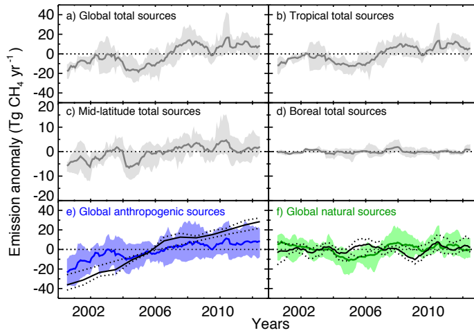
5 Figure 2: 12-month running mean of annual methane emission anomalies (in \text{Tg CH}_4 \text{ yr}^{-1} ) inferred by the ensemble of inversions (mean as the solid line and min/max range as the shaded area) in grey for (a) global, (b) tropical, (c) mid-latitudes and (d) boreal total sources; in blue for (e) global anthropogenic sources and in green for (f) natural sources. The solid and dotted black lines represent the mean and min/max range (respectively) of the bottom-up estimates: anthropogenic inventories in (e) and ensemble of wetland models in (f). The vertical scale is divided by 2 for the mid-latitude and boreal regions.
