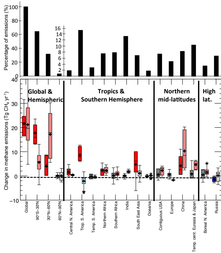
Figure 4: Top: Contribution to the global methane emissions by region (in %, based on the mean top-down estimates over 2003-2012 from Saunois et al. (2016)). Bottom: Changes in methane emissions 2002-2006 and 2008-2012 at global, hemispheric and regional scales in TgCH 4 yr -1 . Red boxplots indicate a significant positive contribution to emission changes (first and third quartiles above zero), blue boxplots indicate a significant negative contribution to emission changes (first and third quartiles below zero), grey boxplots indicate not-significant emission changes. Dark coloured boxes are for top-down (five long inversions) and light coloured for bottom-up approaches (see text for details). Median is indicated inside each boxplot (see Methods, section 2). Mean values, reported in the text, are represented with "+" symbols. Outliers are represented with stars. (Note: the bottom-up approaches that provide country estimates (and not maps, USEPA and FAOSTAT) have not been processed to provide hemispheric values. As a result the ensemble used for the three hemispheric regions differs from the ensemble used for the global and regional estimates.)
