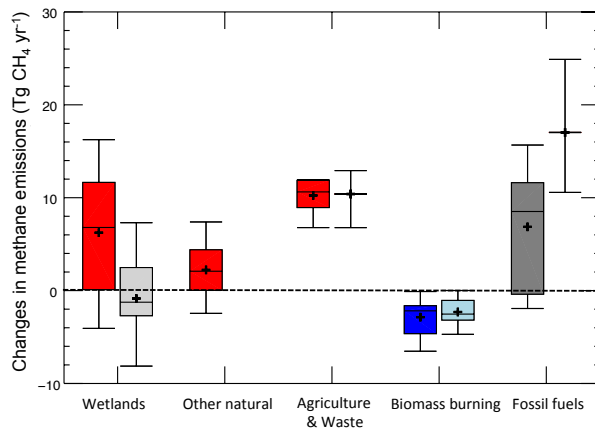
5 Figure 5: Changes in methane emissions between 2002-2006 and 2008-2012 in Tg CH 4 yr -1 for the five source types. Red boxplots indicate a significant positive contribution to emission changes (first and third quartiles above zero), blue boxplots indicate a significant negative contribution to emission changes (first and third quartiles below zero), grey boxplots indicate non-significant emission changes. Dark (light) coloured boxes are for top-down (bottom-up) approaches (see text for details). Median is indicated inside each boxplot (see Methods, Section 2). Mean values, reported in the text, are represented with "+" symbols.
