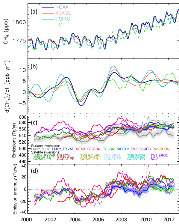
5 Figure 1: Evolution of the global methane cycle since 2000. (a) Observed atmospheric mixing ratios (ppb) as synthesized for four different surface networks with a global coverage (NOAA, AGAGE, CSIRO, UCI). (b) Global Growth rate computed from (a) in ppb/yr. 12-month running mean of (c) annual global emission (TgCH 4 .yr -1 ) and (d) annual global emission anomaly (TgCH 4 .yr -1 ) inferred by the ensemble of inversions.
