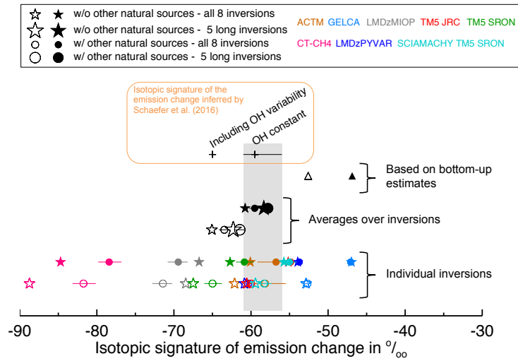
5 Figure 6: Isotopic signature (in ‰) of the emission change between 2002-2006 and 2008-2012 based on Eq. 1 and the isotopic source signatures from Schaefer et al. (2016) and Schwietzke et al. (2016) in filled and open symbols respectively. The range of the isotopic signature of the emission change derived by the box-model of Schaefer et al. (2016) is indicated as the grey shaded area when assuming constant OH. The isotopic signatures derived from the ensemble of bottom-up estimates are shown with triangle symbol. The individual inversions are shown in colour. The mean inversion estimates are shown with stars and circles, without and with taking into account the “other natural” sources, respectively. The range around the circle indicates the range due to the choice of the isotopic source signature for the “other natural” source between -40 ‰ and -57 ‰ (see text).
