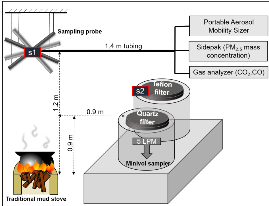
Figure 1: Schematic representation of the experimental setup. S1 and S2 denote the position of the wireless optical sensors.
