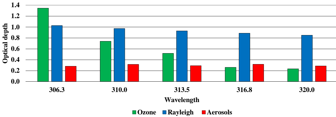
Figure 11: Comparison of long-term averages for the total ozone optical depth, the optical depth of Rayleigh scattering and AOD, 1994–2016.
