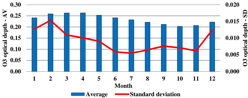
15 Figure 12: Average monthly characteristics of the total ozone optical depth for the wavelength of 320 nm, 1994–2016.
