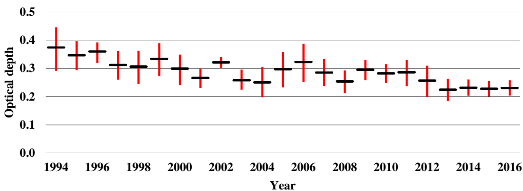
15 Figure 9: Annual averages of AOD and their uncertainty for the wavelength of 320 nm, 1994–2016.
