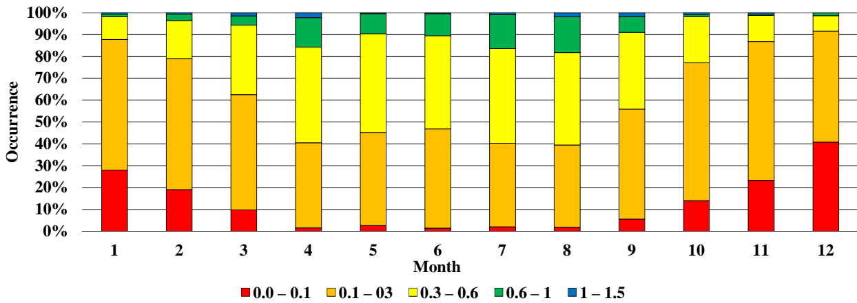
Figure 14: Relative distribution of daily average values of AOD for the wavelength of 320 nm, 1994–2016.
