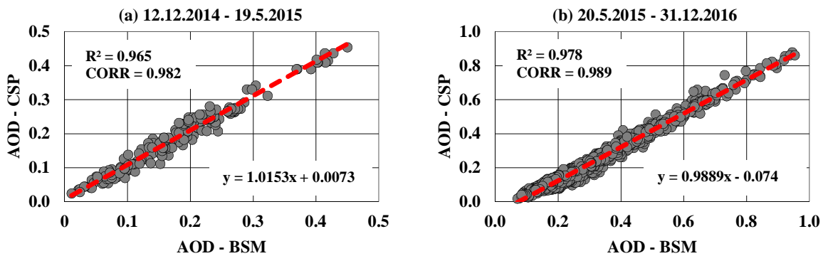
Figure 8: Comparison of AOD values for the wavelength of 320 nm obtained by means of the BSM and the Cimel sunphotometer (CSP).
