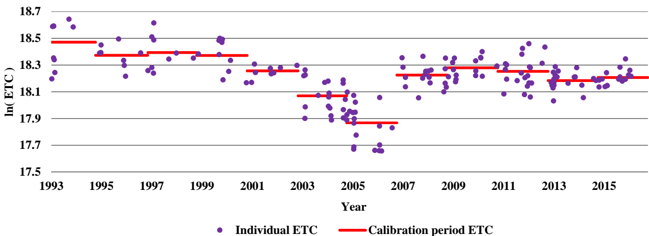
Figure 4: Trend of ETCs values for the wavelength of 320 nm during 12 intercalibration periods, 18.8.1993–13.5.2017.
