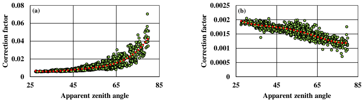
Figure 3: Size of the correction factor for the elimination of stray-light effect depending on the apparent zenith angle (a) for the wavelength of 306.3 nm; (b) for the wavelength of 320 nm. 15
