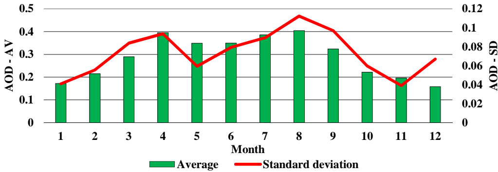
10 Figure 13: Average monthly characteristics of the AOD for the wavelength of 320 nm, 1994–2016.
