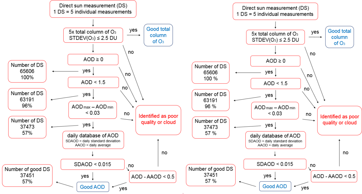
10 Figure 1: Schematic illustration of the DS measurement quality control procedure process that includes cloud screening as well . The number of DS measurements for the period 18.8.1993–13.5.2017 that satisfy the respective criterion is indicated on the left side.
