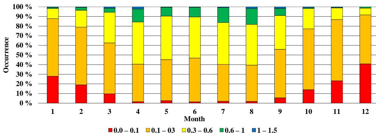
Figure 14: Relative contribution distribution of daily average values of AOD to the monthly averages for the wavelength of 320 nm, 1994–2016.
