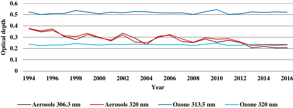
5 Figure 10: Comparison of values of average annual optical depth for the selected wavelengths for ozone and aerosols, 1994–2016.
