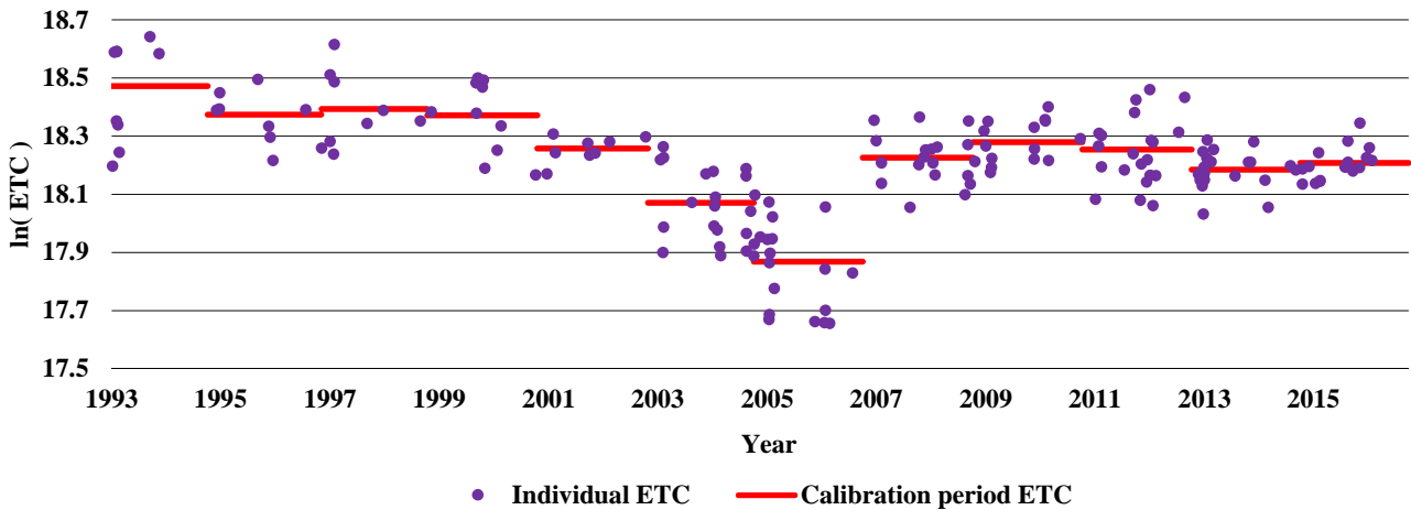
Figure 4: Time series Trend of ETCs values for the wavelength of 320 nm during 12 intercalibration periods, 18.8.1993–13.5.2017.
