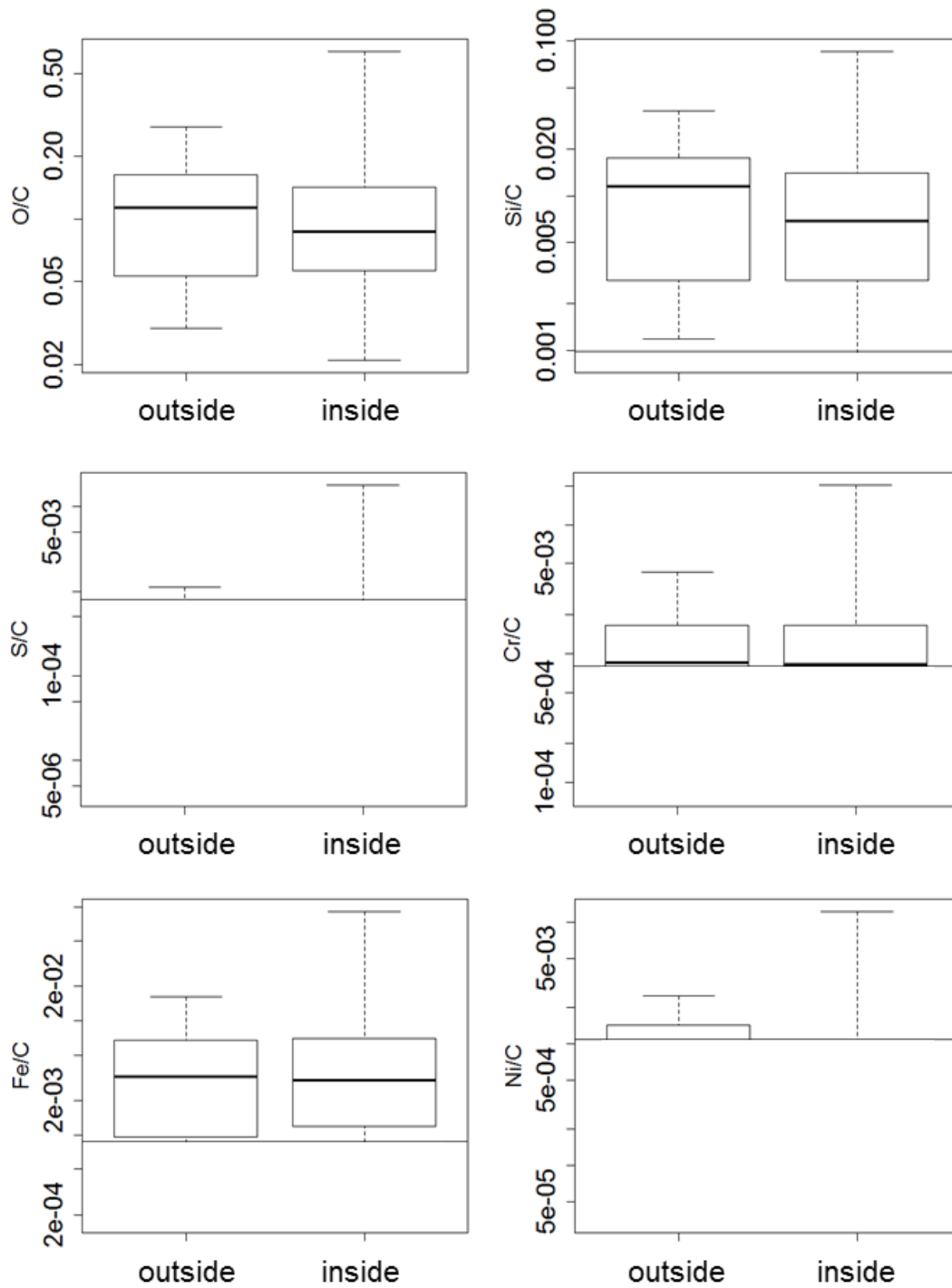
Figure 8: Censored boxplots of element ratios (atom %) relative to C, separately for outside and inside the polar vortex. Sample K was excluded from the analysis due to the different substrate used. Lower and upper quartiles appear as a box, minimum and maximum values as whiskers. Values below detection limit (horizontal line) are not shown.
