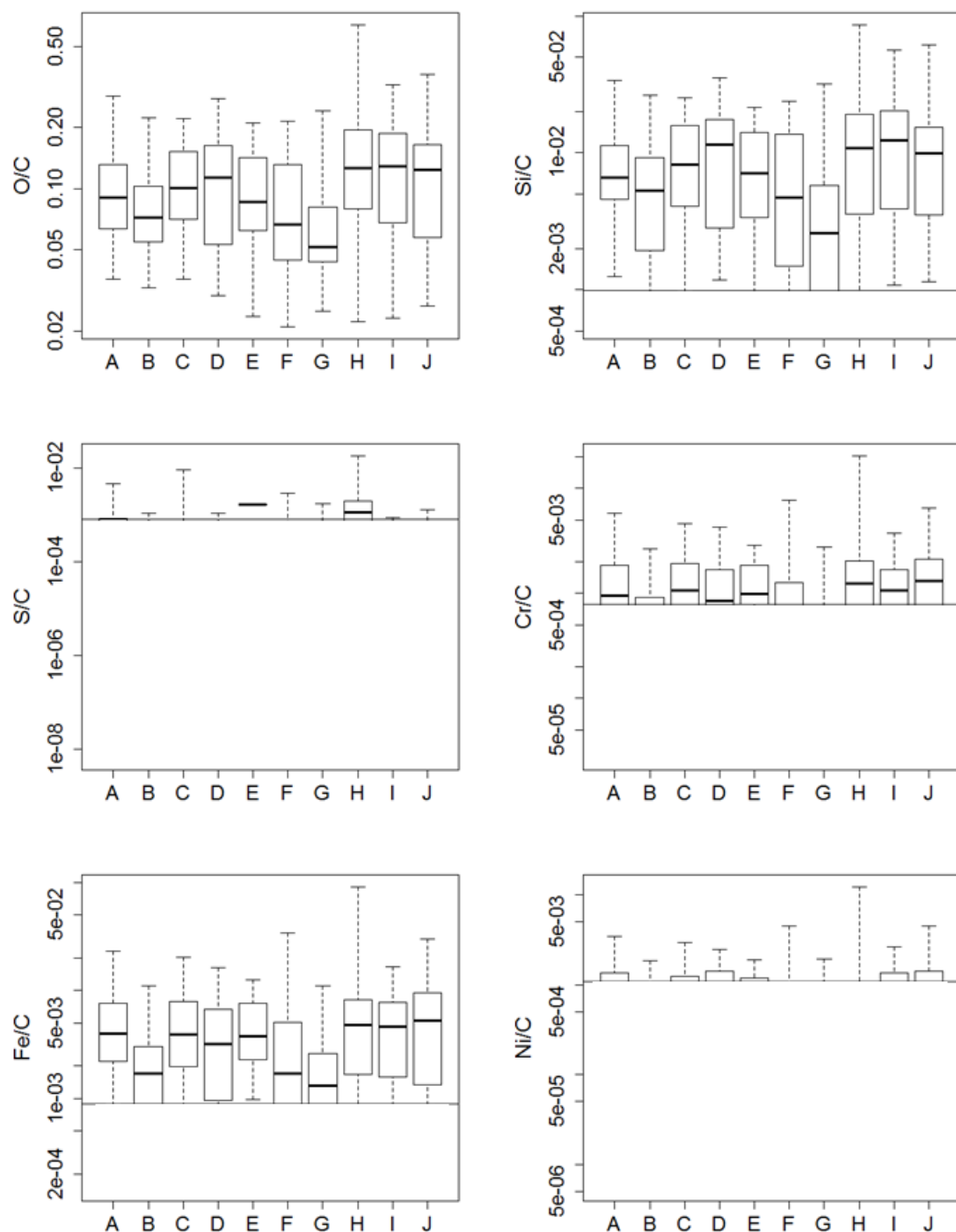
Figure 6: Censored boxplots of element ratios relative to C (atom %) determined by SEM-EDX (30 particles per sample). Sample K is not shown due to the different substrate used. Lower and upper quartiles appear as a box, minimum and maximum values as whiskers. Values below detection limit (horizontal line) are not shown.
