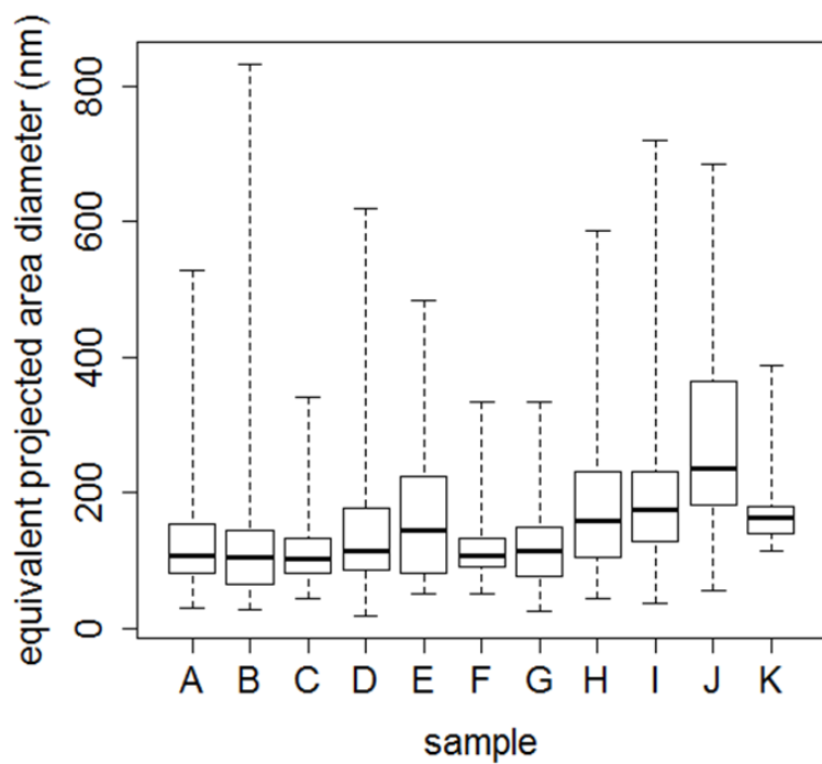
Figure 3: Boxplot of particle size (equivalent projected area diameter D_{pa} ). Lower and upper quartiles appear as a box, minimum and maximum values as whiskers.
