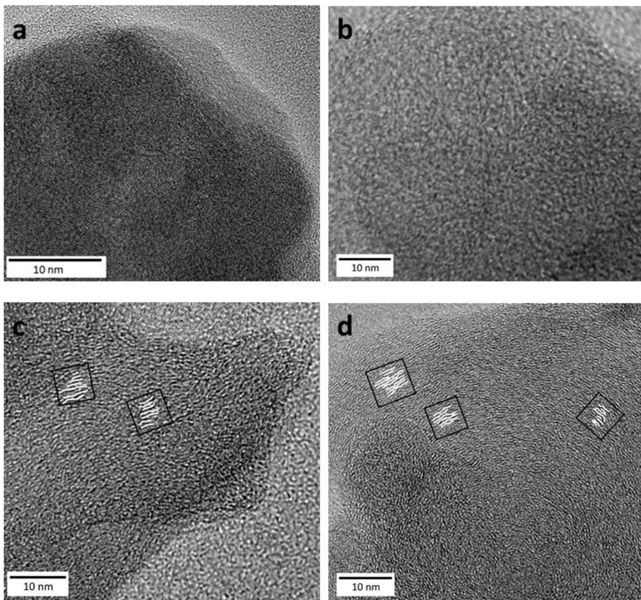
Figure 7: High resolution TEM image of individual refractory carbonaceous particles from sample G (17.4 km altitude): (a, b) completely amorphous particles, (c, d) particles showing small regions with ordering.
