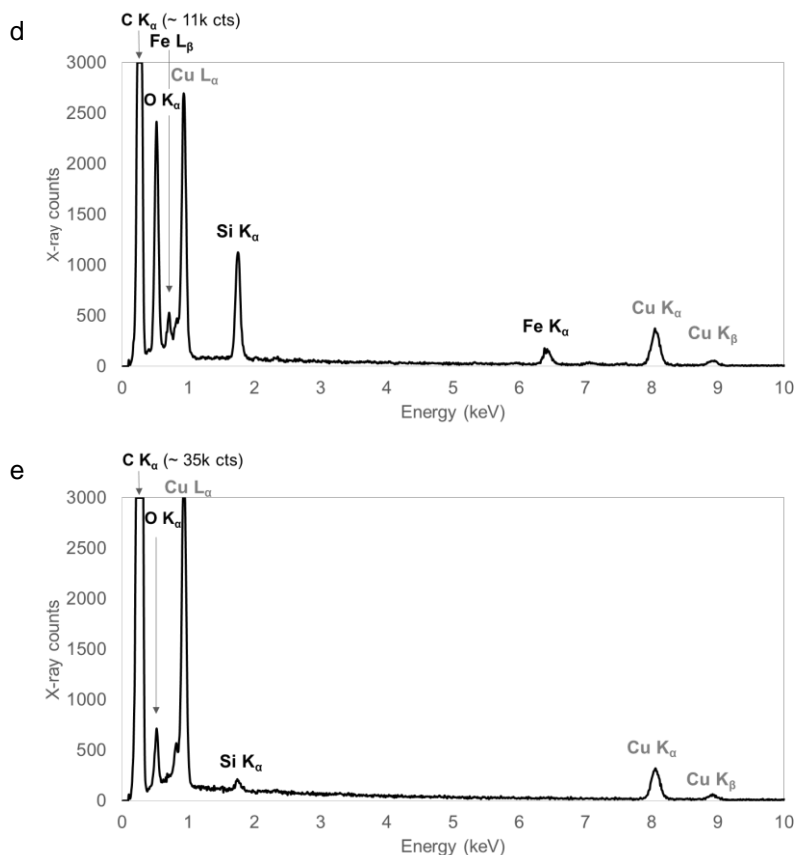
Figure 2: TEM bright field image (a) of a typical refractory carbonaceous particle from sample H (19.1 km altitude). The image is representative for all refractory carbonaceous particles. The morphology is not depending on chemical composition, size, morphology or nanostructure. Energy-dispersive X-ray spectra of (b) a typical refractory carbonaceous particle with Fe, Cr and Ni, (c) Fe and Cr, (d) Fe and (e) without any other minor constitute. The particle predominantly consists of C and O. Minor amounts of Si are always present and may partly be an artifact of the substrate. Cu is an artifact from the TEM grid. K α and K β as well as L α and L β denote different X-ray peaks emitted from the same element.
