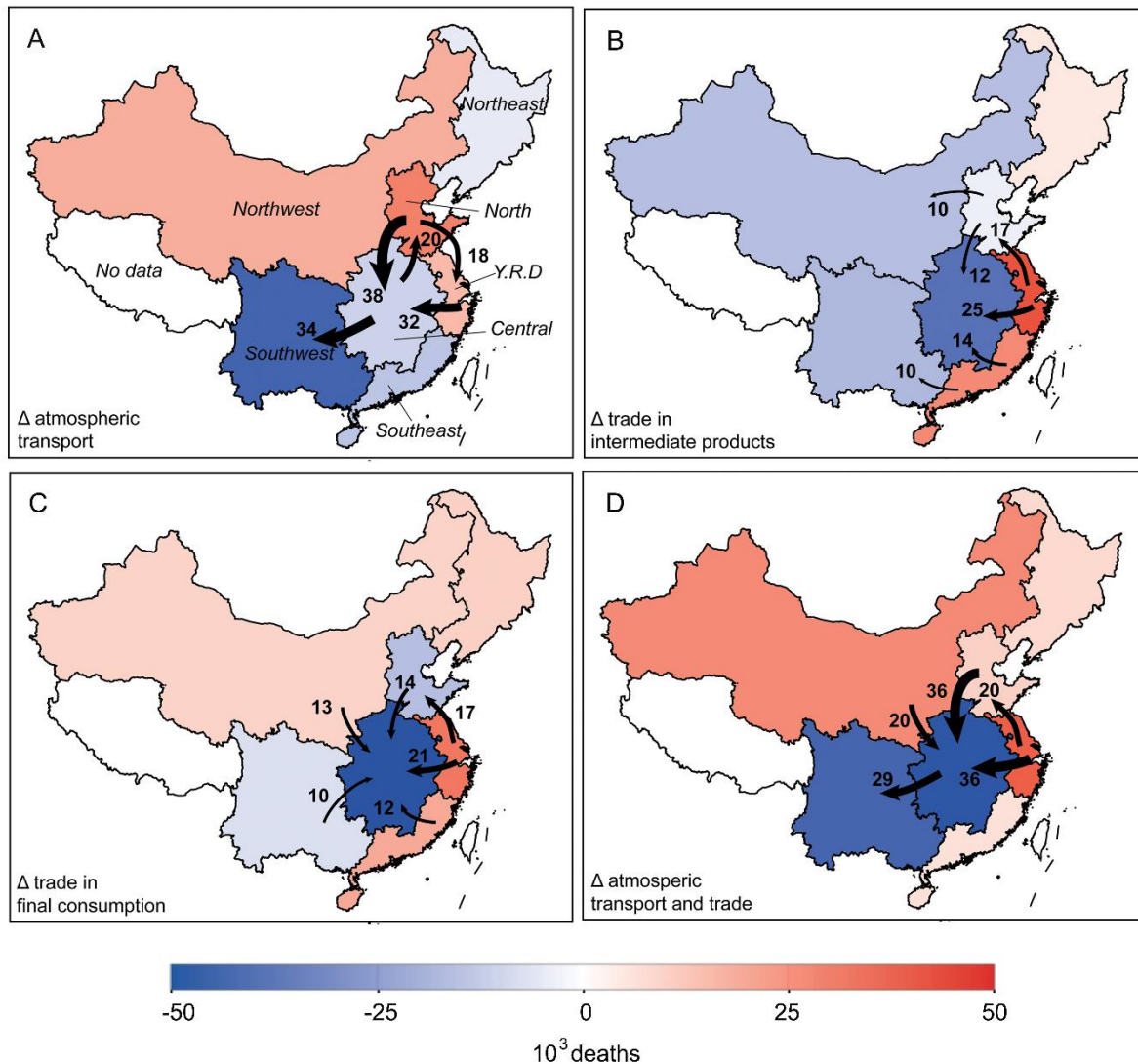
Figure 3. The effect of atmospheric transport (A) and trade (B-D) on each region's PM 2.5 -related premature deaths. Panel A compares the number of premature mortality related to emissions produced in each region and deaths that occurred in that region. Panel B and C compare regional production related premature deaths with deaths related to production of final goods in that region, and deaths related to consumption of goods and services in that region, respectively. Panel D compares the number of premature deaths occurred in each region with deaths related to consumption of goods and services in that region. Deaths in other regions due to Chinese pollution and deaths due to emissions in other nations are not included in any of the maps, and international export on regional premature deaths are not included in map C and D. Arrows between regions denote the largest interregional transfers, with numbers of displaced premature deaths shown in thousands.
