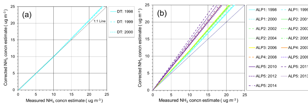
15 Figure 2: Comparison of annual empirical calibration curves for the passive samplers against the reference estimates from DELTA sampling at > 8 sites in the UK National Ammonia Monitoring Network (NAMN). (a) DT = Diffusion Tubes. (b) ALP = ALPHA samplers, ALP1 is prototype 1 (1998-2000), ALP2 (2001-2005) and ALP3-ALP5 were manufactured from injection moulds 1 and 2, respectively. ALP4 and ALP 5 = new inlet PTFE membrane (Swiftlab 07-OPM-027: 305 \mu\text{m} , regular polypropylene grid support material) that replaced the previous TE38 PTFE membrane ( 265 \mu\text{m} , randomly arranged polypropylene support material). ALP5 = new laboratory with analysis on FloRRia (previously on AMFIA).
