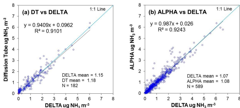
Figure 3: Regression of passive samplers vs DELTA measurements at >8 sites in the UK National Ammonia Monitoring Network (NAMN), showing results for (a) diffusion tubes (DT), used during the early years of the network (1998-2000), and (b) ALPHA samplers (results shown are for 2009-2014 where all analyses were carried out at a new laboratory). All passive data shown are the monthly measured concentrations for each site using the calibrated data for the respective passive methods.
