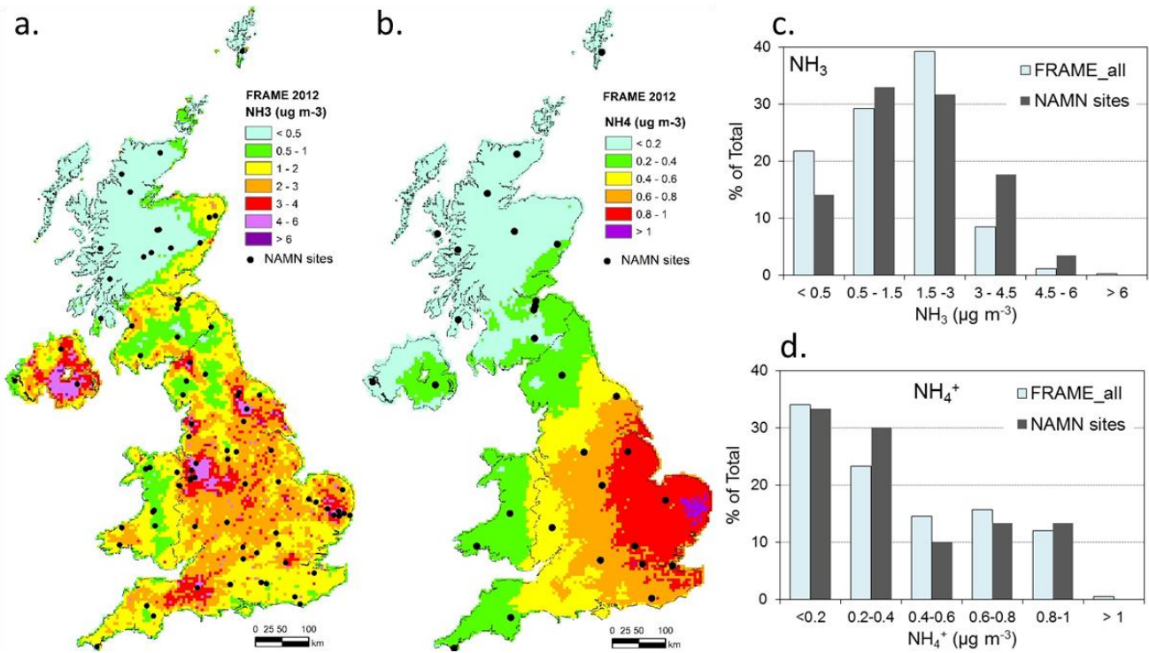
5 Figure 1: Maps of modelled annual mean concentrations of (a) \text{NH}_3 and (b) \text{NH}_4^+ at 5 km \times 5 km grid resolution from the FRAME atmospheric transport model using 2012 UK emissions data, based on Dore et al. (2008), overlaid with the National Ammonia Monitoring Network (NAMN) measurement sites, and frequency distributions of the modelled concentrations of (c) \text{NH}_3 and (d) \text{NH}_4^+ for the FRAME 5 km grid squares containing a NAMN site (85 and 30 sites, respectively, in 2012) and for all model grid squares over the UK.
