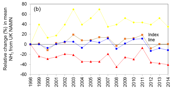
5 10 Figure 16: (a) Relative trends between 1998 and 2014 in NH 3 emissions from the UK National Atmospheric Emission Inventory (NAEI) for total emissions (all NH 3 sources) and emissions from cattle, pigs & poultry, and sheep separately (data from: http://naei.defra.gov.uk/ and Misselbrook et al, 2015). (b) Relative trends between 1998 and 2014 in measured annual mean NH 3 concentrations ( \mu\text{g NH}_3 \text{ m}^{-3} ) for all UK National Ammonia Monitoring Network (NAMN) sites, and for grouped sites classified as dominated by cattle, pigs & poultry, and sheep. Both figures are plotted with the same scale to allow direct comparison of the relative magnitudes in trends.
