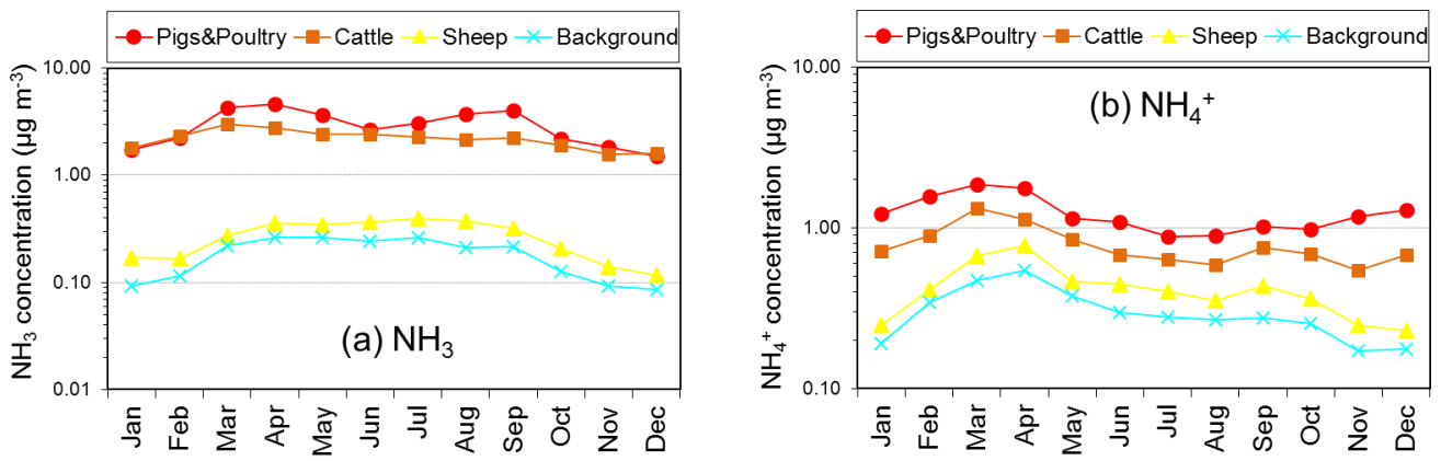
Figure 7: Seasonal trends in (a) \text{NH}_3 (mean monthly data for 1998-2014) and (b) \text{NH}_4^+ (mean monthly data for 1999-2014) concentrations of sites in the UK National Ammonia Monitoring Network (NAMN) classified according to four key emission source categories: cattle, sheep, pigs & poultry and background (based on 2005 dominant emission source classification). The concentrations are plotted on a log scale for better visualisation of the low concentration background and sheep profiles.
