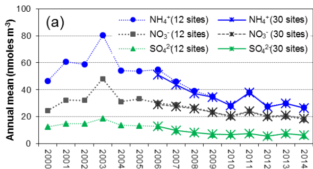
20 25 Figure 18: (a) Long-term trends in particulate NH 4 + from the UK National Ammonia Monitoring Network (NAMN) compared with particulate NO 3 - and SO 4 2- concentrations from the UK Acid Gas and Aerosol Network (AGANet; Connolly et al. 2016) measured at the same time. Each data point represents the averaged monthly measurements from all AGANet sites (increased from 12 to 30 sites since Jan 2006) and also the original 12 AGANet sites in the network (1999 data were excluded as measurements started in September 1999). (b) Trends in total UK emissions of NH 3 , NO x and SO 2 over the same period (2000-2014). Data from the National Atmospheric Emission Inventory (NAEI, http://naei.defra.gov.uk/ ).
