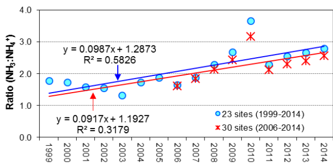
15 Figure 17: Long-term trends in ratio of NH 3 :NH 4 + , indicating an increase in this ratio with time. The comparisons shown is for datasets i) 23 sites with complete NH 4 + time series from 1999 to 2014, and ii) 30 sites with complete NH 4 + time series from 2006 to 2014.
