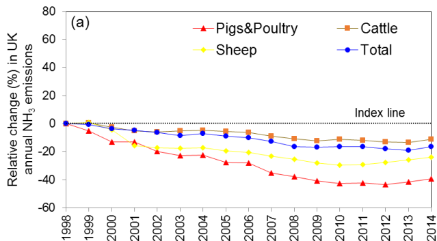
5 10 Figure 16: (a) Relative trends between 1998 and 2014 in NH 3 emissions from the UK National Atmospheric Emission Inventory (NAEI) for total emissions (all NH 3 sources) and emissions from cattle, pigs & poultry, and sheep separately (data from: http://naei.defra.gov.uk/ and Misselbrook et al, 2015). (b) Relative trends between 1998 and 2014 in measured annual mean NH 3 concentrations ( \mu\text{g NH}_3 \text{ m}^{-3} ) for all UK National Ammonia Monitoring Network (NAMN) sites, and for grouped sites classified as dominated by cattle, pigs & poultry, and sheep. Both figures are plotted with the same scale to allow direct comparison of the relative magnitudes in trends.
