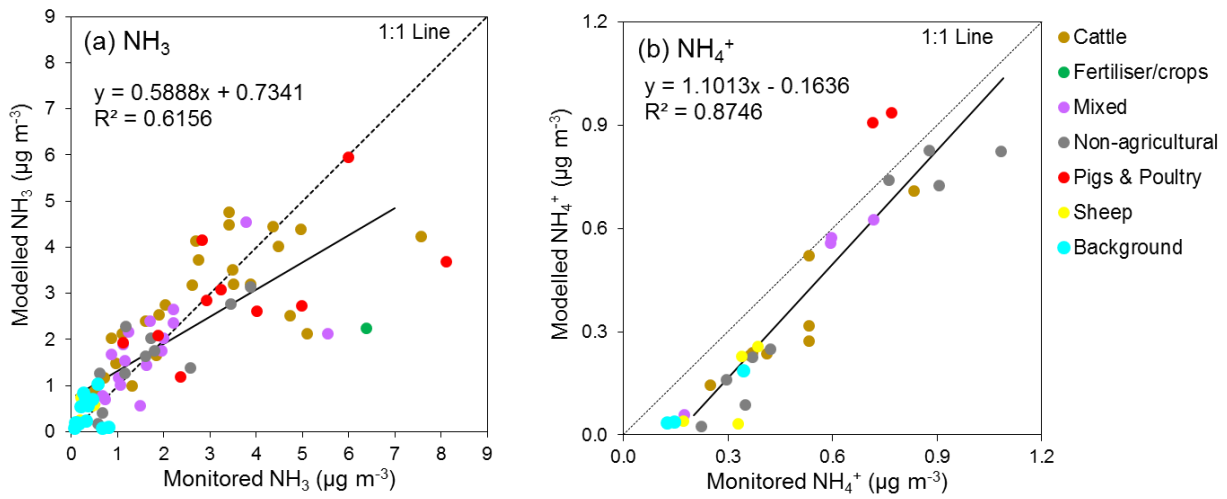
Figure 5: Comparison of 2012 annual mean concentrations of (a) \text{NH}_3 and (b) \text{NH}_4^+ modelled using the FRAME atmospheric model with 2012 measurements from the UK National Ammonia Monitoring Network (NAMN) for all sites according to dominant emission source classification.
