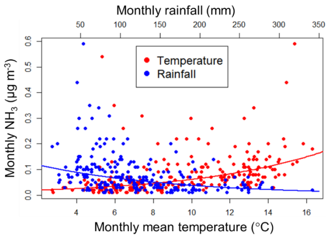
Figure 9. Relationships between measured monthly-mean \text{NH}_3 concentrations from the UK National Ammonia Monitoring Network (NAMN) and mean monthly temperature and rainfall at Inverpolly (UKA00457). \text{NH}_3 was negatively correlated with rainfall (blue line: \text{Log}(\text{NH}_3) = -0.0059 \cdot \text{Log}(\text{rain}) - 2.1612 , R^2 = 0.19 , n = 231 , p < 0.05 ) and positively correlated with temperature (red line: \text{Log}(\text{NH}_3) = 0.1482 \cdot \text{Log}(\text{temp}) - 4.2708 , R^2 = 0.33 , n = 231 , p < 0.05 ). Rain and temperature data are from the nearby Aultbea meteorological station (ID no. 52; MetOffice, 2016).
