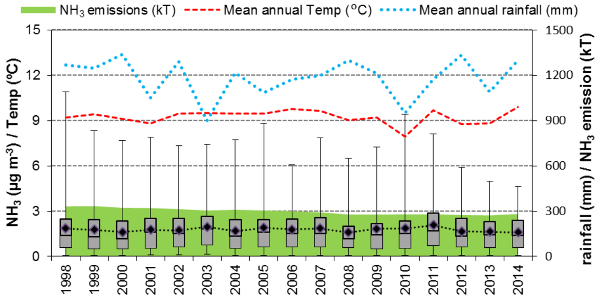
5 Figure 11: Changes in annual mean atmospheric NH 3 concentrations averaged over all sites in the National Ammonia Monitoring Network (NAMN) operational between 1998 and 2014 (59 sites). The diamonds show the mean NH 3 concentration, with the grey box indicating the median and interquartile range, while the error bars show the range (minimum and maximum) of measured mean concentrations. Annual mean UK meteorological data (source http://www.metoffice.gov.uk/ ) are also plotted for comparison over the same period. 2010 was an unusual year, characterised by a considerably lower than average mean annual temperature of 7.9 °C due to exceptionally cold winters, with Dec 2010 recorded as the coldest for over 100 years ( cf. mean = 9.2 °C for 1998 to 2014) and lower than average rainfall of 950 mm ( cf. mean = 1190 mm for 1998 to 2014).
