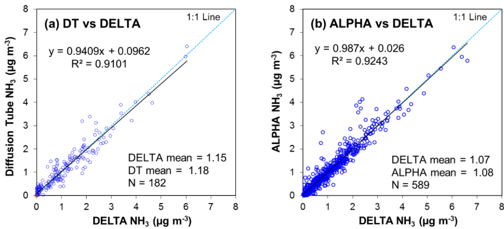
5 Figure 3: Regression of passive samplers vs DELTA measurements at >8 sites in the UK National Ammonia Monitoring Network (NAMN), showing results for (a) diffusion tubes (DT), used during the early years of the network (1998-2000), and (b) for ALPHA samplers (results shown are for 2009-2014 where all analyses were carried out at a new laboratory). All passive data shown are the monthly measured concentrations for each site using the calibrated data for the respective passive methods.
