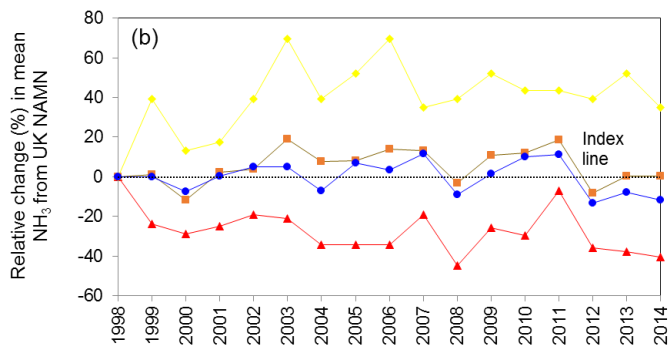
5 10 Figure 16: (a) Relative trends between 1998 and 2014 in NH 3 emissions from the UK National Atmospheric Emission Inventory (NAEI) for total emissions (all NH 3 sources) and emissions from cattle, pigs & poultry, and sheep separately (data from: http://naei.defra.gov.uk/ and Misselbrook et al, 2015). (b) Relative trends between 1998 and 2014 in measured annual mean NH 3 concentrations ( \mu\text{g NH}_3 \text{ m}^{-3} ) for all UK National Ammonia Monitoring Network (NAMN) sites, and for grouped sites classified as dominated by cattle, pigs & poultry, and sheep. Both figures are plotted with the same scale to allow direct comparison of the relative magnitudes in trends.
