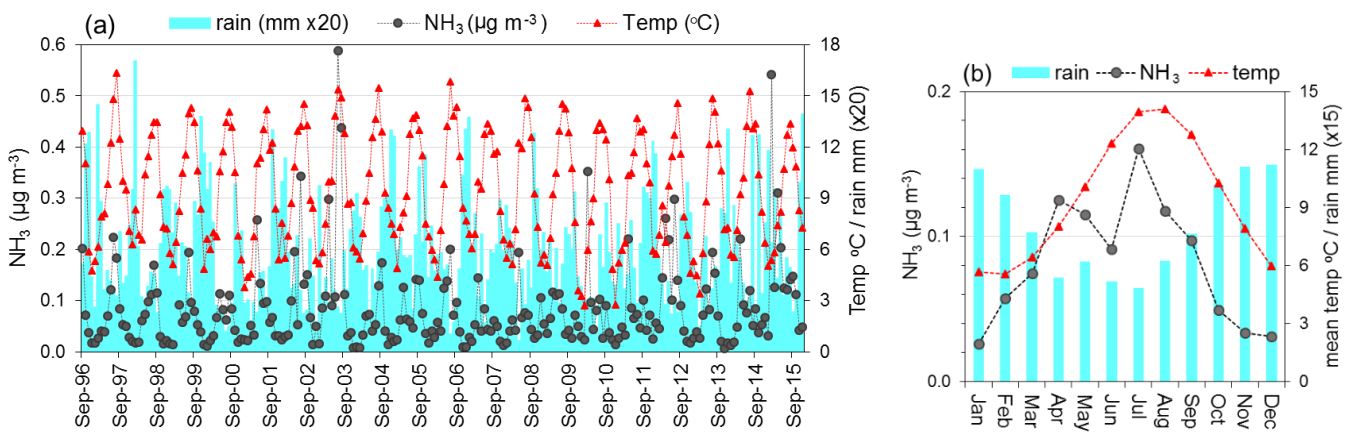
Figure 8: (a) Long-term trends in measured monthly-mean \text{NH}_3 concentrations at the remote background Inverpolly site in NW Scotland (UKA00457), demonstrating strong intra- and inter-annual variability, from the UK National Ammonia Monitoring Network (NAMN). Also plotted for comparison are monthly rainfall and temperature data from the nearby Aultbea meteorological station (ID no. 52; MetOffice, 2016). (b) Comparison of seasonal trends in \text{NH}_3 concentrations with temperature and rainfall at Inverpolly. Data shown are averaged over the period 1996 – 2015. Peak concentrations of \text{NH}_3 can be seen to coincide with summer maxima in the temperature profile, while the lowest concentration occur in winter when the temperature is lowest and also when rainfall is generally highest.
