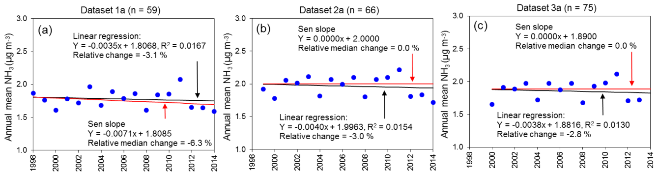
Figure 12: Time series trend analysis by non-parametric Mann-Kendall Sen slope vs parametric linear regression on annually averaged \text{NH}_3 concentrations from the UK National Ammonia Monitoring Network (NAMN) for a) dataset 1a (1998-2014, n=59 ), b) dataset 2a (1999-2014, n=66 ) and c) dataset 3a (2000-2014, n=75 ). Individual data points are annually averaged \text{NH}_3 concentrations.
