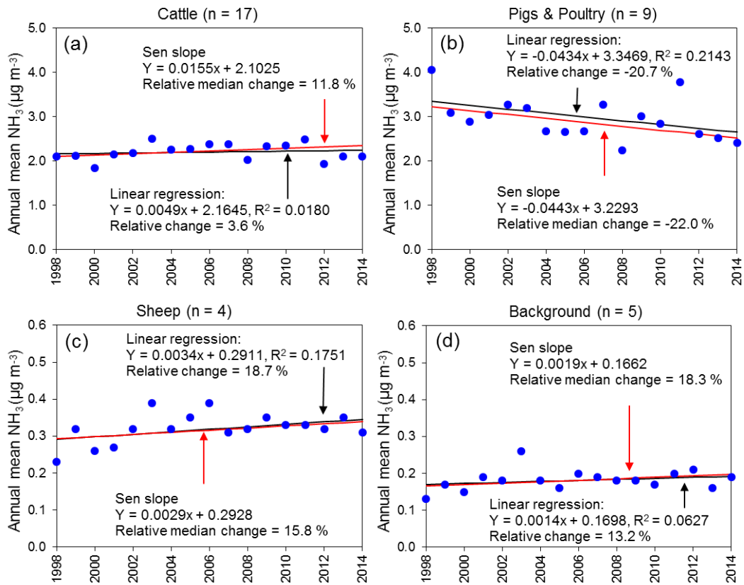
5 Figure 14: Time series trend analysis by non-parametric Mann-Kendall Sen slope vs parametric linear regression on annually averaged \text{NH}_3 concentrations from the UK National Ammonia Monitoring Network (NAMN) for sites in 5 km grid squares classed as dominated by (a) cattle (> 45 % of total \text{NH}_3 emissions from this category in a grid square); (b) pigs & poultry (> 45 % of total \text{NH}_3 emissions from this category in a grid square); (c) sheep (> 45 % of total \text{NH}_3 emissions from sheep in a grid square); (d) NAMN sites in grid squares classed as background (defined as grid squares with average \text{NH}_3 emissions < 1 kg N ha -1 y -1 ). Individual data points are annually averaged \text{NH}_3 concentrations.
