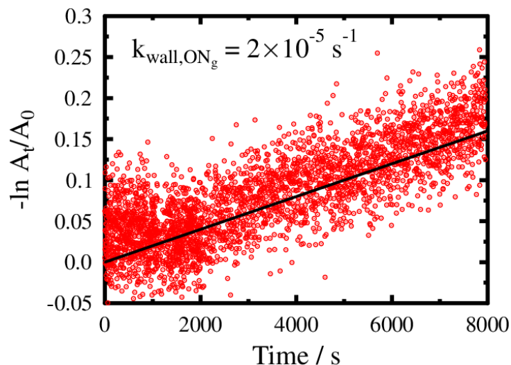
Figure S1. Wall loss rate of m/z 342 as measured by CIMS, corresponding to the monoterpene hydroxy nitrate- \Gamma adduct.
