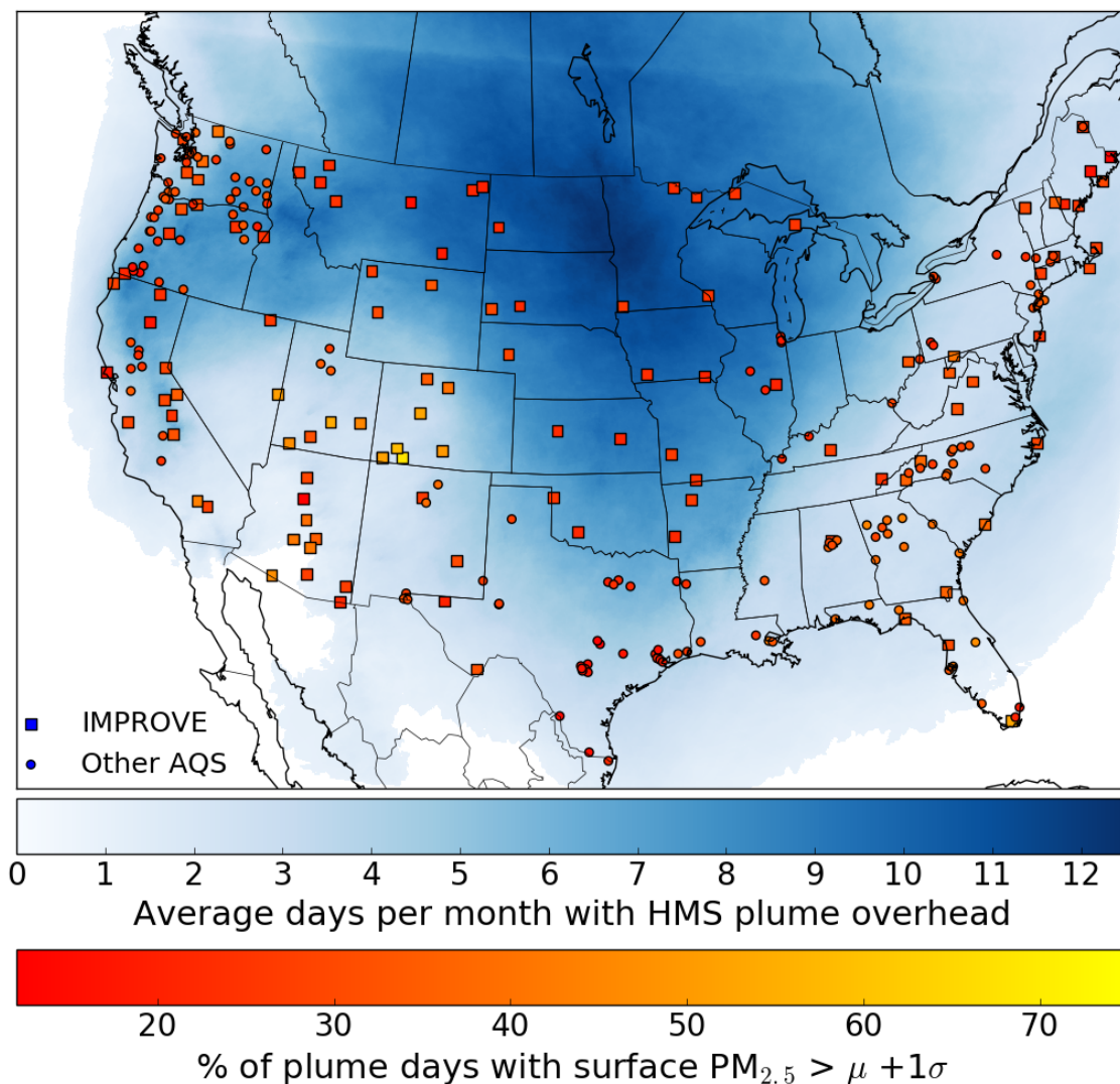
5 10 Figure 1: North American smoke climatology for June-September 2007-2014. Blue shading indicates the average days per month HMS smoke plumes are analyzed overhead. Markers show non FRM (Federal Reference Method) PM_{2.5} monitors shaded by the percent of plume days where surface 24-hr average PM_{2.5} is greater than the mean ( \mu ) plus one standard deviation ( \sigma ) value for the monitors mean value in June-September. Only monitors with data on 90% of days between June-September 2007-2014 are presented. IMPROVE monitors are marked by squares; all other monitors from the EPA Air Quality System (AQS) are marked by circles. IMPROVE monitors record data every third day. We make the assumption that smoke plumes are equally likely to occur on measurement days as non-measurement days, and thus multiply the number of ground level smoke-impacted plume days at IMPROVE sites by three. Monitors that fall within white areas are influenced by smoke < 1 day per month. The climatology presented here does not relate to smoke plume or ground level PM_{2.5} concentrations, only the presence of smoke in the column and proportion of those days when surface PM_{2.5} is elevated.
