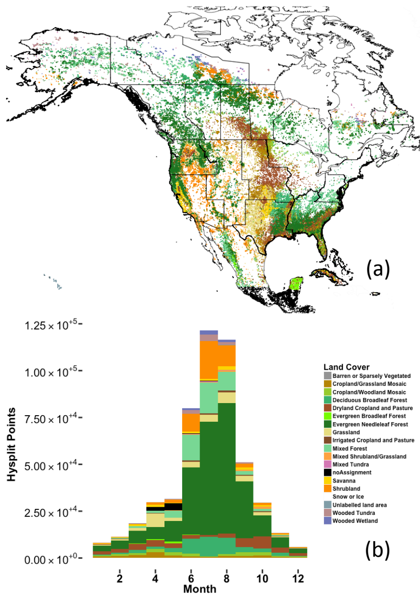
Figure 8: Location, (a) seasonality, (b) and land cover classification assignment (color) for all HYSPLIT points analyzed over North America between 2007-2014 (n=517,214). No land cover assignment is made for Southern Mexico (MX) and U.S. Islands
