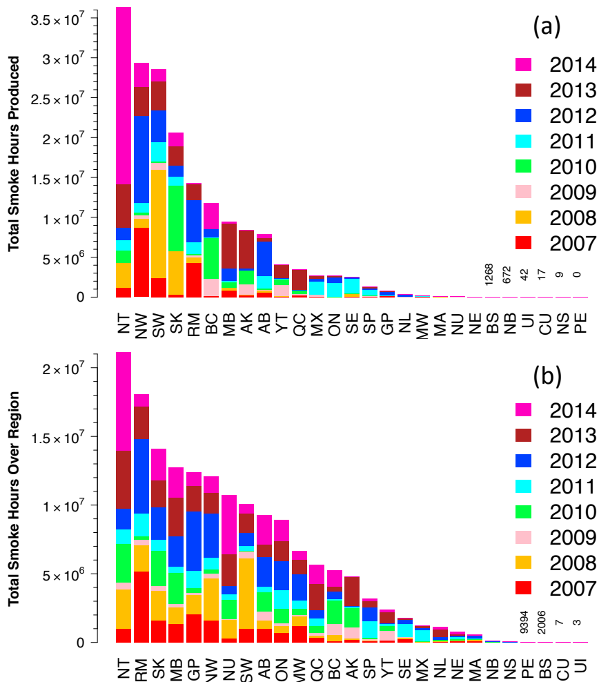
Figure 10: (a) Total number of smoke hours produced (anywhere) by each region for months June-September between 2007 and 2014 using GDAS1 meteorology. (b) Total number of smoke hours over each region for months June-September between 2007 and 2014 using GDAS1 meteorology.
