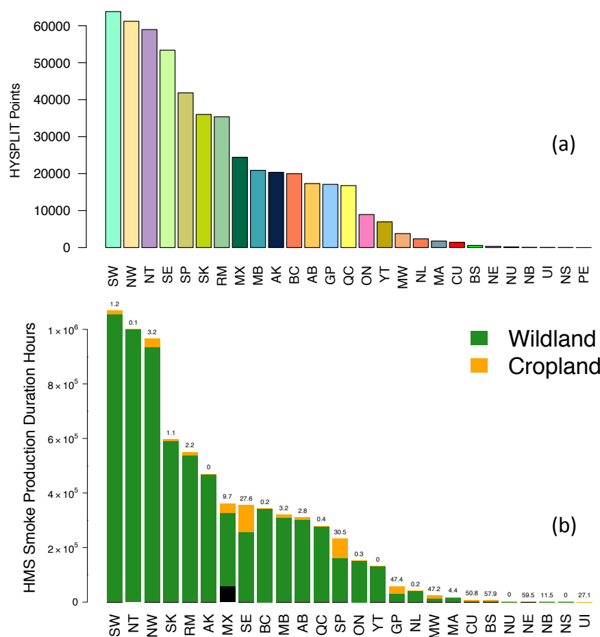
Figure 7: (a) Total HMS HYSPLIT point detections for all regions and months between 2007-2014. Region colors and abbreviations are defined in Fig. 6. (b) Total HMS smoke production duration hours (SPDH) for the same time period. The number on top of each bar indicates the percentage of SPDH that are from croplands. The black portion of Mexico (MX) represents fires that occurred on land outside of the land cover data extent used in this analysis.
