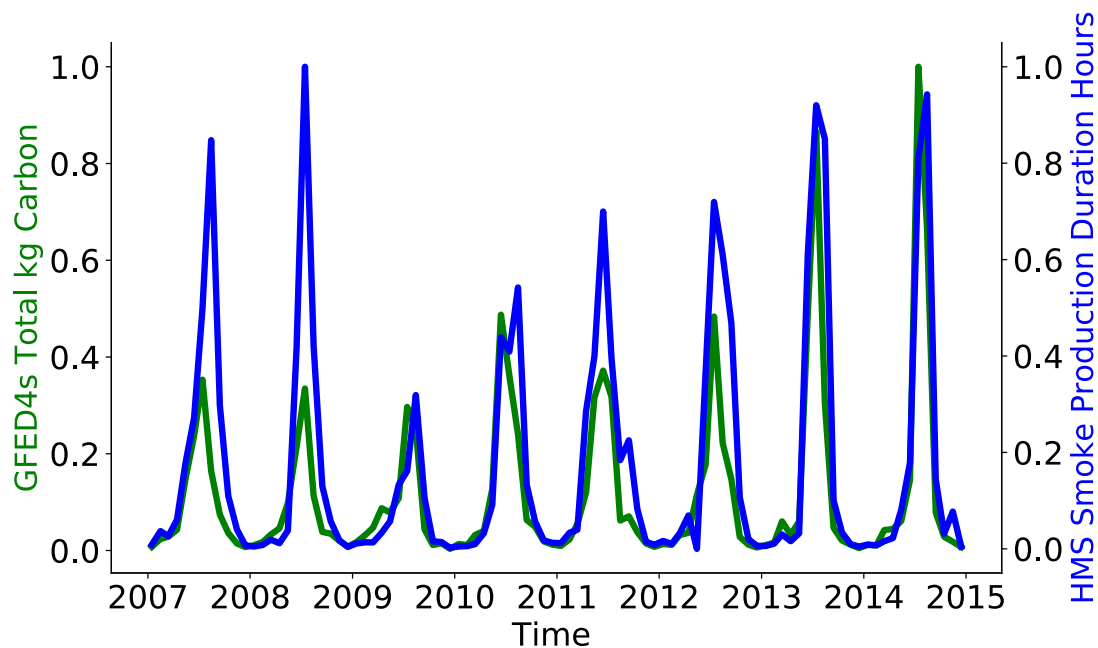
Figure 4: Time series of monthly domain ( 20-80^\circ \text{N} , 50-170^\circ \text{W} ) summed kg carbon (left axis) and HMS-hours (right axis). Monthly totals have been divided by the maximum monthly value observed between 2007-2014. The Pearson correlation coefficient for the presented monthly time series is 0.842.
