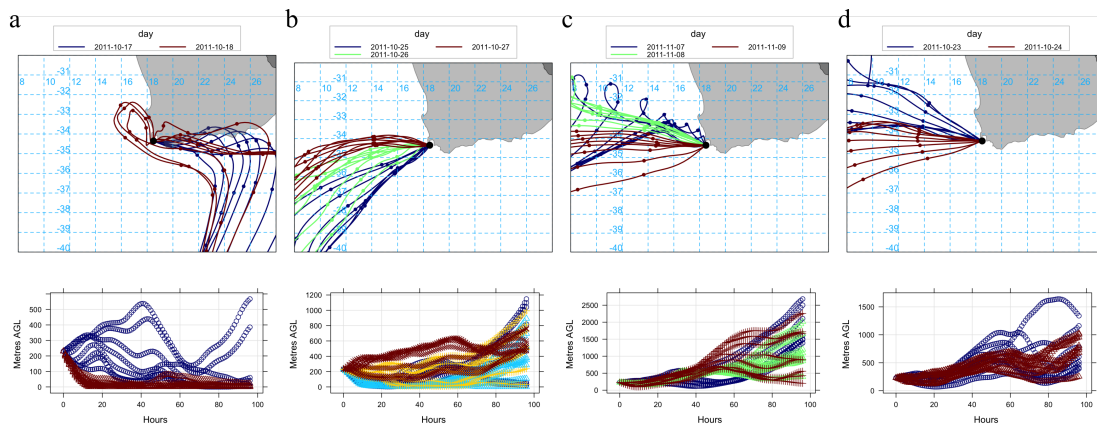
Fig. 5. Composite daily back trajectories for the selected Events (a) E1 17 – 18 October 2011, (b) E2 25 – 27 October 2011, (c), E3 7 – 9 November 2011, (d) Background samples 23 - 24 October 2011. Trajectory
