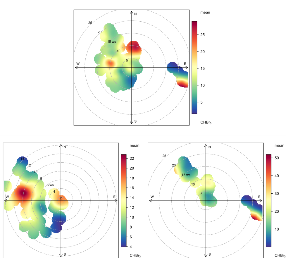
Fig. 3. Polar plots of bromoform as a function of wind speed and direction. The top figure highlights all the data, while the lower plots show background and non-background respectively. These figures give an
