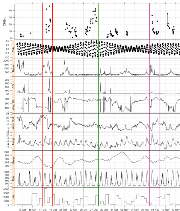
Fig. 1. Time series plot of measurements at Cape Point during October / November 2011. Events are highlighted by the coloured lines: E1 = red, E2 = green, E3 = violet.
