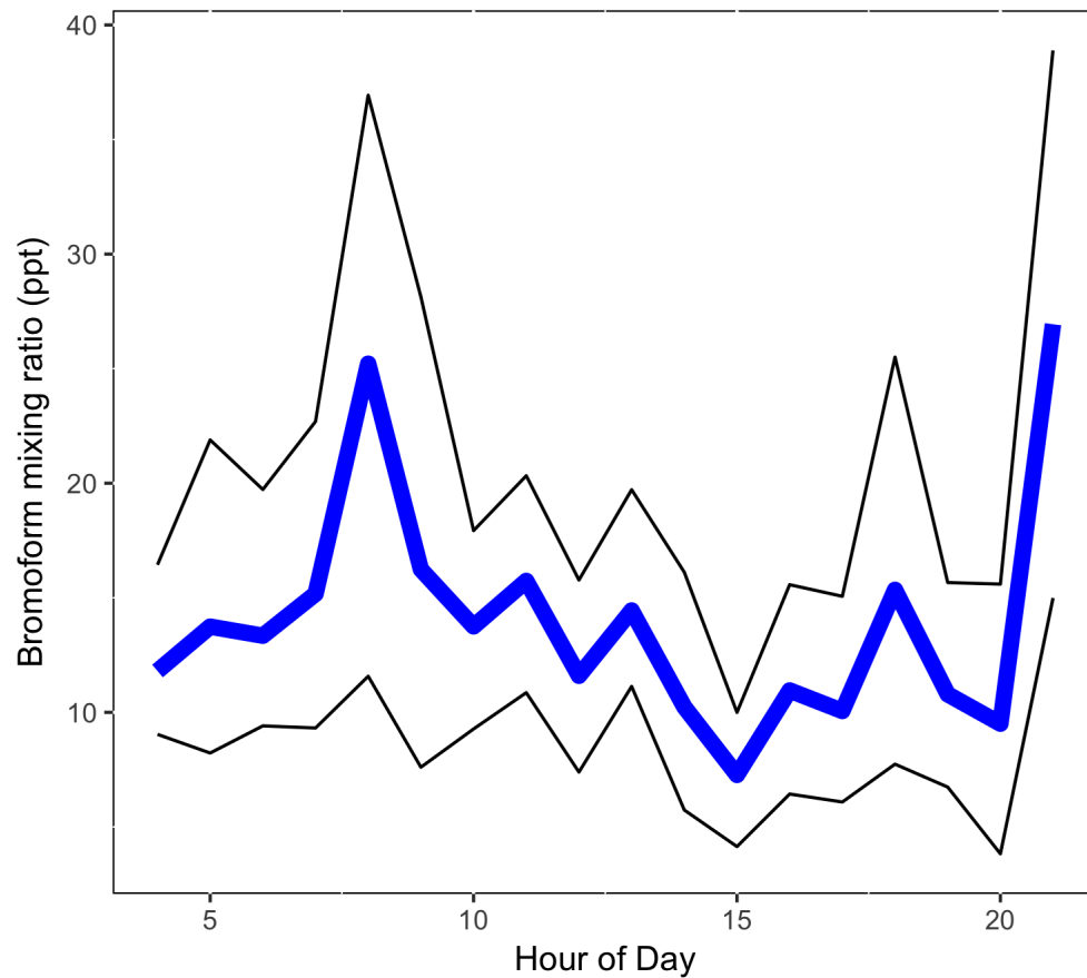
Fig. 2. Mean diurnal cycle, calculated from all measurements binned by hour. The black lines above and below signify the 95 % confidence interval.
