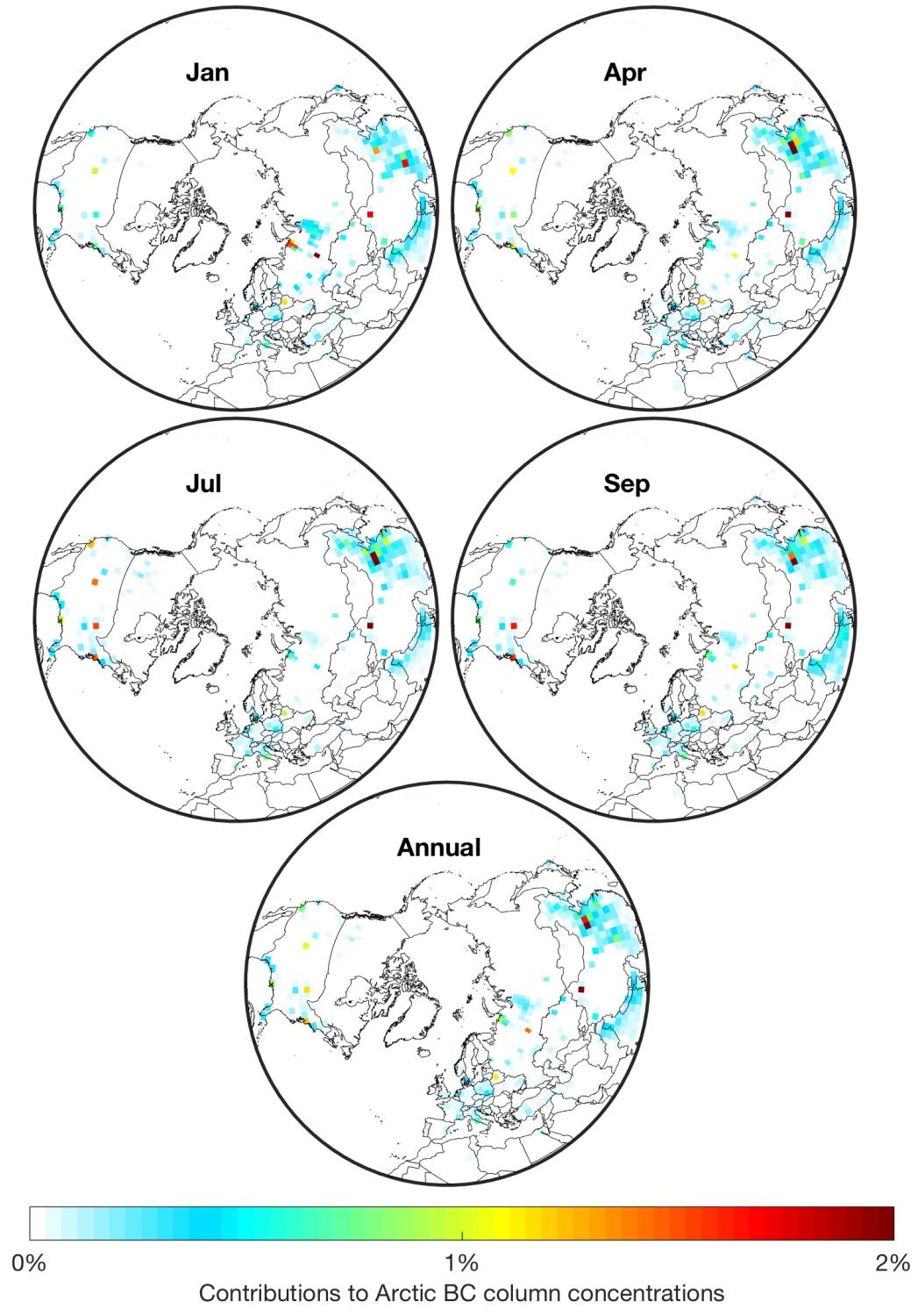
Figure 9. Contributions to Arctic BC column concentrations from changes in local emissions (as percent change in Arctic BC column concentration per fractional change in emissions) in 2011. Local
