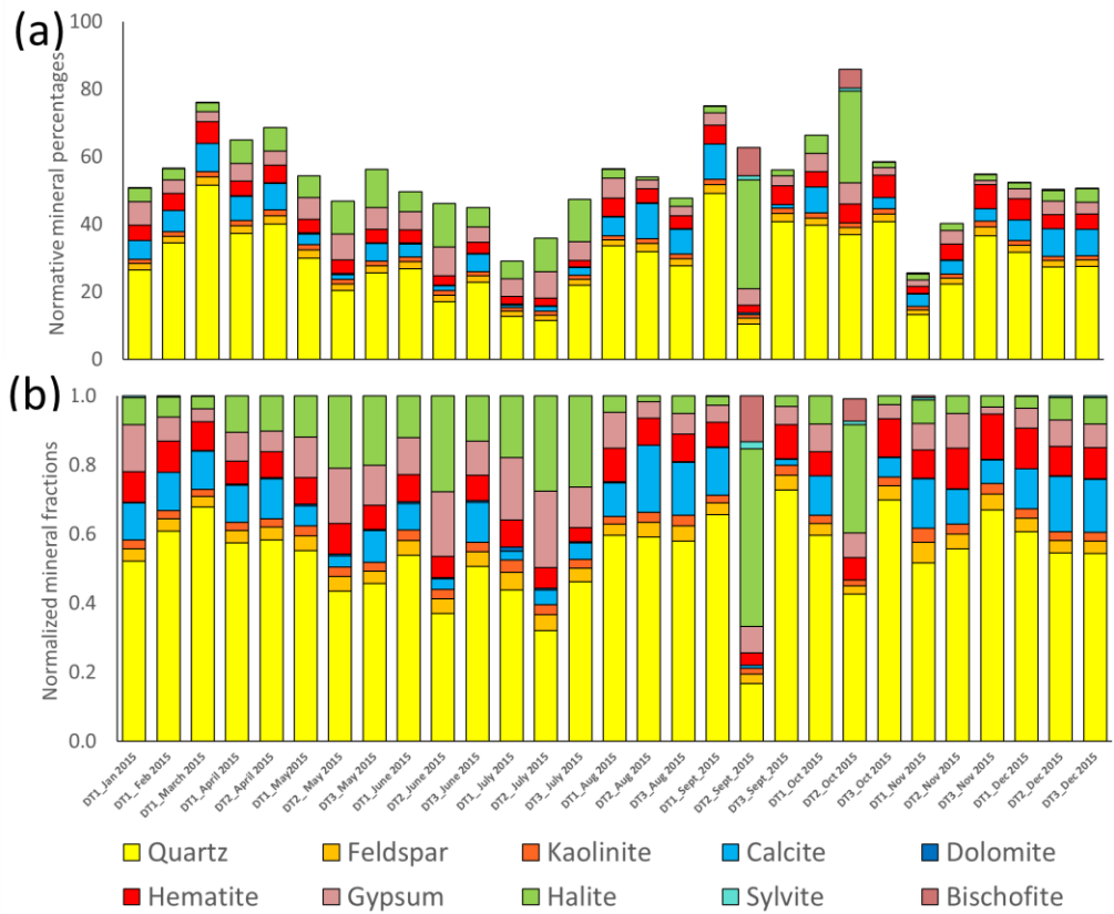
Figure 11 (a). Chemical abundances combined as normative minerals, (b) normalized to 100 %.
