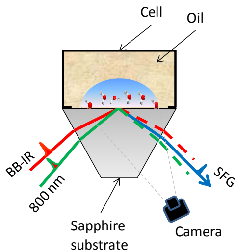
Figure 1. Schematic of the sample setup used in the SFG experiments. The SFG signal is generated in a co-propagating total internal reflection geometry at the spatial and temporal overlap of the incoming visible (800nm) and infrared (BB-IR) light. The camera is used to observe the droplet while placing it on the surface and filling the cell with oil, and to observe its status during the experiment.
