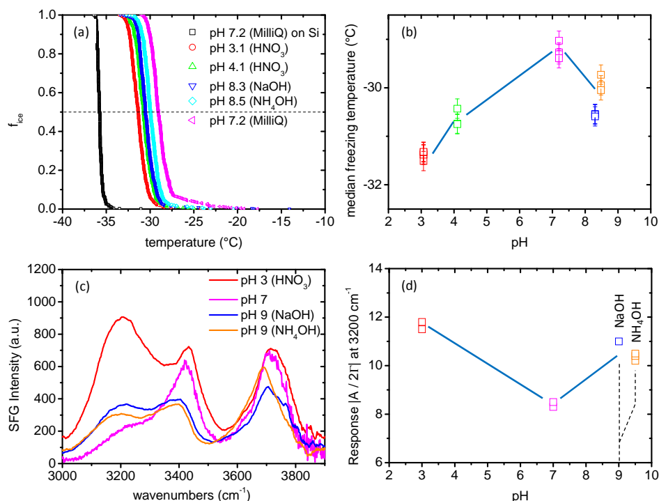
Figure 2. (a) Fraction of frozen droplets as a function of temperature of Sapphire (0001) surface in contact with different pH solutions. The black curve shows the data for water on a silicon substrate. (b) Freezing temperature as a function of pH of the different solutions for three independent experiments. (c) SFG spectra of liquid water at the Sapphire (0001) surface, right before the nucleation event (see text for details); for fits, see Fig. 3. (d) Absolute value of the amplitude divided by width as a function of pH for the 3200 cm -1 resonance inferred from the data shown in (c). Different data points indicate data obtained from freshly prepared surfaces, recorded on different runs.
