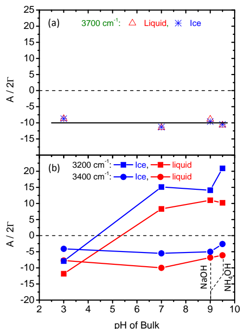
Figure 4. Amplitudes of indicated resonances divided by their width as a function of pH for (a) the 3700 cm -1 resonance and (b) the 3200 and 3400 cm -1 resonances, all three inferred from Lorentzian fits to the spectra of Fig. 3. low and high pH, may restrict the freedom of the interfacial molecules to structure themselves in the ice crystal.
