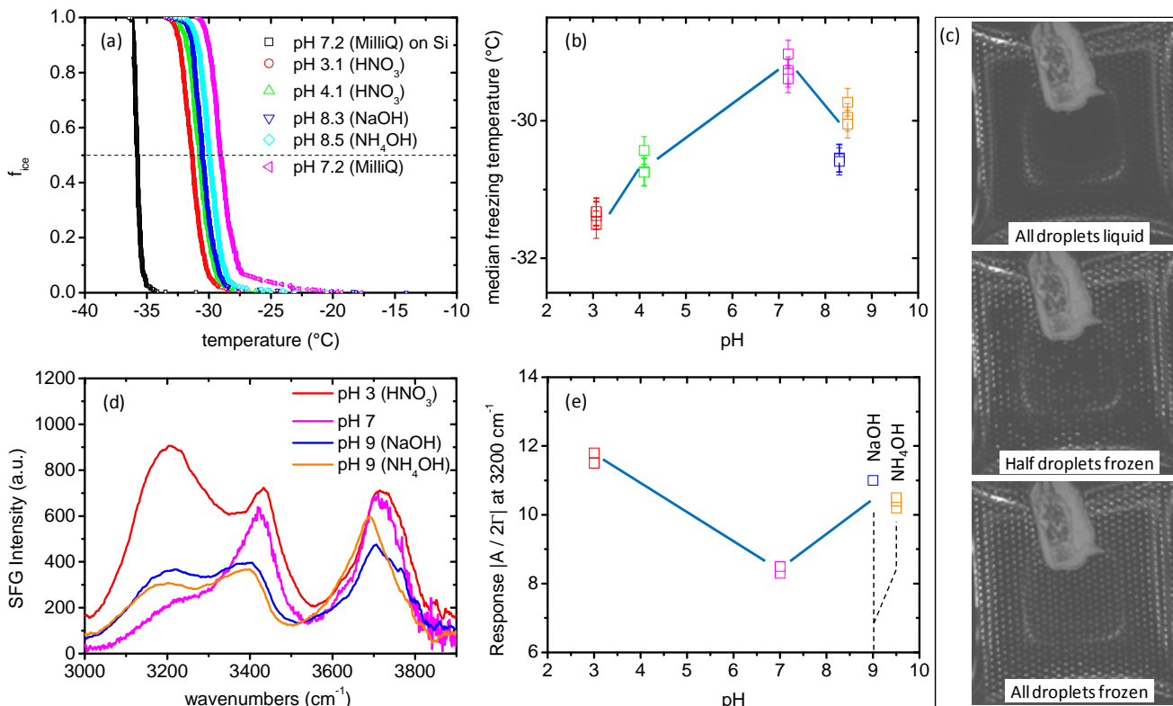
10 Figure 2. (a) Fraction of frozen droplets as a function of temperature of Sapphire (0001) surface in contact with different pH solutions. The black curve shows the data for water on a silicon substrate. (b) Freezing temperature as a function of pH of the different solutions for three independent experiments. (c) Images of typical droplets on the substrate at different stages of the droplet freezing assay experiment. (d) SFG spectra of liquid water at the Sapphire (0001) surface, right before the nucleation event (see text for details); for fits, see Fig. 3. (e) Absolute value of the amplitude divided by width as a function of pH for the 3200 cm -1 resonance inferred from the data shown in (d). Different data points indicate data obtained from freshly prepared surfaces, recorded on different runs. 15
