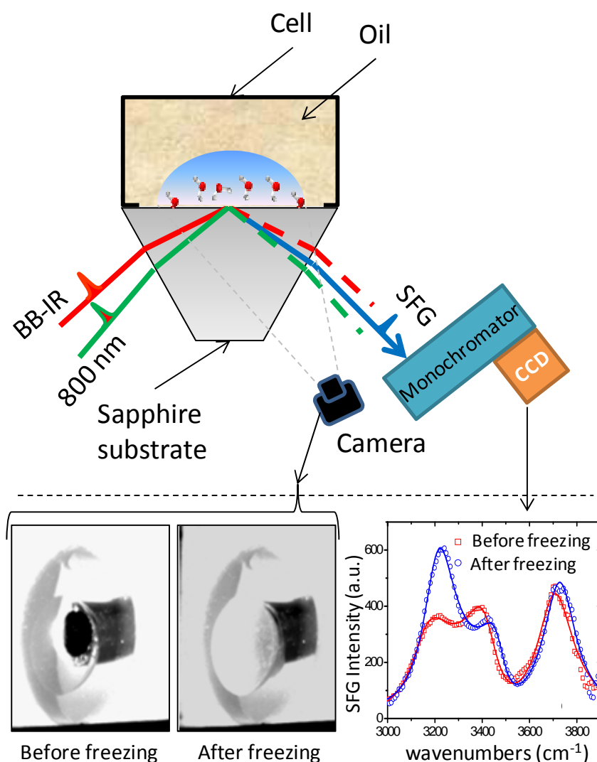
15 Figure 1. Upper panel: Schematic of the sample setup used in the SFG experiments. The SFG signal is generated in a co-propagating total internal reflection geometry at the spatial and temporal overlap of the incoming visible (800nm) and infrared (BB-IR) light, focused down to a \sim 100\ \mu\text{m} diameter spot size. The camera (Guppy F-036 Allied Vision Technology with LINOS Macro-CCD Lens 0.14x (1:7) f4) is used to observe the droplet while placing it on the surface and filling the cell with oil, and to observe its status during the experiment. Lower panel left: images of a typical drop on the substrate before and after freezing. Lower panel right: Typical water spectra before and after the freezing.
