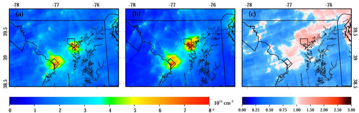
Figure 10. Oversampled tropospheric column \text{NO}_2 at 1.33 km in the Baltimore-Washington metropolitan area for June & July 2011 only. (a) OMI_CMAQ_OD. (b) CMAQ \text{NO}_2 corresponding to valid overpass times. (c) Ratio between the two plots CMAQ / OMI_CMAQ_OD.
