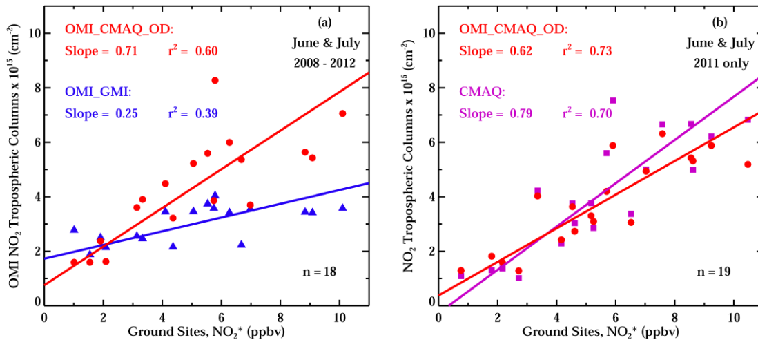
Figure 9. (a) Tropospheric column \text{NO}_2 OMI_GMI and OMI_CMAQ_OD versus co-located ground \text{NO}_2^* chemiluminescence measurements within \pm 2 hours of a valid satellite overpass during June & July 2008 through 2012; all \sim 300 daily ground monitor values are merged into a mean single value and compared to the satellite mean over the same corresponding time period. (b) Same as (a) but now comparing CMAQ and OMI_CMAQ_OD for June & July 2011 only.
