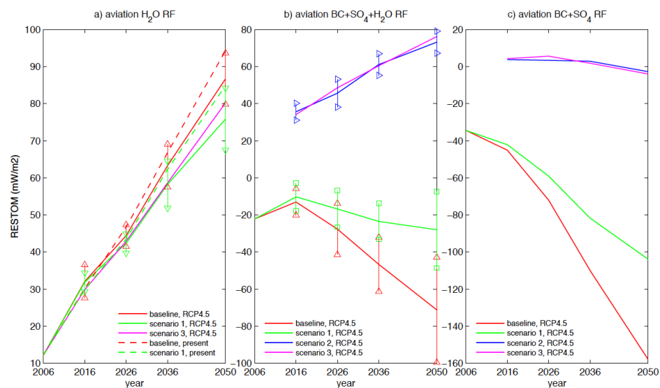
Figure 1: Radiative forcing in CESM from (A) H 2 O emissions alone (contrail cirrus), (B) H 2 O + BC + SO 4 emissions and (C) The residual effect of BC and SO 4 estimated from (B) – (A). Solid lines are for the RCP 4.5 scenario with different meteorology each year; dashed lines in panel (A) are using 2006 meteorology. Since scenario 1 and scenario 2 have the same H 2 O emissions, they have the same RF in (A). The baseline aviation scenario is in red, scenario 1 is green, scenario 2 is blue and scenario 3 is purple.
