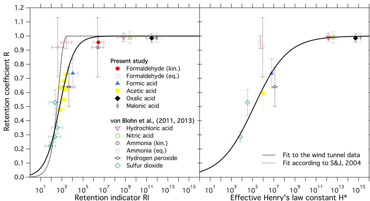
Figure 3. (a): Retention coefficient as function of retention indicator. Filled symbols: organic substances of the present study. Open symbols: wind tunnel data from earlier studies (von Blohn et al., 2011, 2013). The fine lined symbols for formaldehyde and ammonia represent values for equilibrium conditions neglecting the aqueous phase kinetics (see text). Vertical error bars are measurement uncertainties. Horizontal error bars account for the two limits of adiabatic freezing time and total freezing time of the droplets. Dotted line: fit according to Stuart and Jacobson (Stuart and Jacobson, 2004). Solid line: new fit of the wind tunnel data. (b): Retention coefficients as function of H^* . Symbols according to (a). Solid line: new fit of the wind tunnel data. The H^* values are calculated from literature (see Table 4) at given pH and at 0^\circ\text{C} .
