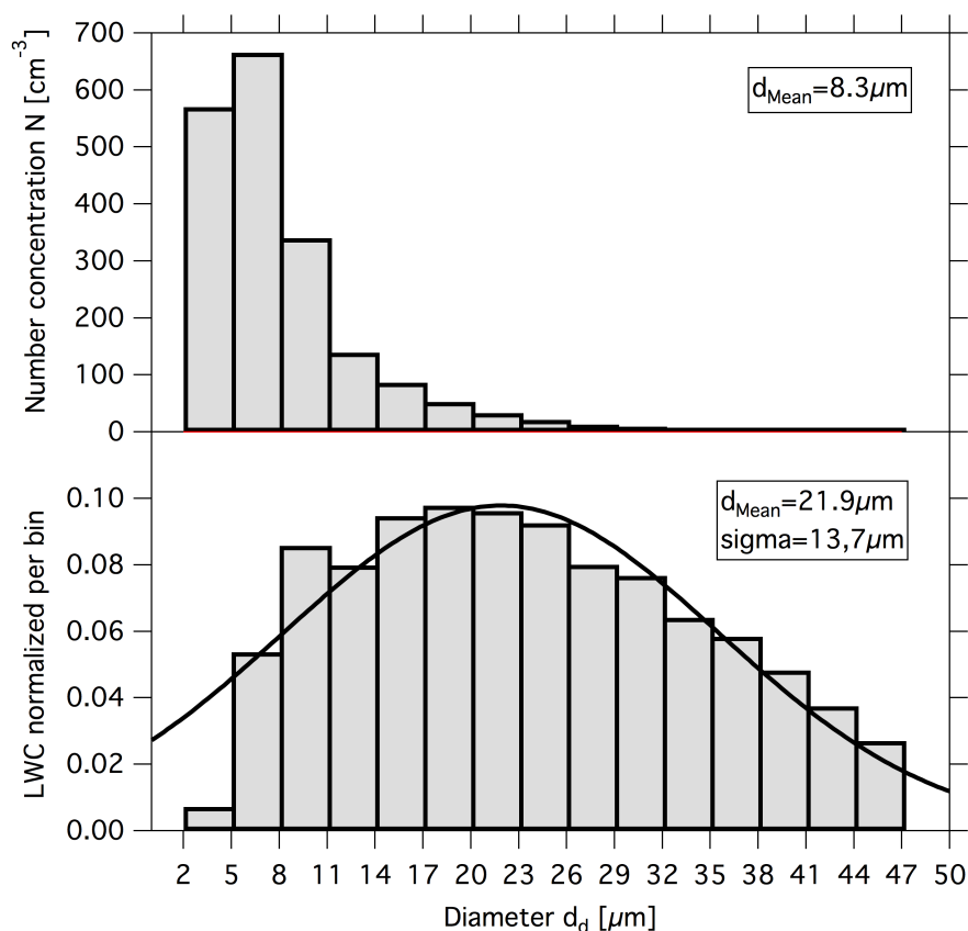
Figure 1. Droplet number (upper panel) and mass (lower panel) distribution of the supercooled cloud generated in the wind tunnel. The average error due to count statistics is 23%.
