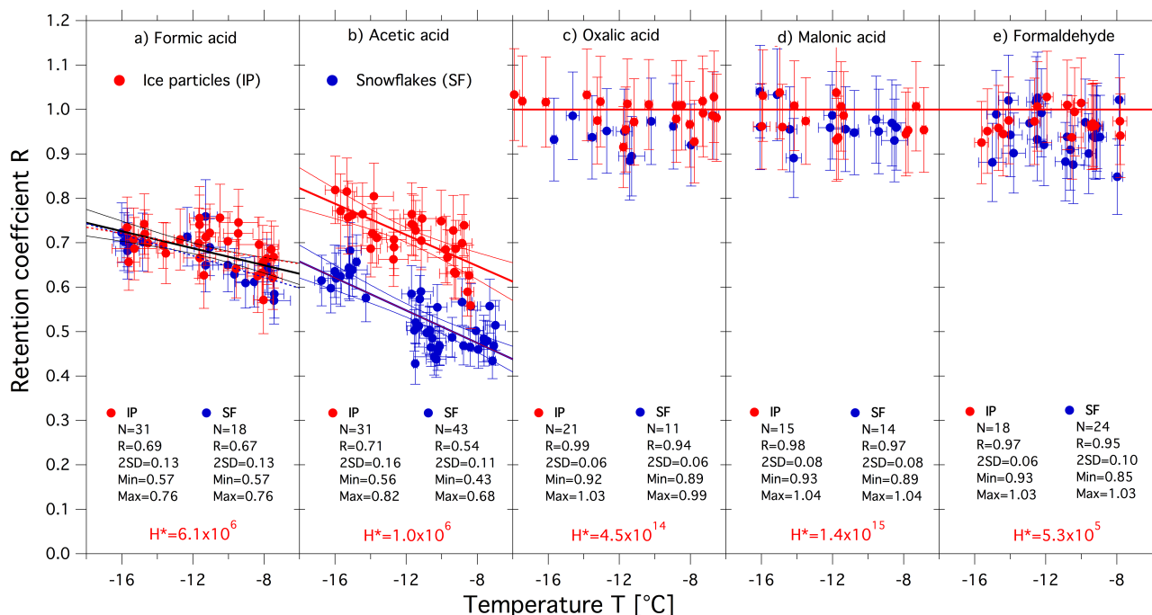
Figure 2. Retention coefficients of all measured substances as function of temperature for different rime collectors. Red symbols: rimed ice particles. Blue symbols: rimed snowflakes.
