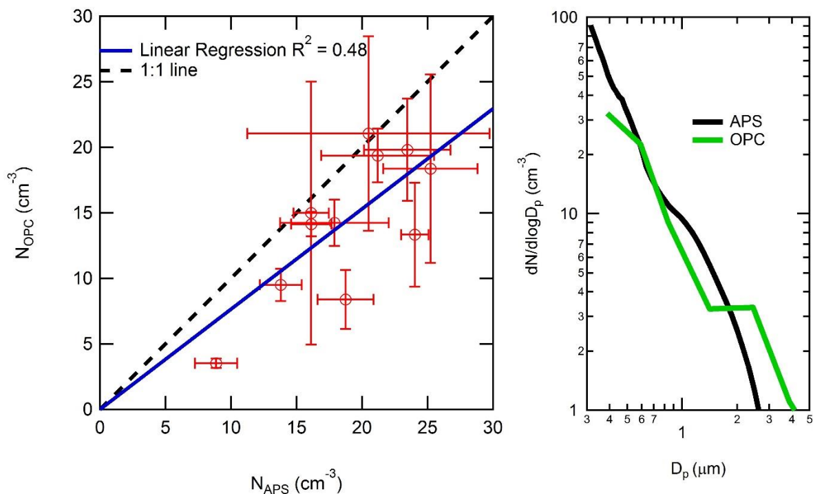
Figure 2. OPC concentrations with particle diameters ( D_p ) greater than 0.3 \mu\text{m} (left) from 11 UAV research flights, listed in Table 1, plotted against APS concentrations ( D_p > 0.3 \mu\text{m} ) at Mace Head Research Station (red circles). Error bars represent \pm 1 standard deviation. The points are fit with a linear regression (blue line). OPC data was averaged between 40 and 80 m asl. Averaged OPC and APS number size distributions averaged for the 11 flights (right).
