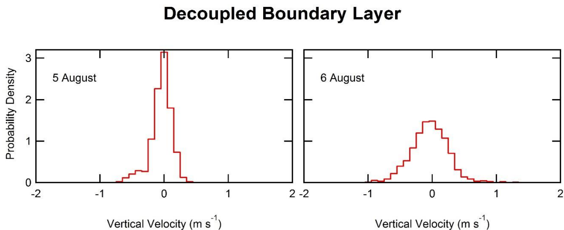
805 Figure 3. Normalized observed vertical velocity distributions measured by the cloud radar and UAV for each case presented in Table 2.
