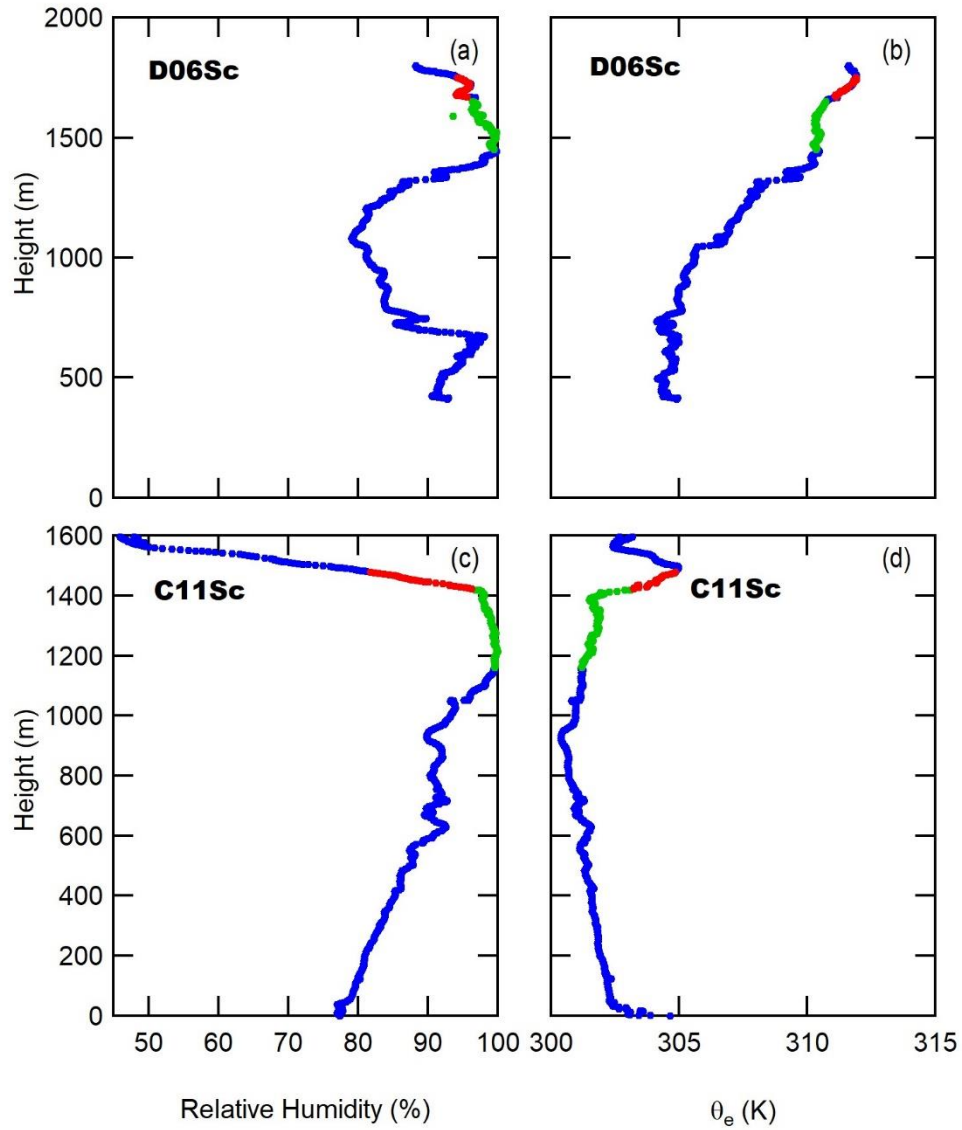
Figure 11. UAV vertical profiles of relative humidity (a, c) and \theta_e (b, d) for flights D06Sc and C11Sc, used in Figure 10. Profiles are defined as cloud-free (blue), in-cloud (green) or entrained air sources (red).
