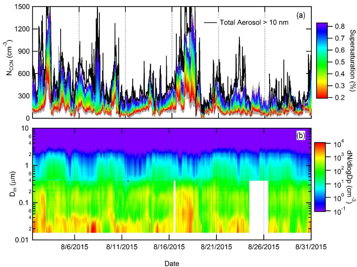
Figure 1. Time series for the month of August 2015 at Mace Head Ireland of ground-based CCN concentrations (top) and merged SMPS and APS number size distributions (bottom).
