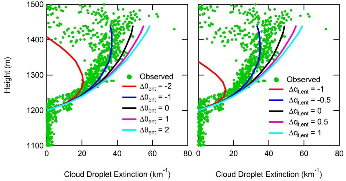
Figure 12. Sensitivity of simulated cloud extinction based on variability of entrained air potential temperature ( \theta_{\text{ent}} , K) and entrained air total water mixing ratio ( q_{\text{t,ent}} , \text{g kg}^{-1} ) for the C11Sc case. The \Delta\theta_{\text{ent}} and \Delta q_{\text{t,ent}} terms define the change in the entrained \theta and q_{\text{t}} values where no change ( \Delta\theta_{\text{ent}} = 0 and \Delta q_{\text{t,ent}} = 0 ) is equivalent to the adiabatic simulation with entrainment from Figure 8c.
