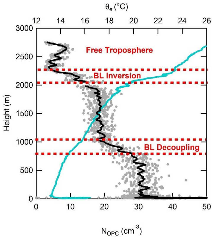
Figure 9. Flight 10 UAV vertical profile of OPC aerosol number concentrations ( D_p > 0.3 \mu m ) (grey) with a 20 second running mean (black) and equivalent potential temperature ( \theta_e , light blue) illustrate decoupling of the boundary layer. In-cloud OPC measurements (2000 m- 2050 m) have been removed.
