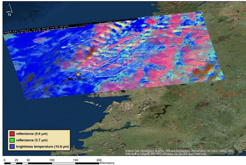
805 Figure 4. Suomi NPP satellite RGB composite image for 21 August 2015 (left). Mace Head Research Station and UAV flight location are indicated by the yellow star. The white polygon represents the zone for retrieving cloud properties – which is represented by the profile of cloud effective radius (right). Effective radius profiles are presented for both the Suomi NPP satellite (red) and the ACPM (blue).
