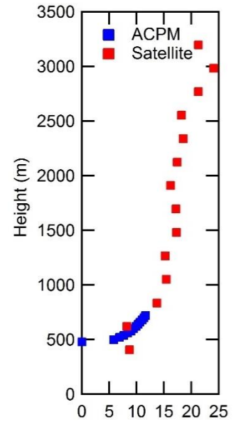
805 Figure 4. Suomi NPP satellite RGB composite image for 21 August 2015 (left). Mace Head Research Station and UAV flight location are indicated by the yellow star. The white polygon represents the zone for retrieving cloud properties – which is represented by the profile of cloud effective radius (right). Effective radius profiles are presented for both the Suomi NPP satellite (red) and the ACPM (blue).
