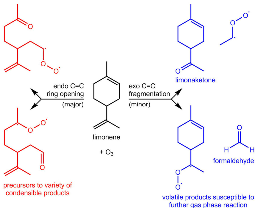
5 Figure 1: Initial products of limonene ozonolysis following reaction with the cyclic endo C=C (red channel) and terminal exo C=C (blue channel). The Criegee intermediates produced in these reactions can proceed to form a variety of multifunctional products observed both in the gas and particle phases.
