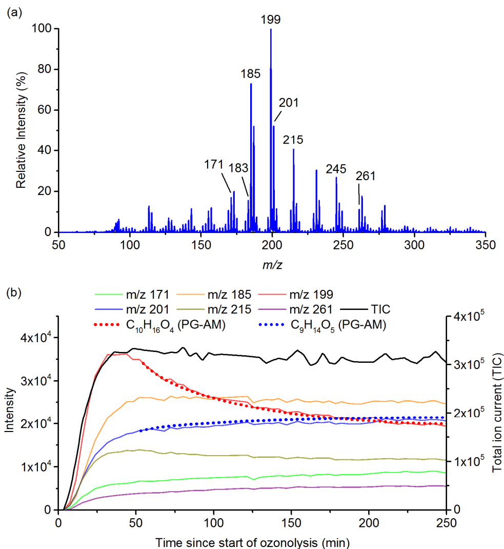
Figure 5: (a) EESI mass spectrum after 50 minutes. Some major peaks discussed in the text are labeled with their m/z . (b) Wall-loss corrected intensities for selected particle-phase ions detected using EESI-MS during limonene SOA formation. The total ion current (TIC) across the entire MS is shown on the secondary y-axis. The dotted lines are a PG-AM simulation for the reaction of C_{10}H_{16}O_4 with ozone to form C_9H_{14}O_5 , assuming semisolid SOA.
