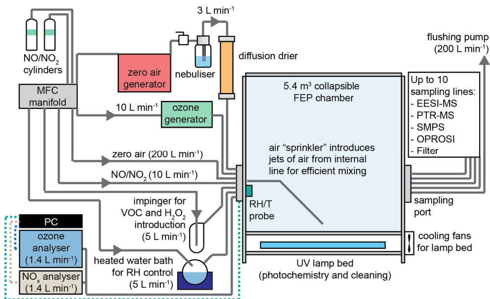
Figure 2: Schematic of the Cambridge Atmospheric Smog Chamber (CASC). The facility consists of a 5.4 m 3 collapsible FEP Teflon chamber with stainless steel ports at each end for introduction of gases and sampling of chamber air by a suite of instrumentation. Gas sampling lines are solid grey, data connections are dashed.
