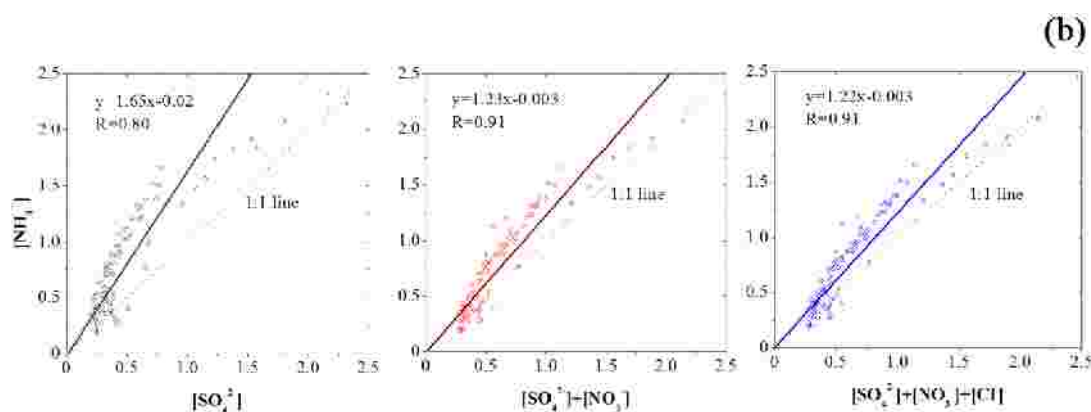
Figure 10. Correlations between [\text{NH}_4^+] and [\text{SO}_4^{2-}] (a), [\text{NH}_4^+] and [\text{SO}_4^{2-}] + [\text{NO}_3^-] (b) and [\text{NH}_4^+] and [\text{SO}_4^{2-}] + [\text{NO}_3^-] + [\text{Cl}^-] (c) during 7-11 August 2013.
