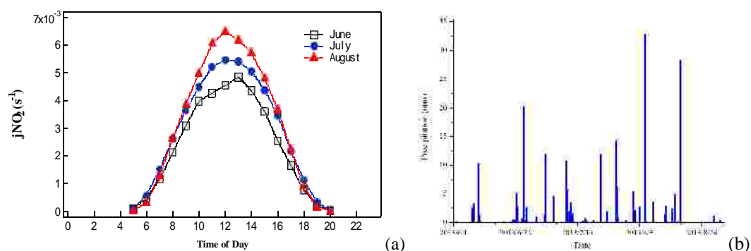
Figure S2. Monthly average diurnal variations of the \text{NO}_2 photolysis frequency ( j\text{NO}_2 ) (a) and hourly rainfall (b) observed at Gucheng during June-August 2013.
