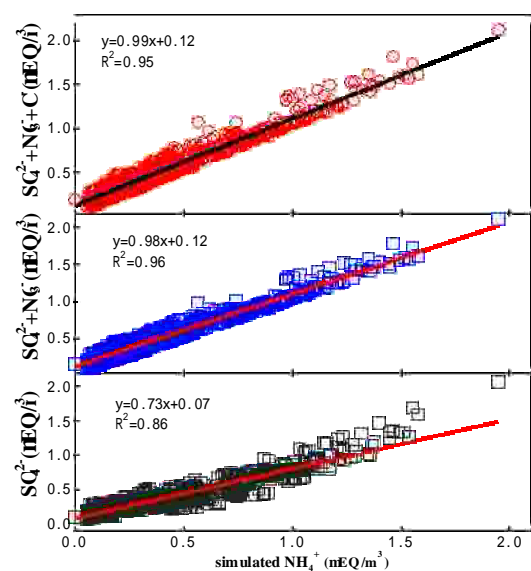
Figure S5 Correlation of modelled \text{NH}_4^+ with modelled \text{SO}_4^{2-} , \text{SO}_4^{2-} + \text{NO}_3^- and \text{SO}_4^{2-} + \text{NO}_3^- + \text{Cl}^- .
