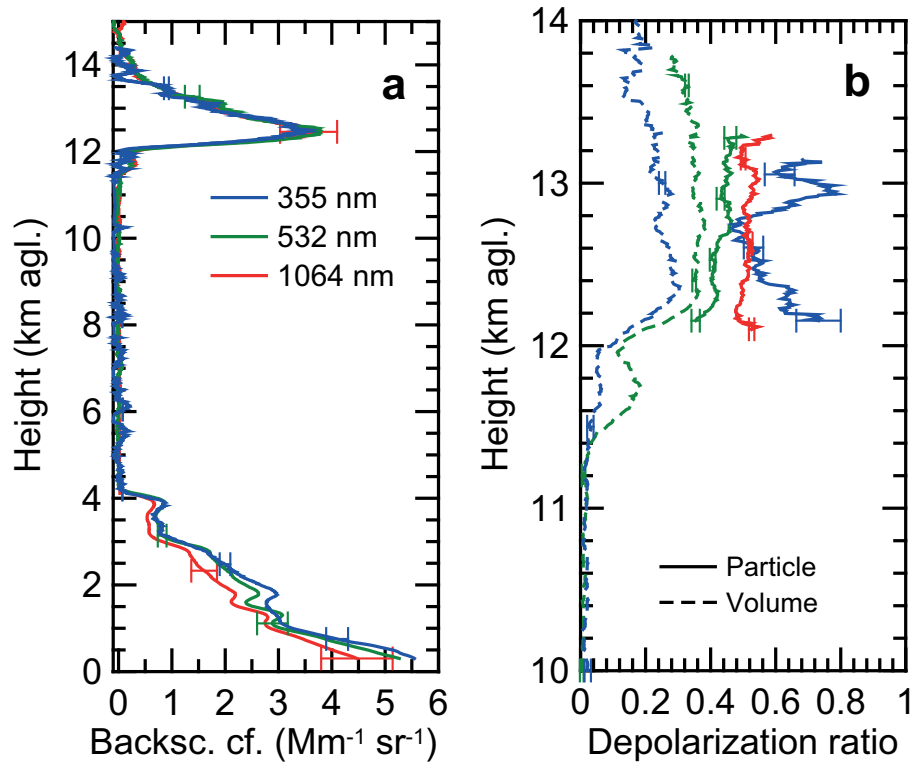
Figure 6. (a) Aerosol layers below 4 km height and cirrus layer from 12–14 km height in terms of particle backscatter coefficient at three wavelengths observed with lidar on 20–21 June 2014, 2310–0210 UTC (signal averaging period), and (b) cirrus ice crystal depolarization ratio (solid lines, volume depolarization ratio as dashed lines) at three wavelengths. At 1064 nm the volume depolarization ratio is equal to the particle depolarization ratio. The vertical signal smoothing length is 200 m. Error bars show the relative uncertainty in the retrievals (one standard deviation).
