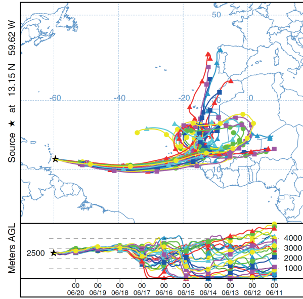
Figure 8. Ensemble of 10-day HYSPLIT backward trajectories for 21 June 2014, 00:00 UTC, arriving at at 2500 m over Barbados.
