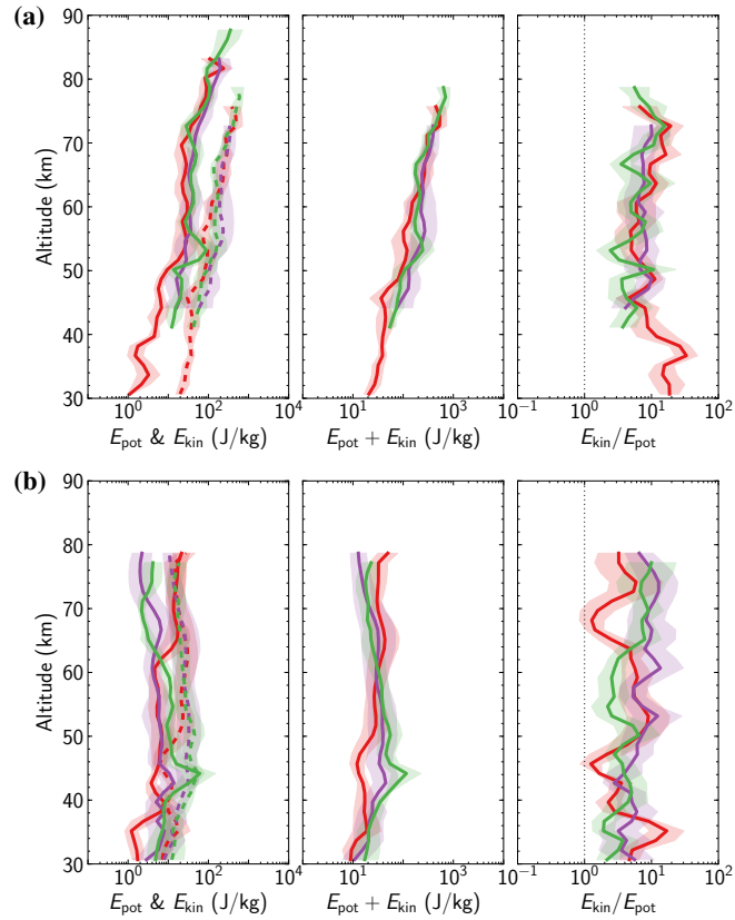
Figure 7. January mean gravity wave energy densities for 2012 (red), 2014 (purple), and 2015 (green) derived from lidar data (a) and ECMWF data (b). Shading represents the respective standard deviation. Left: potential (solid) and kinetic (dashed) GWED. Middle: total GWED. Right: kinetic-to-potential GWED.
