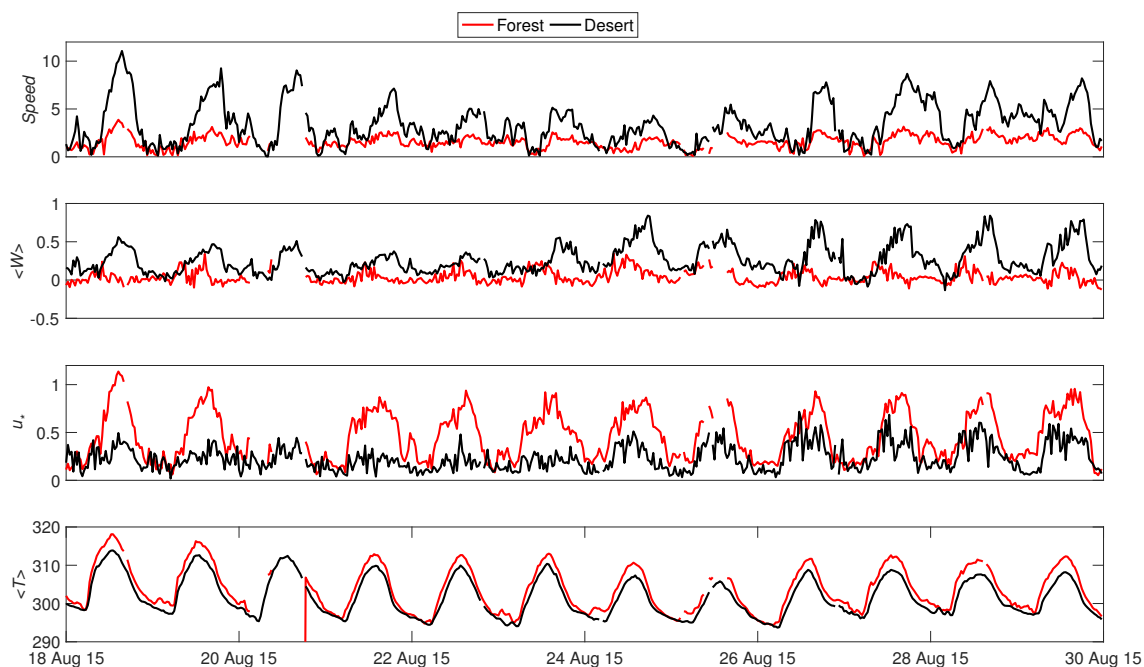
Figure 2. Time series of mean speed ( \text{ms}^{-1} ), mean vertical velocity ( \text{ms}^{-1} ), friction velocity ( \text{ms}^{-1} ) and mean potential temperature (K) for the measurement period. Black line indicates desert and red line indicates forest.
