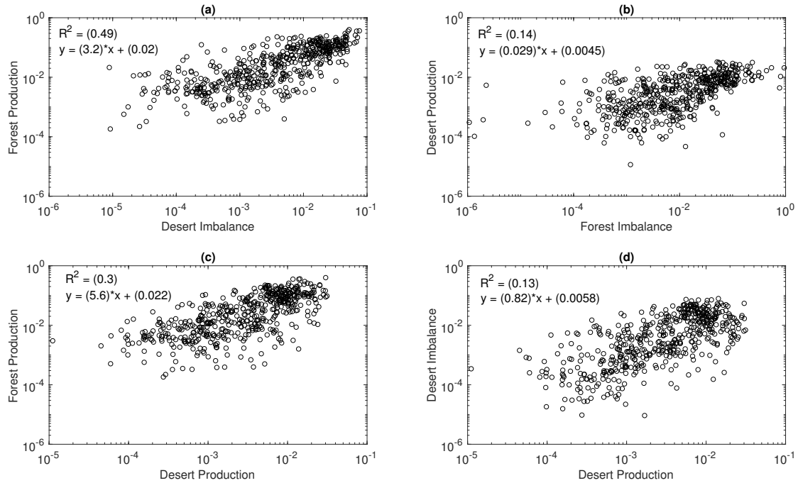
Figure 6. (a) TKE imbalance for desert vs TKE production for forest. (b) TKE imbalance for forest vs TKE production for desert. (c) TKE production for desert vs TKE production for forest. (d) TKE production for desert vs TKE imbalance for desert.
