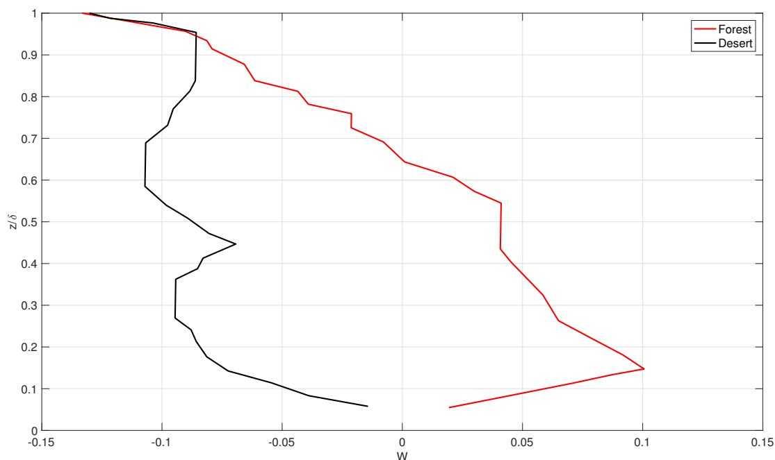
Figure 9. Mean vertical velocity \text{ms}^{-1} above the forest and the desert as measured by LiDARs.
