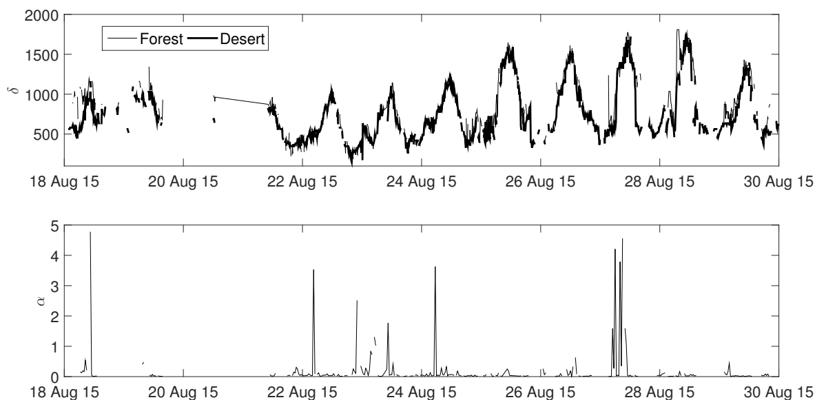
Figure 8. Top panel: Boundary layer heights ( \delta in m) measured using the Doppler LiDARs. Bottom panel: bulk measure of very large scale motion above the forest.
