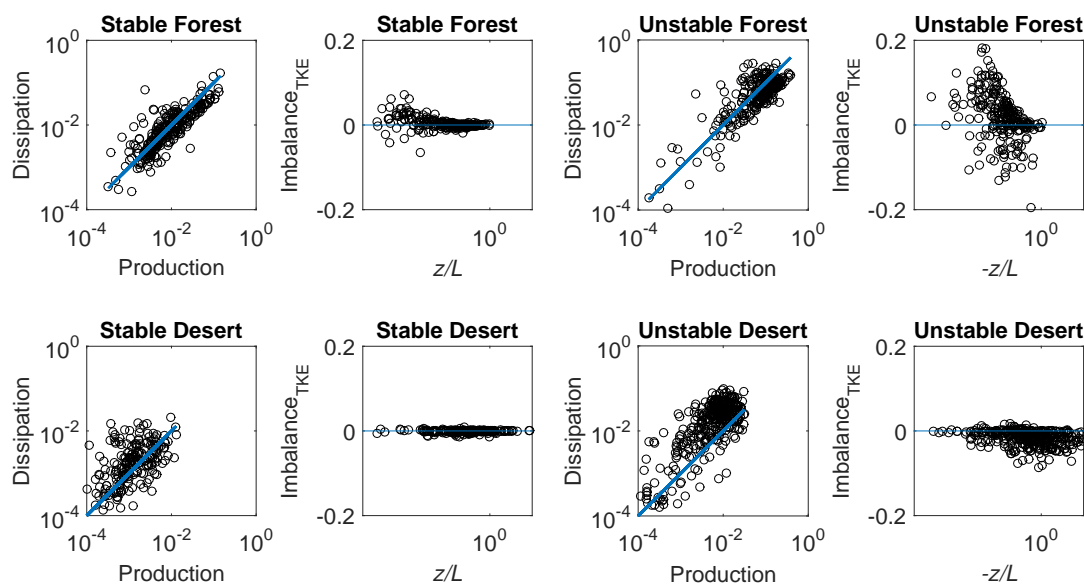
Figure 5. First row: forest, second row: desert. First column: TKE production vs dissipation for stable conditions. Second column: variation of TKE imbalance with stability parameter for stable conditions. Third column: TKE production vs dissipation for unstable conditions. Fourth column: variation of TKE imbalance with stability parameter for unstable conditions.
