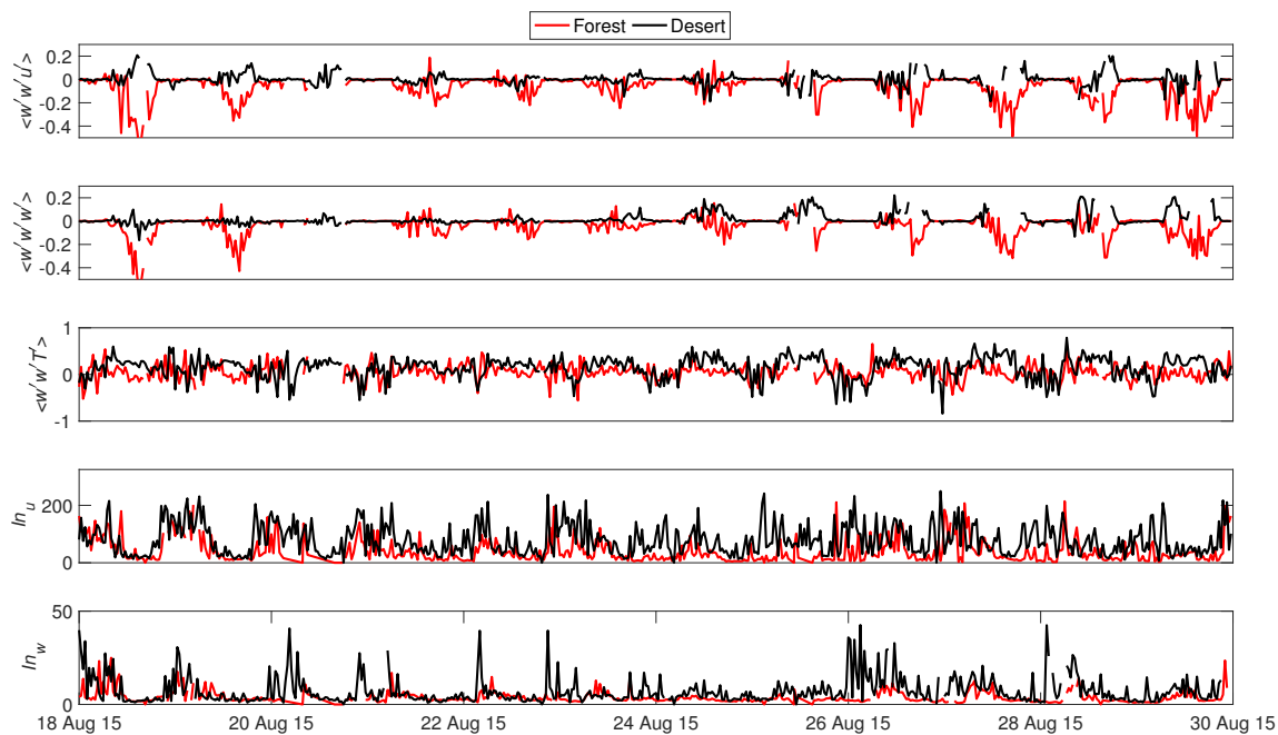
Figure 7. Top three panels: time series of triple moments \overline{w'w'u'} , \overline{w'w'w'} and \overline{w'w'T'} ( \text{m}^3\text{s}^{-3} ). Bottom two panels show the integral time scales of horizontal ( In_u ) and vertical velocities ( In_w ) in seconds.
