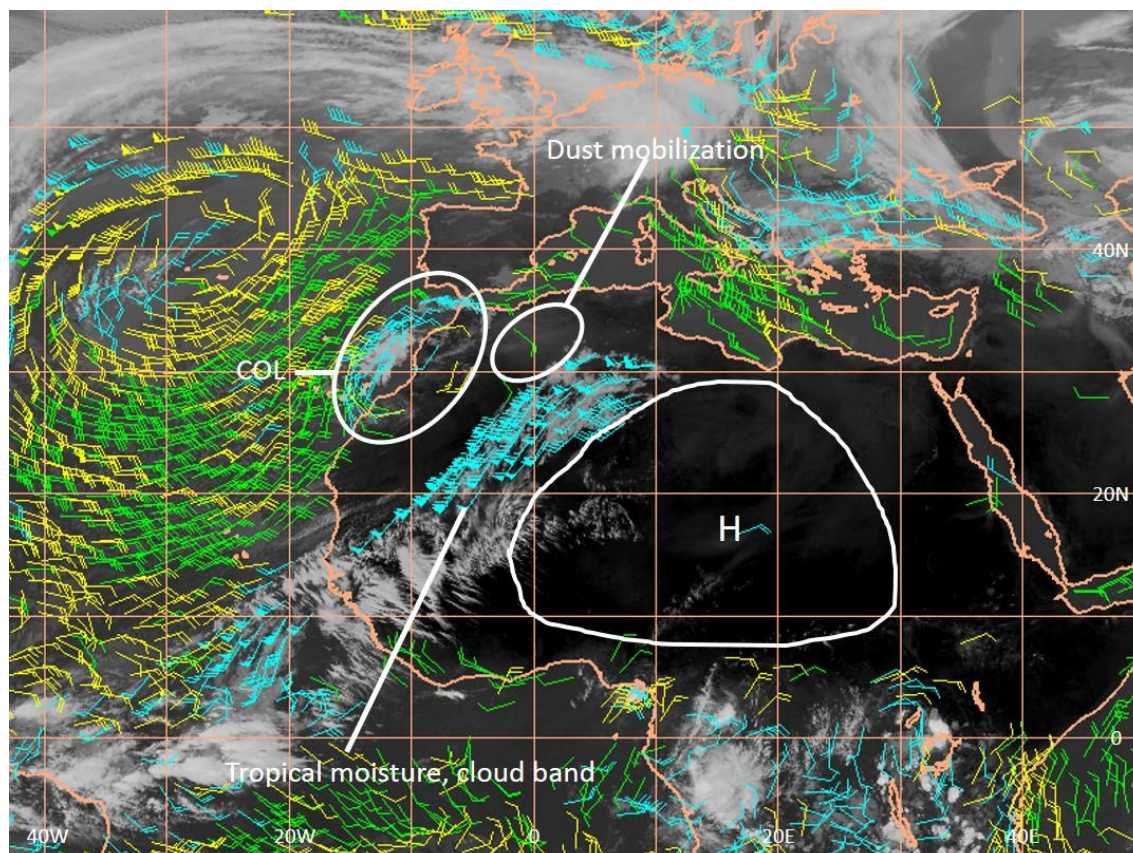
Figure 6. Relevant mid/upper -level features for the African dust outbreak: cut-off low (COL), upper-level anticyclone (H) and the tropical moisture intrusion on February 20, 12 UTC (image from University of Wisconsin-CIMSS).
