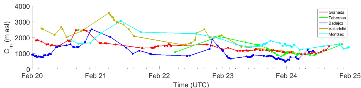
Figure 9. Time series of the integral of the particle backscatter coefficient for all stations (top panel) and time series of the center of mass of the backscatter profiles for all stations (bottom panel).
