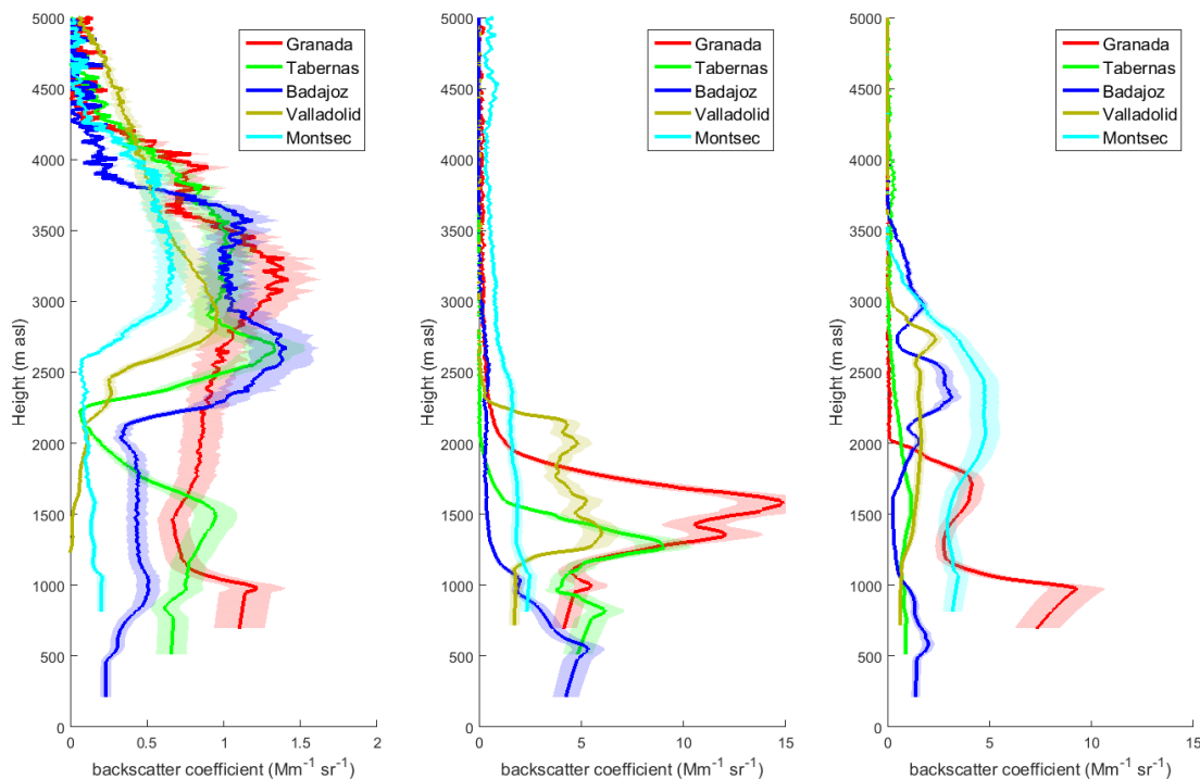
5 Figure 8. Particle backscatter coefficient profiles for all stations at the beginning (a), middle (b) and final stage (c) of the outbreak (note that x axis has different scale and the profiles start at ground level). Shaded area represents the 15% uncertainty.
