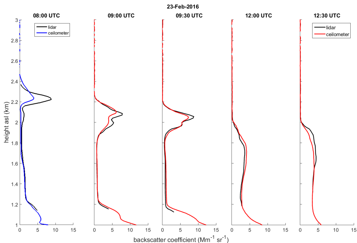
5 Figure 3. Lidar and ceilometer particle backscatter profiles for five cases on 23 February 2016. The first case (marked in blue) is a rejected ceilometer profile and the other four cases (marked in red), are cases with a ceilometer calibration factor within the 33% of the median calibration factor. Errors on lidar profiles have been estimated with a Montecarlo technique (Pappalardo et al., 2004; Mattis et al., 2016) and are in the order of 10^{-9} ( \text{m}^{-1} \text{sr}^{-1} ), therefore they are not shown.
