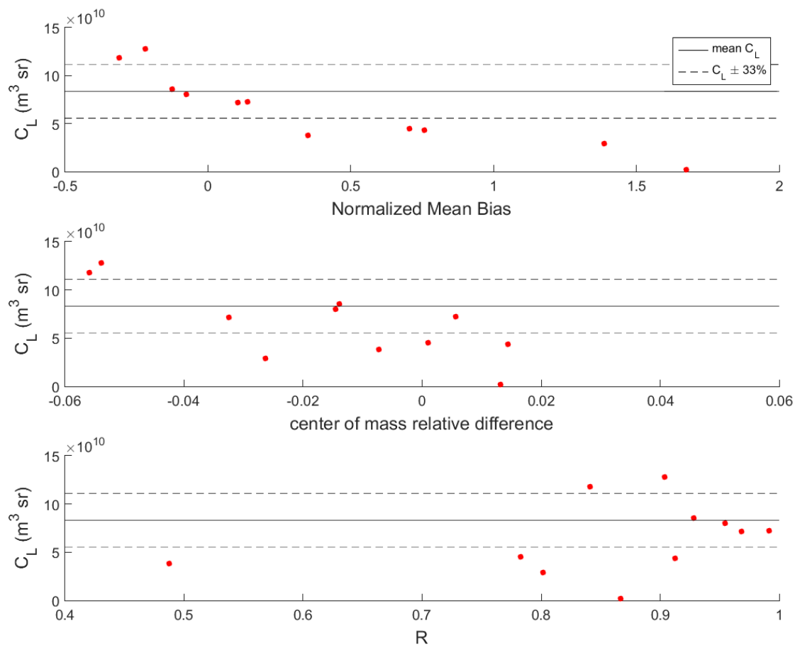
Figure 2. Ceilometer Calibration Factor ( C_L ) vs. normalized mean bias (NMB) on top panel, relative difference in center of mass on middle panel and coefficient of correlation ( R ) on bottom panel. Horizontal line indicates the mean C_L for the dust event period and dashed lines indicates the 33% around this mean value.
