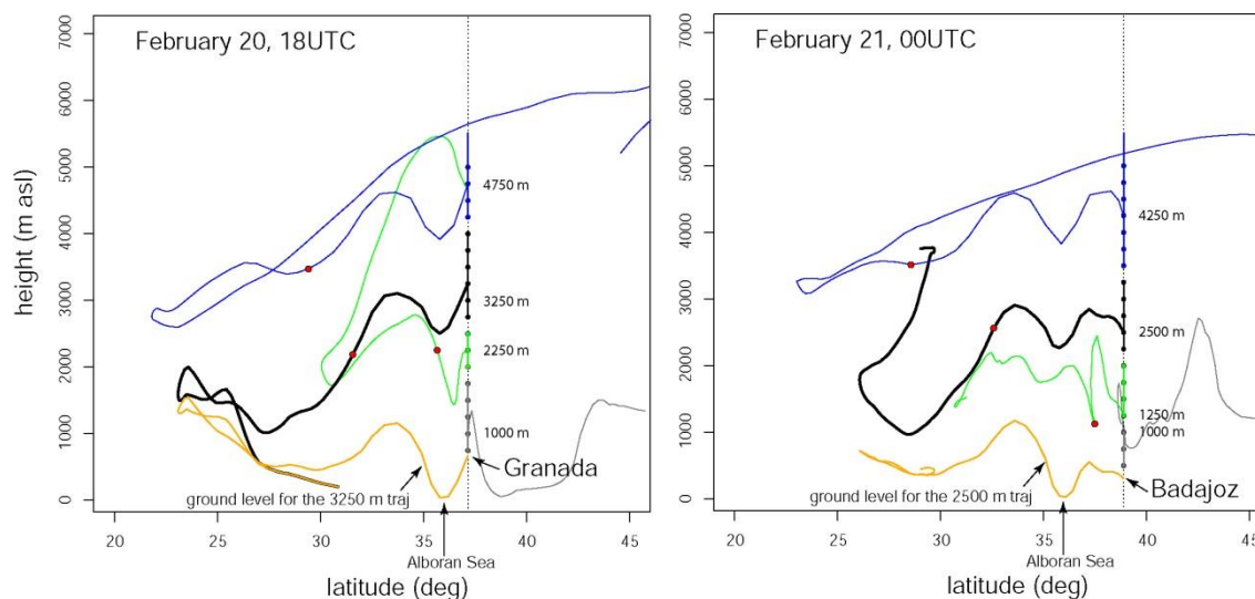
Figure 5. Evolution of the air parcels reaching Granada on February 20, 18:00 UTC (left) and Badajoz on February 21, 00:00 UTC (right) at different heights. Back-trajectories were calculated from the ground level to 5000 m asl, at every 250 m. Lines in grey indicate trajectories arriving at the lowest levels, with no African history; in green are trajectories that passed over the southern slope of the Saharan Atlas before the observed dust mobilization; in black are the trajectories followed by the parcels residing at the times and area where dust was observed; the trajectories residing at higher levels are depicted in blue. One representative trajectory is shown for each evolution and the altitude interval is shown in the same color as the representative trajectory. The brown line corresponds to the ground level for the trajectories more associated to the dust advection (thick black lines). The location of the air parcels around the time of observation of the dust plumes is shown as a red circle.
