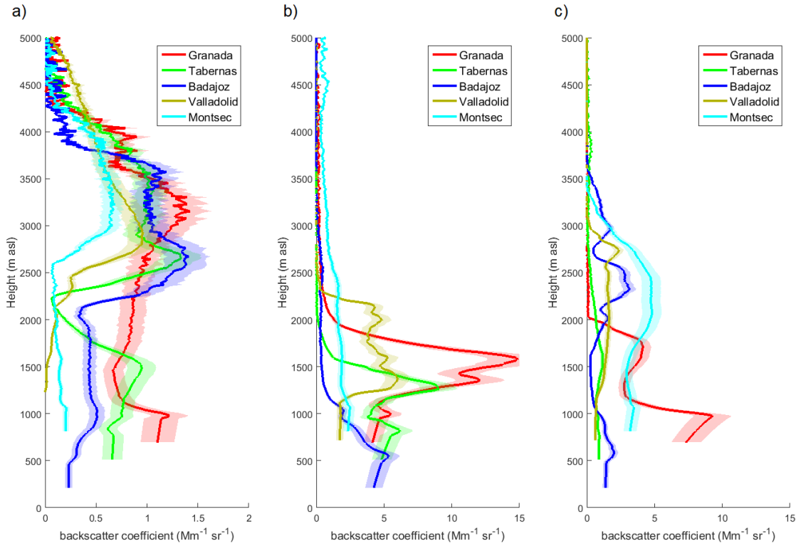
Figure 8. Particle backscatter coefficient profiles for all stations at the beginning (a), middle (b) and final stage (c) of the outbreak (note that x axis has different scale and the profiles start at ground level). Shaded area represents the 15% uncertainty.
