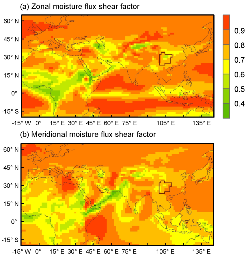
Fig. 1. Horizontal moisture flux shear factor in summer
