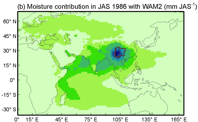
Fig. 2. Moisture contribution for JAS precipitation in 1986 SWC
