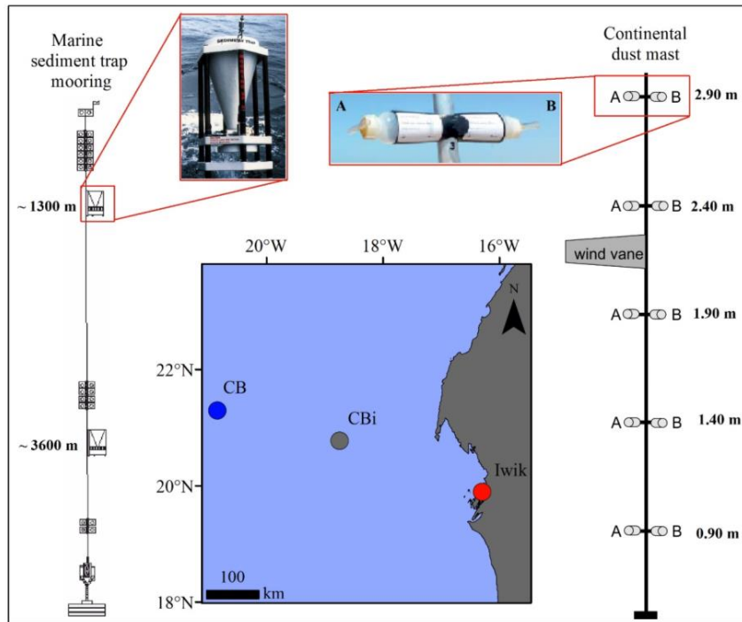
220 Figure 2: The marine sediment trap moorings CB and CBi offshore Cape Blanc and the dust masts near Iwik, 221 Mauritania. On the left, a sketch of the sediment trap mooring (sketch of CB 24 copied from Fischer et al. (2013)) 222 together with a photograph of the trap (downloaded from www.kum-kiel.de ) is displayed. On the right, a sketch of the 223 dust mast together with a photograph of the MWAC sampling bottles is depicted. 224
