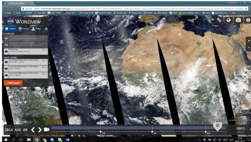
Figure A4: Dust storm on 08 August 2014.
