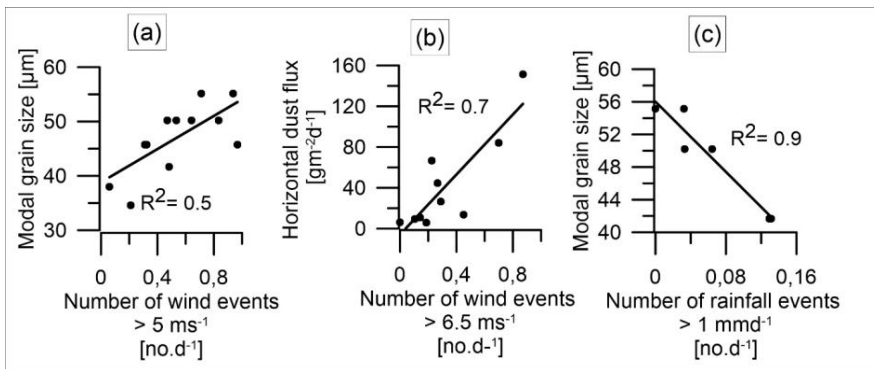
540 541 Figure 7: Correlation between the observed local surface wind speed at site Iwik and the measured (a) modal grain size 542 and (b) flux. (c) Correlation between the observed local precipitation at site Iwik (TRMM data) and the modal grain 543 size of the summer samples.
