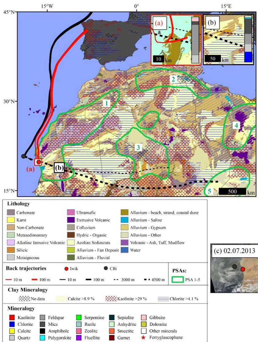
643 Figure 11: High- (4500 m) and low-level (10 m) four-day back trajectories of a dust event ending during the sampling 644 interval 24.06.-15.07.13 at site Iwik and during the sampling interval 25.06.-16.07.13 at site CBI. The potential source 645 areas and the mineralogy of the samples are given in the subfigures a-b. The dust storm event is indicated in subfigure 646 c.
