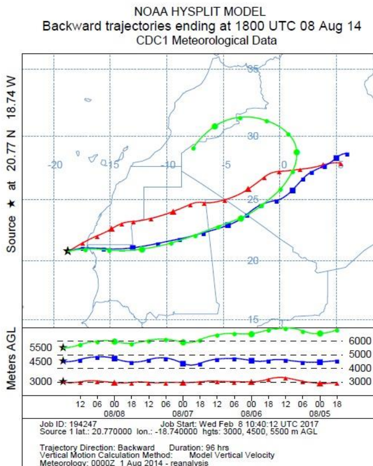
Figure A8: Four day back-trajectories at a height of 3000 m, 4500 m and 5500 m on 08 August 2014.
