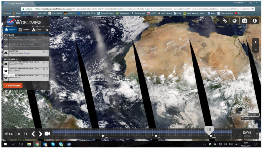
Figure A2: Dust storm on 31 July 2014.
