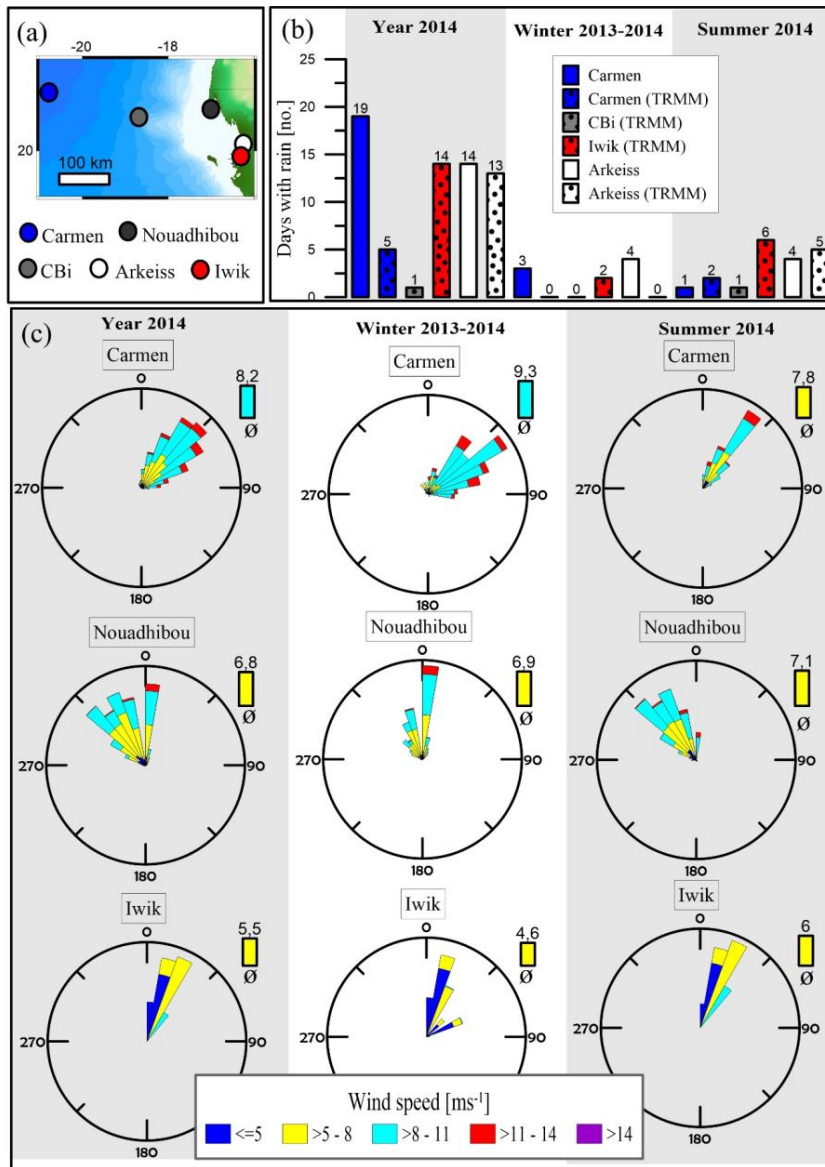
434 Figure 4: Meteorological data (a) map showing the study sites Carmen (CB), CBi, and Iwik, Nouadhibou and Arkeiss 435 the meteorological station in Nouadhibou (b) precipitation at the study sites Carmen (CB), CBi, 436 and Iwik and Arkeiss (c) wind direction and speed at the study sites Carmen (CB), Nouadhibou and Iwik, 437 and at the meteorological station in Nouadhibou.
