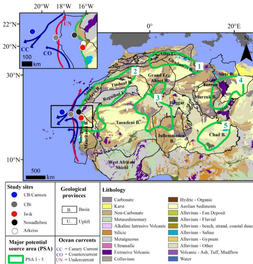
107 108 Figure 1: Map of the study sites under investigation: the scientific buoy Carmen as well as the sediment trap moorings 109 CB and CBi offshore Cape Blanc, the MWAC dust collector onshore near Iwik and the surface station near Nouadhibou 110 and Arkeiss. Location of the sediment trap moorings CB and CBi offshore Cape Blanc and the MWAC dust collector on 111 shore near Iwik (shapefile of the surface lithology and the geological provinces: downloaded from the USGS website 112 http://rmgsc.cr.usgs.gov/ecosystems/africa.shtml#SL and 113 http://certmapper.cr.usgs.gov/geoportal/catalog/main/home.page , major potential dust source areas: redrawn from 114 Scheuven et al. (2013), ocean currents: redrawn from Mittelstaedt (1991)).
