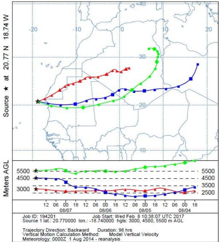
Figure A7: Four day back-trajectories at a height of 3000 m, 4500 m and 5500 m on 07 August 2014.
