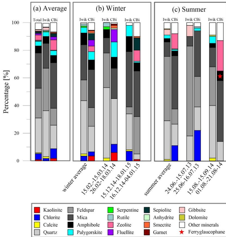
575 Figure 8: Mineralogical composition (a) averaged over all samples and for sites Iwik and CBI, (b) averaged for the 576 winter samples at sites Iwik and CBI and for each individual winter sample and (c) averaged for the summer samples 577 at sites Iwik and CBI and for each individual summer sample. The category ‘other minerals’ comprises the minerals 578 todorokite, sodalite, konicklite, gyanaitite, nitratine, urea, bernalite, akermanite, mixed-layer clay and talc.
