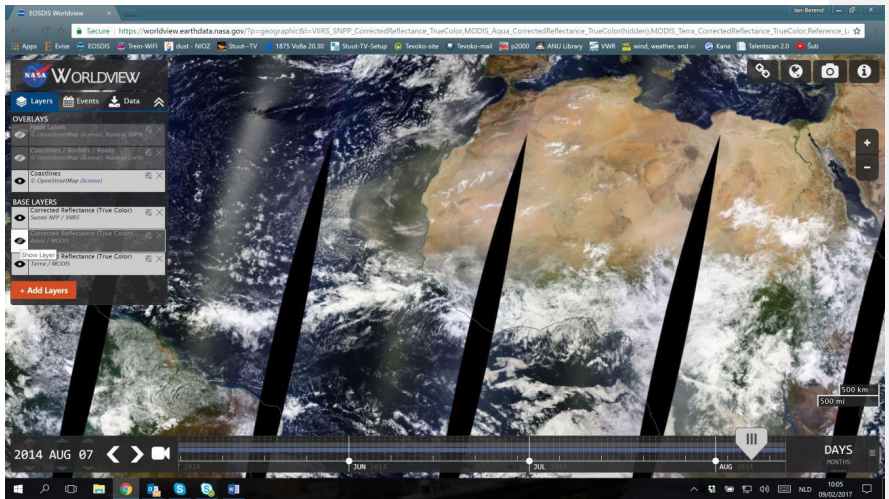
Figure A3: Dust storm on 07 August 2014.
