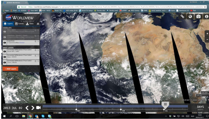
Figure A1: Dust storm on 02 July 2013.
