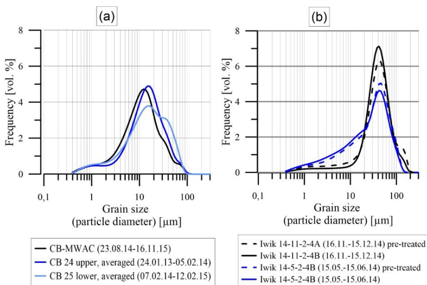
325 326 Figure 3: (a) Grain-size distributions for the station CB: Dust sampled with the MWAC sampler 2 m above sea level, 327 with the upper sediment trap at 1214 mbsl and the lower trap at 3622 mbsl. (b) Grain-size distributions of samples of 328 the Iwik 14 time series which have been pre-treated with HCl, H 2 O 2 and NaOH (dotted lines) and without pre- 329 treatment (lines).
