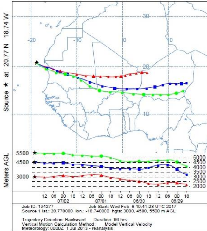
Figure A5: Four day back-trajectories at a height of 3000 m, 4500 m and 5500 m on 02 July 2013.
