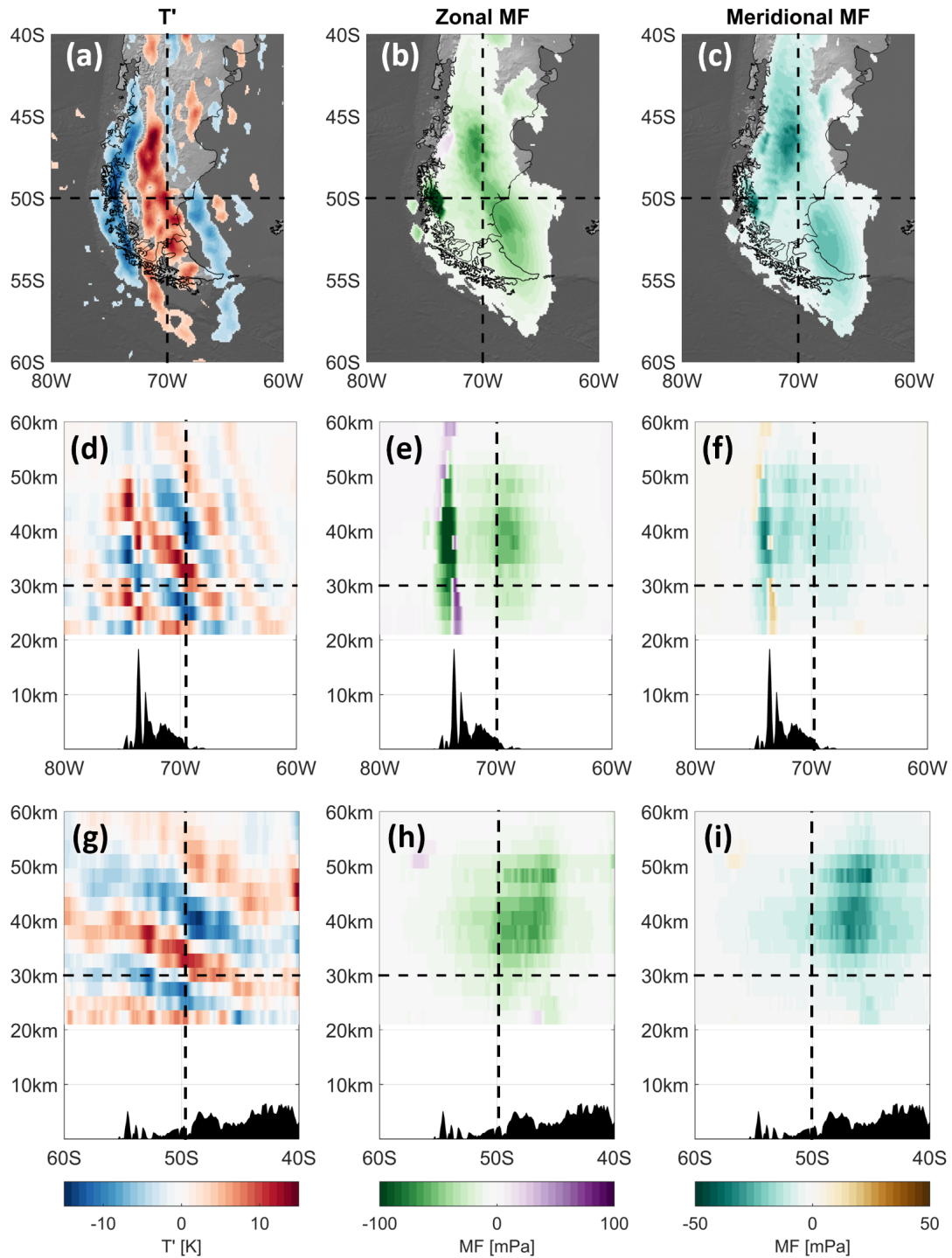
Figure 5. (a,d,g) T' , (b,e,h) zonal MF and (c,f,i) meridional MF associated with the waves shown in Fig. 2. (a-c) show maps at 30 km altitude. (d-f) show data at 50^\circ\text{S} , and (g-i) 70^\circ\text{W} , both against height. Black shading in panels (d-i) shows surface topography, scaled \times 5 for clarity. As in previous figures, the exponential increase in wave amplitude with altitude has been removed in (a,d,g) in order to highlight the vertical structure.
