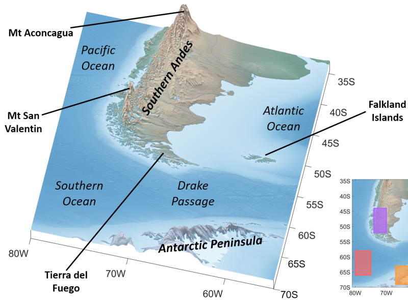
Figure 1. [main panel] Map of region examined in this study, defining geographic terms used. [inset] Subregions examined in Sect. 6: ‘Andes’ (purple), ‘Peninsula’ (orange), and ‘Southern Ocean’ (red).
