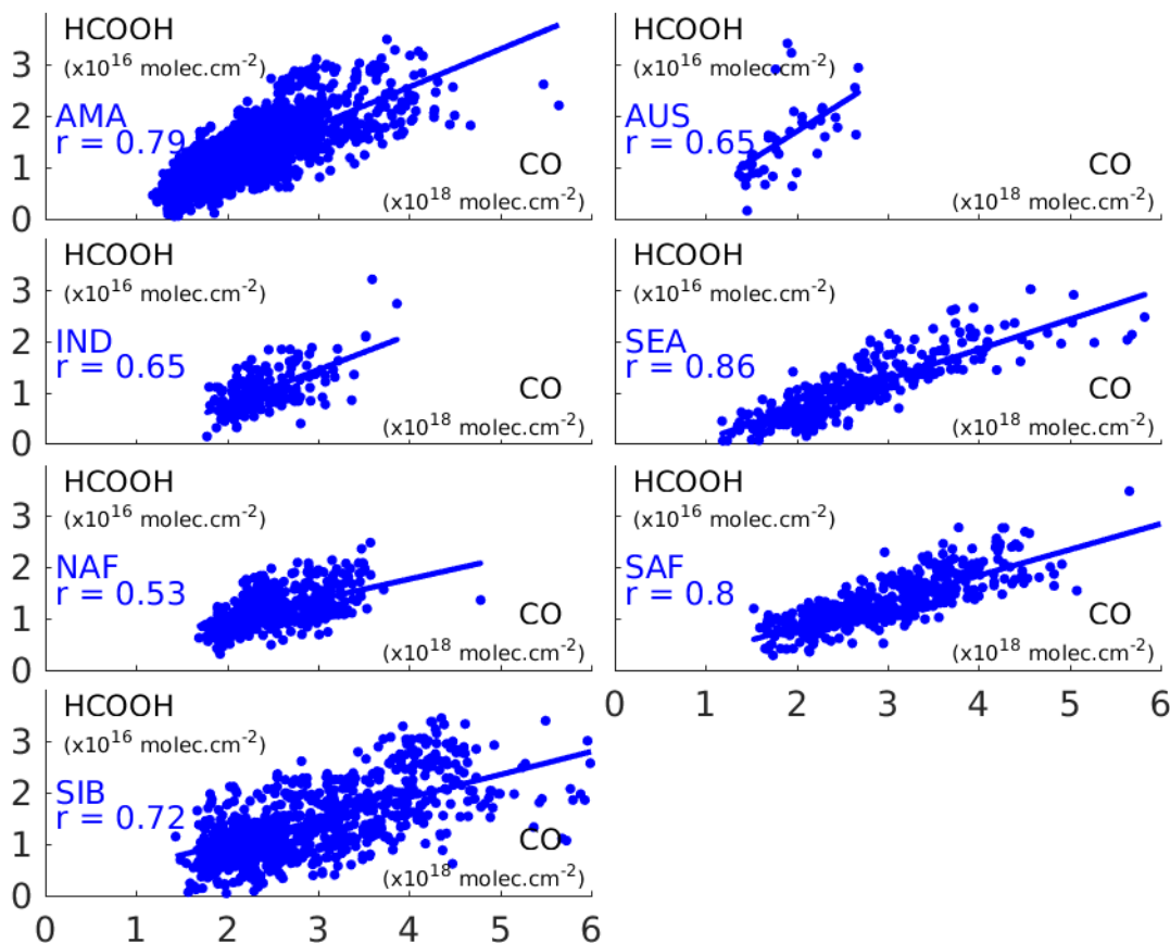
800 Figure 4: Scatterplots between the IASI fire-affected HCOOH total columns (in 10^{16} molec./ cm^2 ) and the CO total columns (in 10^{18} molec./ cm^2 ) over the seven regions (AMA=Amazonia, AUS=Australia, IND = India, SEA = Southern East Asia, NAF= Northern Africa, SAF= Southern Africa, SIB= Siberia). The linear regression is represented by the blue line and the correlation coefficient is also provided for each region.
