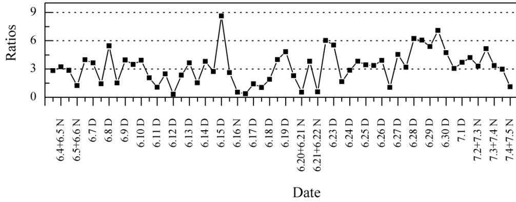
Fig. 10. Time series of the Ph/C 9 ratios (D: day, N: night).
