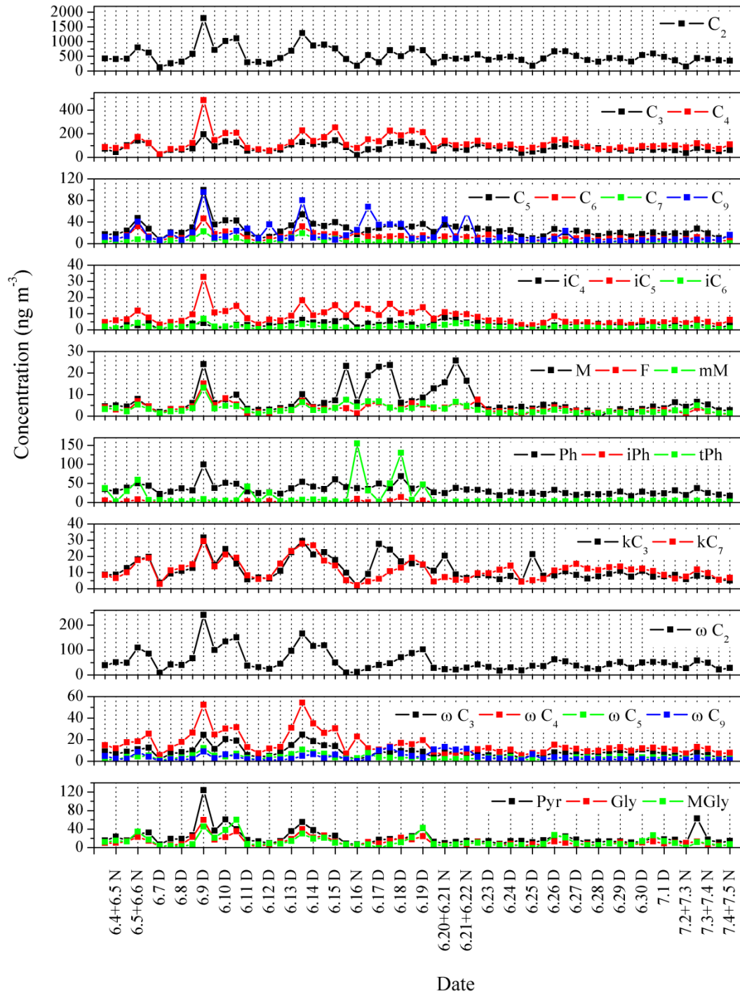
Fig. S3. Temporal variations of selected species in PM 2.5 aerosol collected at Mt. Tai on the day (D) and night (N) in 2014.
