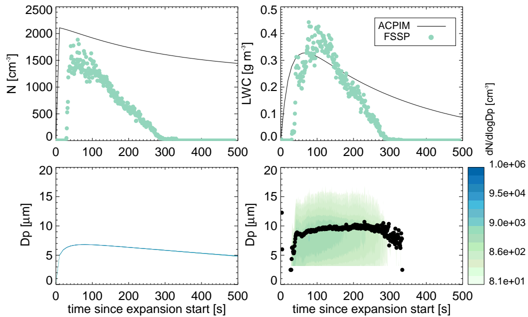
Figure 8. Comparison of ammonium sulfate measurements ( Exp. 9, run2, see Table 1 and ACPI simulation of number concentrations (upper left), LWC (upper right), size distribution and mean volume diameter (lower panels, measured right, simulated left).
